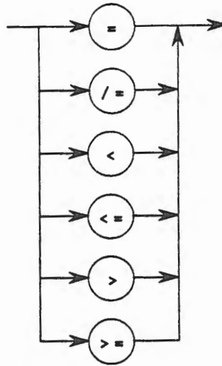
Object Declaration Syntax Chart 2.10
