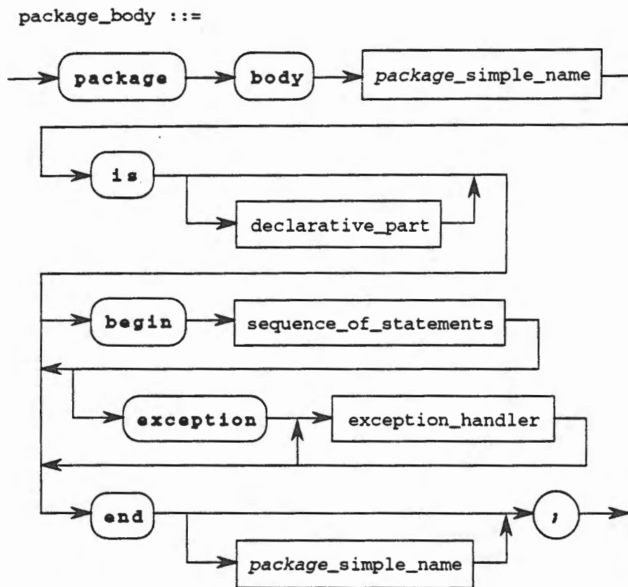
Ada Package Body Syntax Chart 8.2
