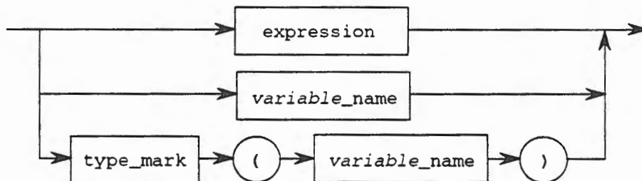
Ada Expressions Syntax Chart 2.12
