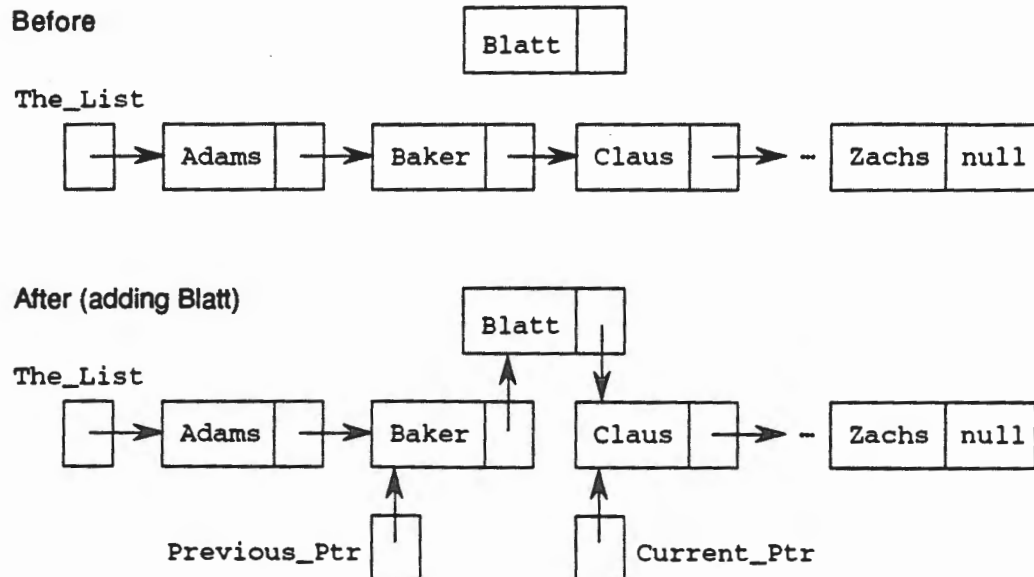
Inserting in the Middle of List Figure 9.25
