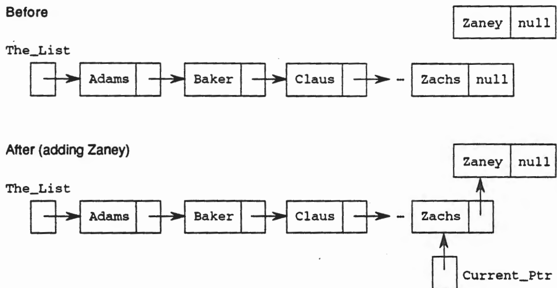
Inserting at the End of List Figure 9.26
