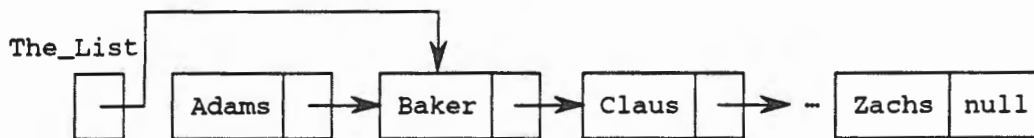
Deleting from the Beginning of List Figure 9.27
