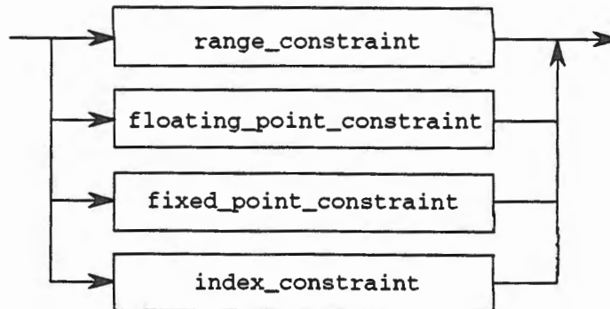
Record Type Declaration Syntax Chart 11.3
