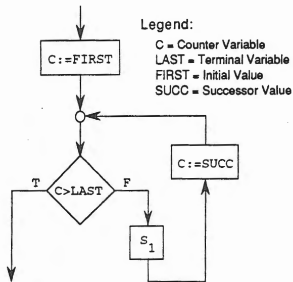
For Loop Flowchart Figure 2.9
