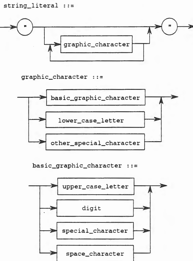
String Literal Syntax Chart 2.4
