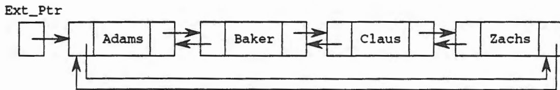
Circular Doubly Linked List Figure 9.22
