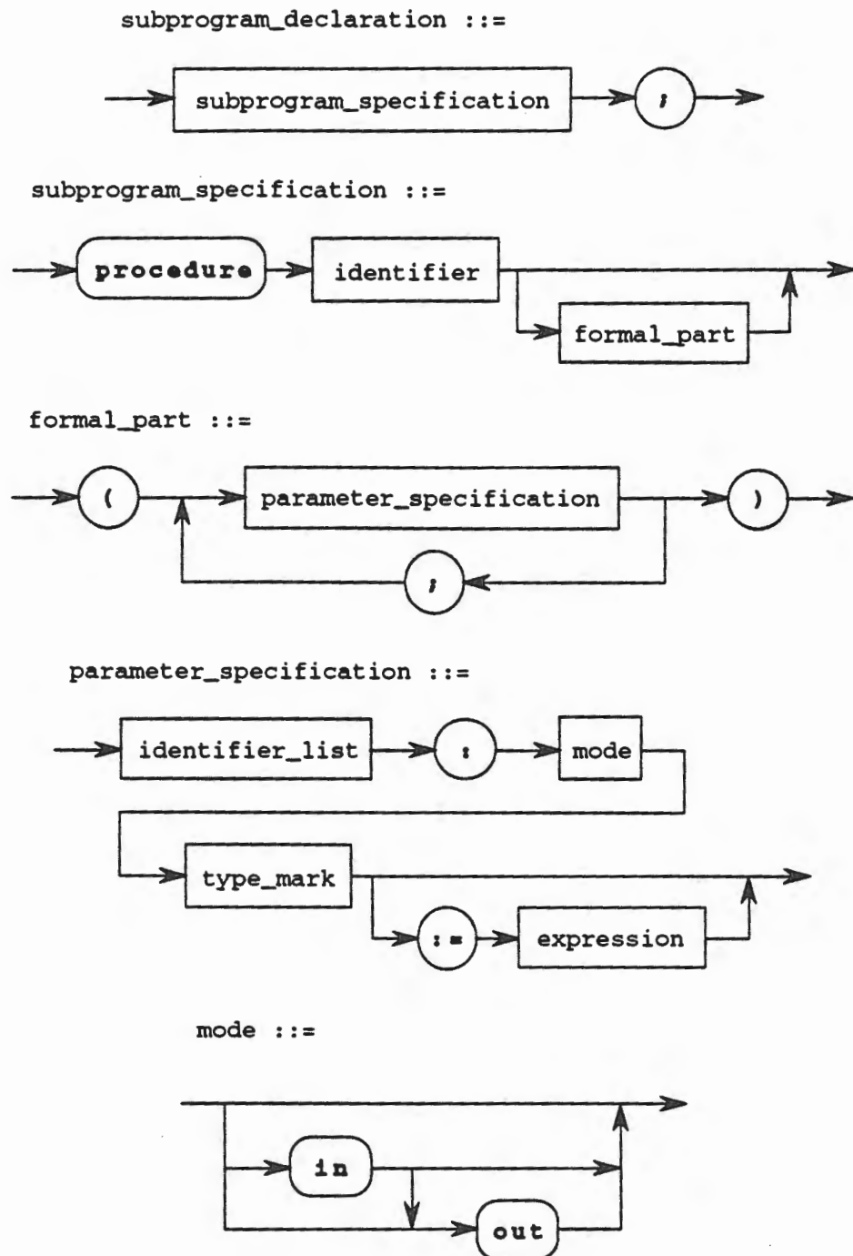
Procedure Specification Syntax Chart 8.3
