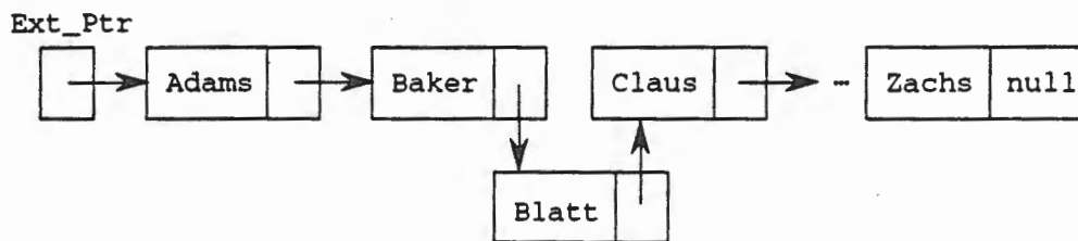
Node Insertion Figure 9.14
