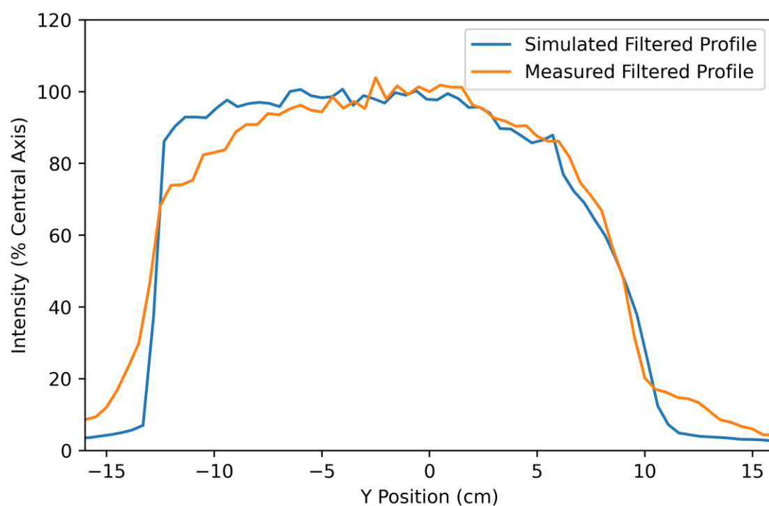
Figure 32. Simulated beam heel plotted versus the measured profile in the Y direction, parallel with the electron beam within the X-ray tube with the multilayer filter.
