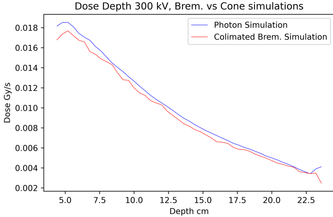
Figure 8. Dose rate versus depth curves as a function of depth into the body in cm for the X-ray cone simulation (Blue) and the full electron/target/X-ray simulation (Red). The slight variation with the collimated bremsstrahlung spectrum can be attributed to poor convergence, and some failed statistical checks even after long simulation times.
