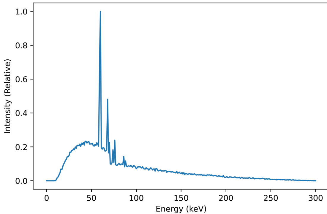
Figure 38. Unfiltered 300 kVp X-ray spectrum with an average X-ray energy of 83 keV. The spikes between 50 and 80 keV are due to K and L shell X-rays from the tungsten target.
