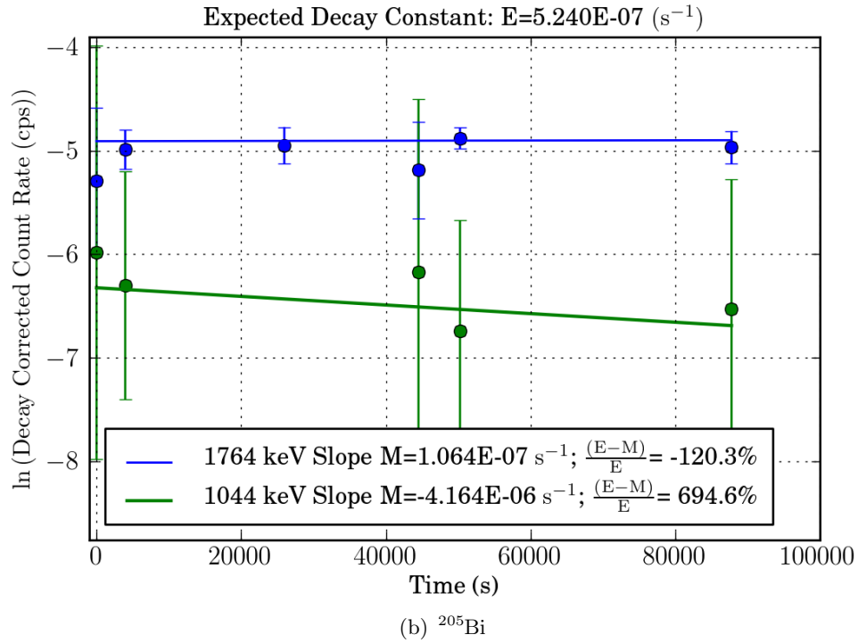
Figure 5.9: Time analysis measuring the decay constant for the ^{204}\text{Bi} and ^{205}\text{Bi} candidate peaks.
