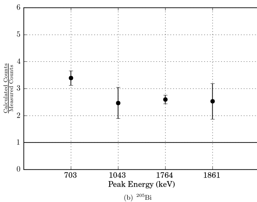
Figure 5.15: The ratio of calculated counts to measured counts for the ^{204}\text{Bi} and ^{205}\text{Bi} candidate peaks.
