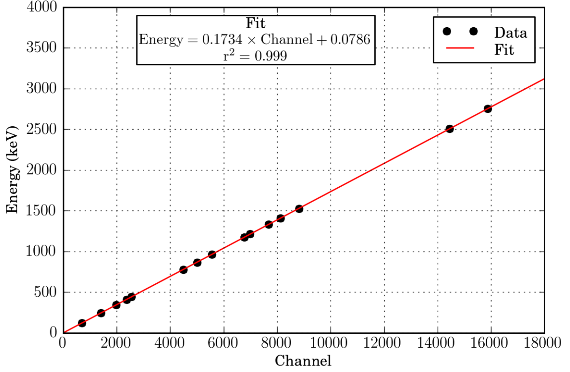
Figure 5.5: Energy calibration curve for the HPGe spectrometer used for the ARCS foil irradiation.
