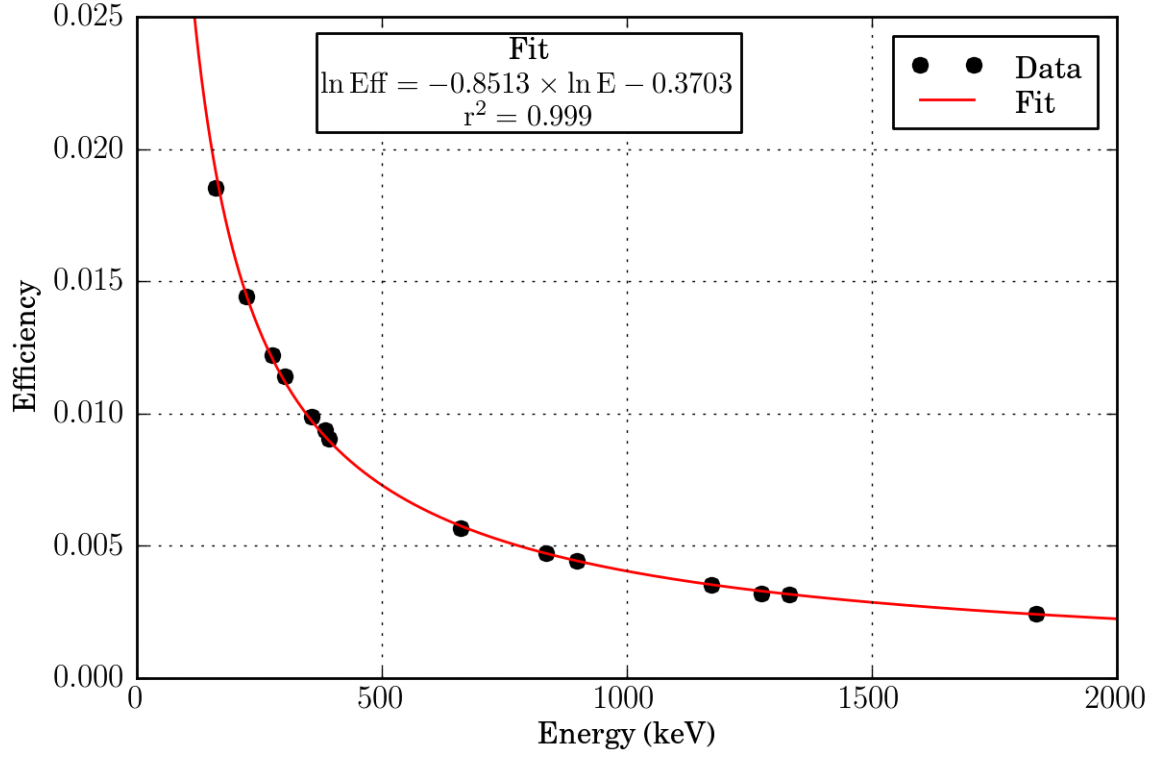
Figure 5.24: Efficiency calibration curve for the HPGe spectrometer used for the POWGEN foil irradiation.
