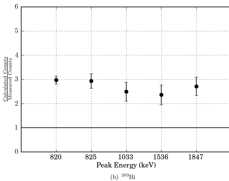
Figure 5.14: The ratio of calculated counts to measured counts for the ^{202}\text{Bi} and ^{203}\text{Bi} candidate peaks.
