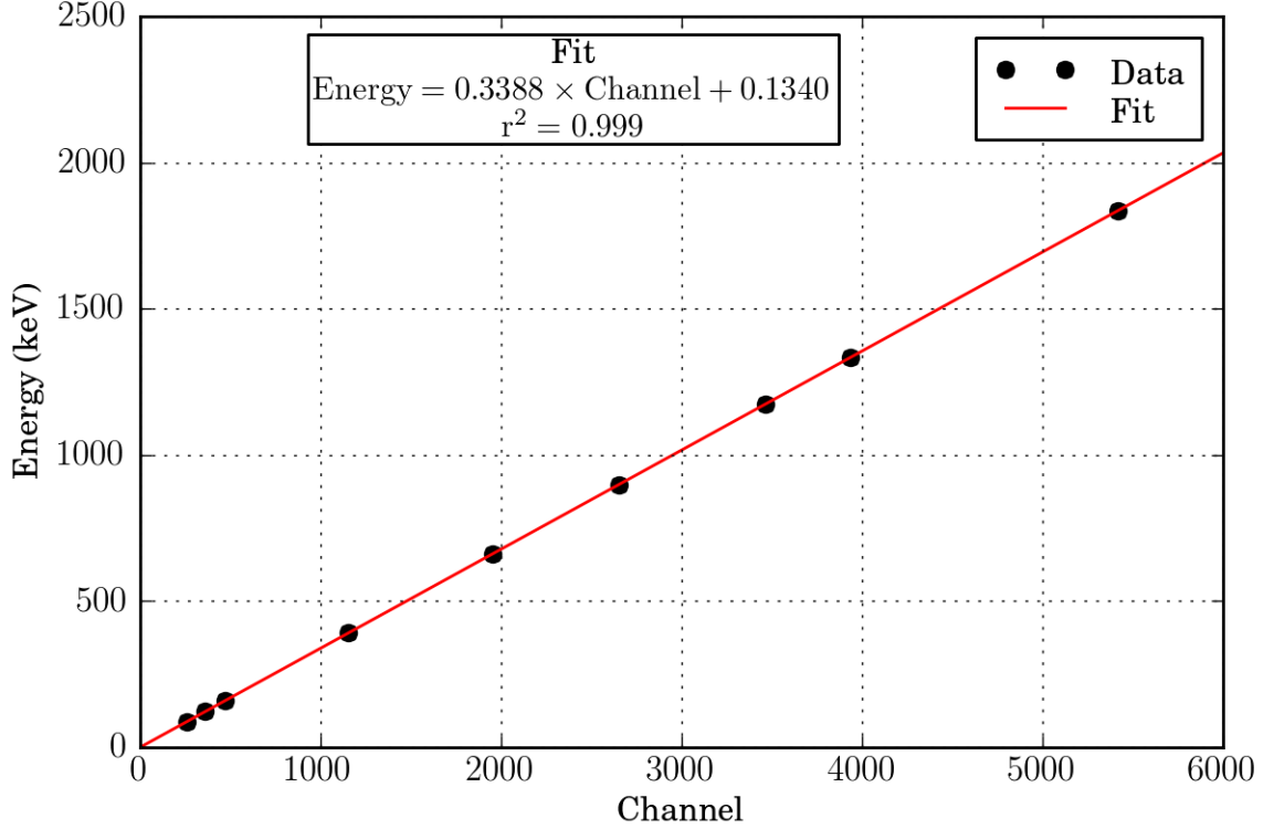
Figure 5.23: Energy calibration curve for the HPGe spectrometer used for the POWGEN foil irradiation.
