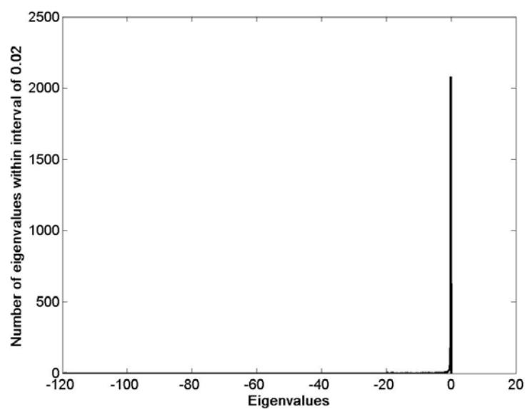
Figure 5.8 Eigenvalue distribution of matrix in Fig. 5.7.
