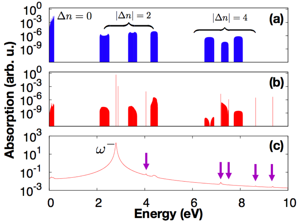
Figure 3.4: The absorption spectra (a) without and (b) with e-h pairs interactions, for a thin film of thickness 4d_m and k = 0.012 \text{ a.u.} . (c) is the result of (b) broadened by a Lorentzian with full width at half maximum \gamma = 0.04 \text{ eV} .
