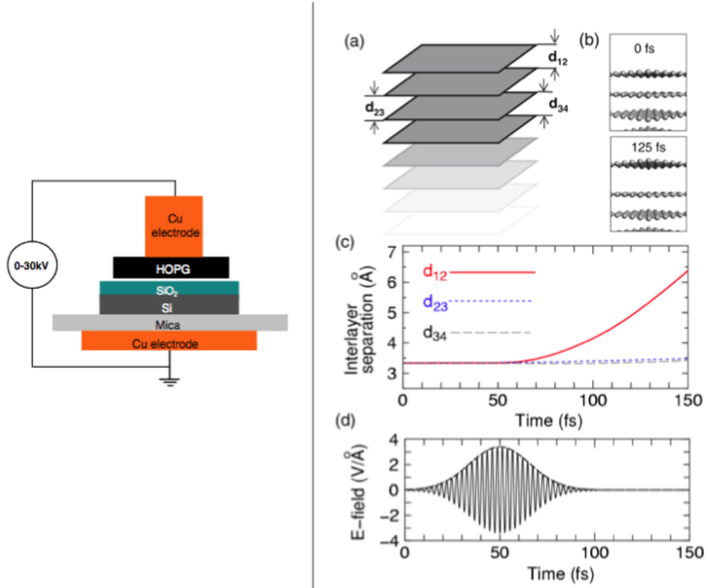
Figure 6.1: Left [152]: schematic of the experimental set-up for electrostatic deposition of graphene sheets, where HOPG stands for highly oriented pyrolytic graphite. Right [153]: schematic layer stacking (a) and structural snapshots (b) of the surface of AB-stacked graphite during exposure to a laser pulse with the full width at half maximum of 45 fs and a wavelength \lambda = 800 nm. (c) Time evolution of the interlayer distances. (d) Time-dependence of the optical electric field E characterizing the laser pulse.
