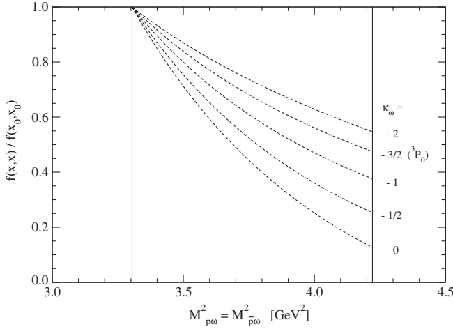
FIG. 5. Theoretical J/\psi \rightarrow p\bar{p}\omega DP event density along the diagonal M_{p\omega}^2 = M_{\bar{p}\omega}^2 , showing the strong \kappa_\omega dependence.
