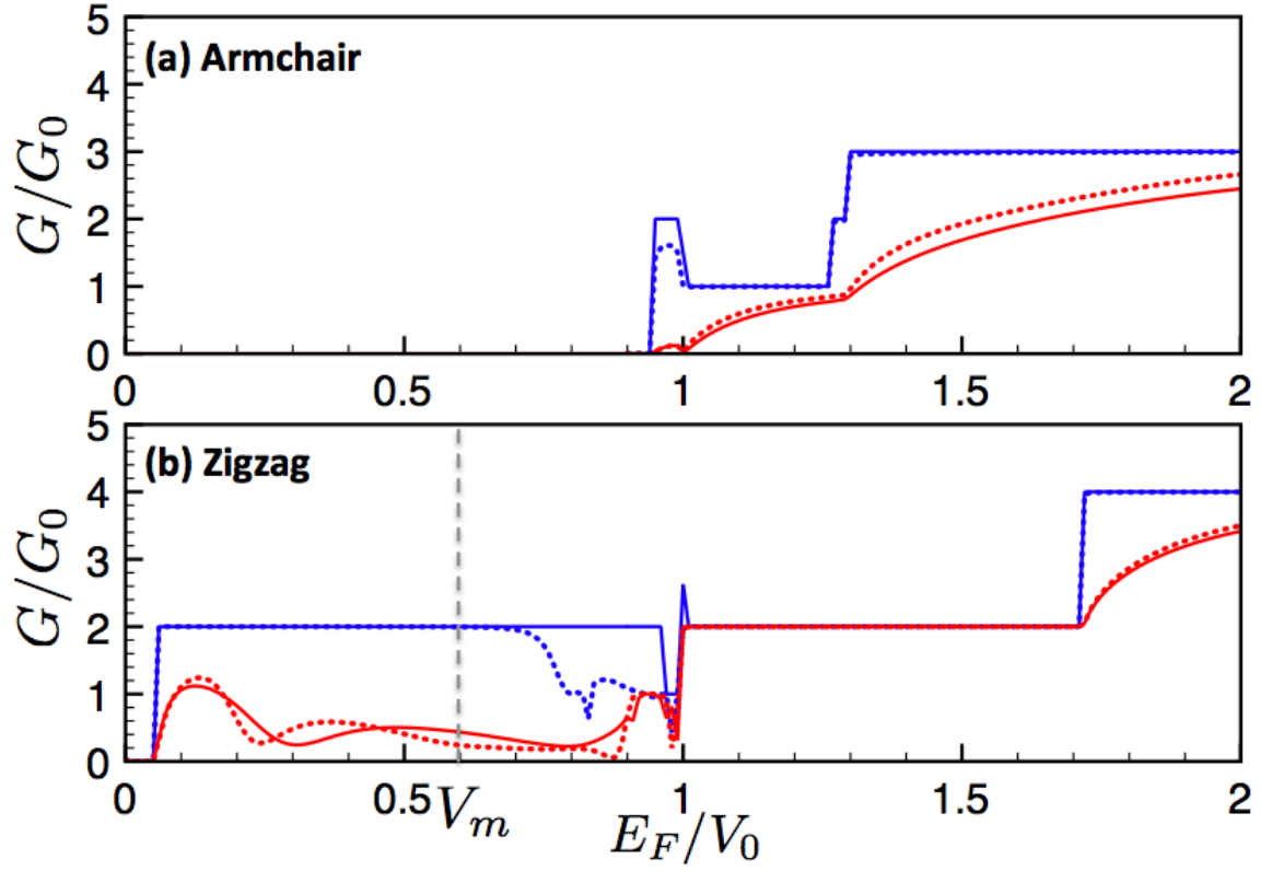
Figure 5.8: Conductance of (a) armchair ( N = 80 w_a ) and (b) zigzag ( M = 80 w_z ) nanoribbons. The solid lines refer to the ideal abrupt potential change on the interface. The dashed lines refer to the smooth potential change with interface length of D = 5 and V_m = 0.6V_0 for parallel configuration. Red (blue) lines refer to parallel (anti-parallel) configuration.
