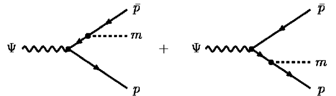
FIG. 1. Feynman diagrams of the meson emission model.
