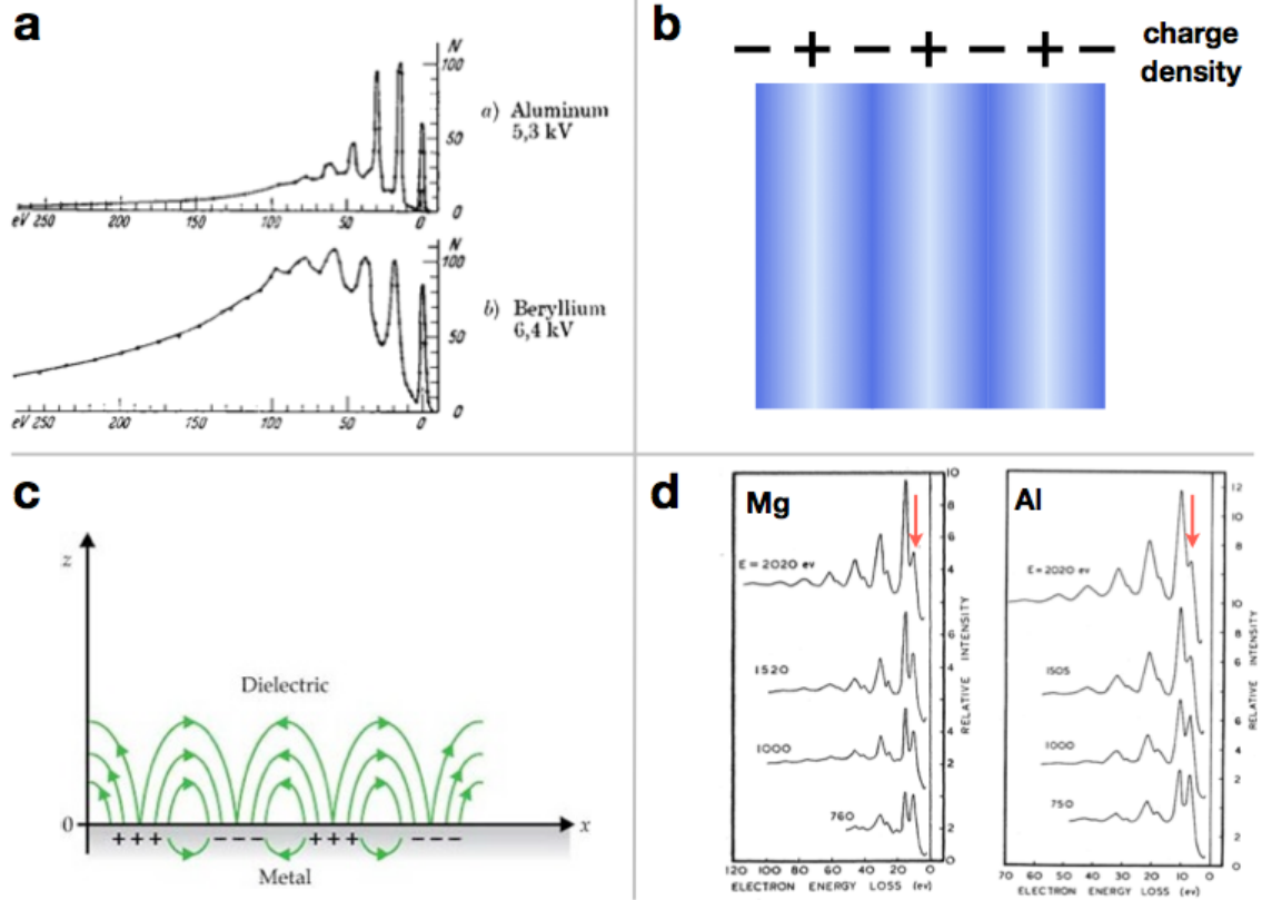
Figure 1.2: (a) Bulk plasmons of Al and Be measured by electron energy loss spectroscopy (EELS) [1]. (b) Charge density oscillations of bulk plasmons. (c) Charge density oscillations and induced electric fields of surface plasmons. (d) Surface and bulk plasmons of Mg and Al measured by EELS (Small shoulders aside huge the bulk plasmon peaks marked by the red arrows are due to the surface plasmon absorptions.) [2, 3].
