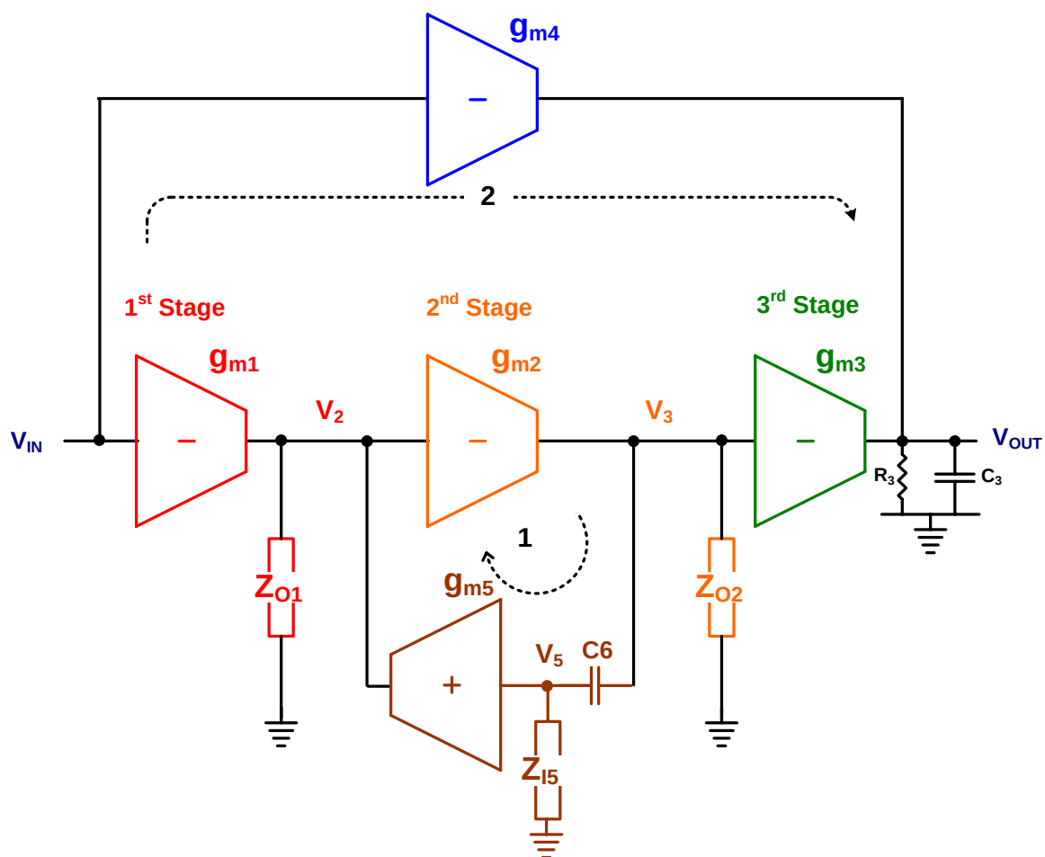
Figure 3.8. Block level schematic of the complete frequency compensated single-ended, half-circuit of the CT-amplifier
