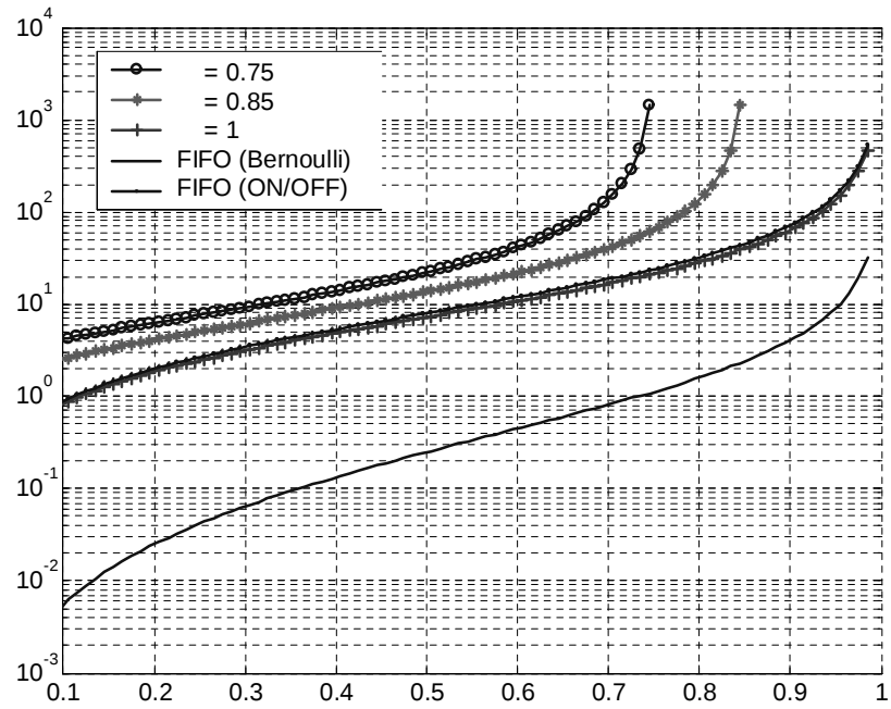
Figure 2-4: Mean queueing latency as a function of the offered load for random and FIFO arbitration schemes.
