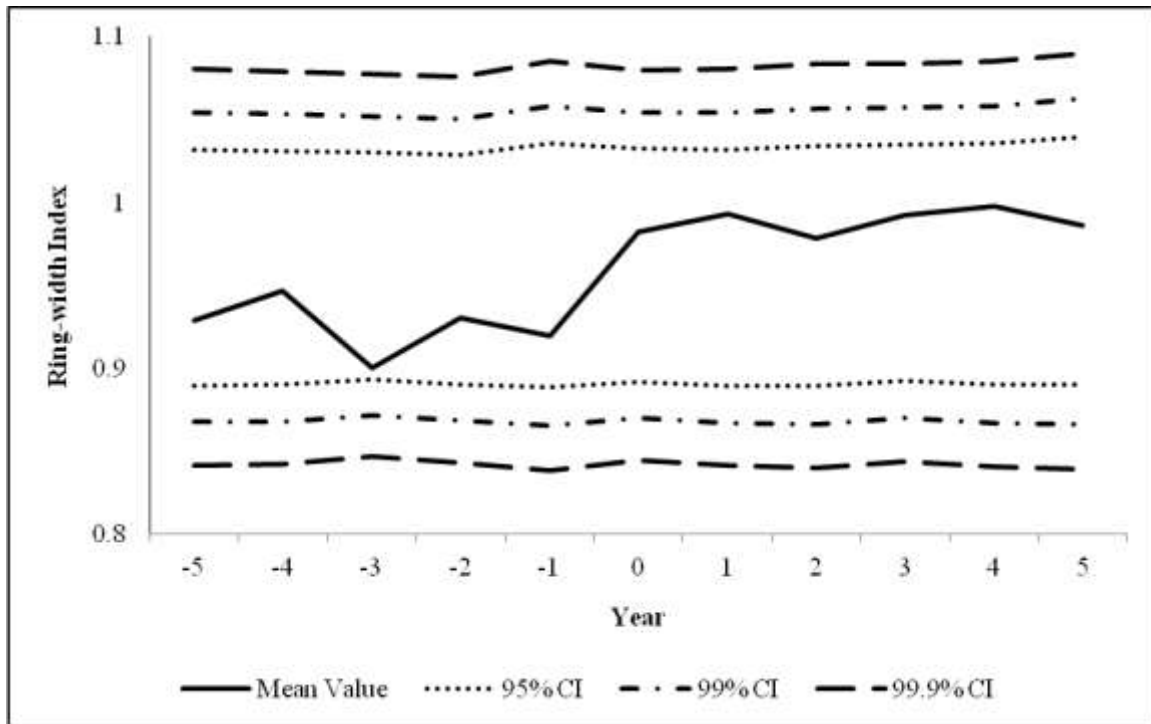
Figure 5.7 Results from superposed epoch analysis showing the relationship between climate, tree growth, and regional fire events for the combined fire chronology.
