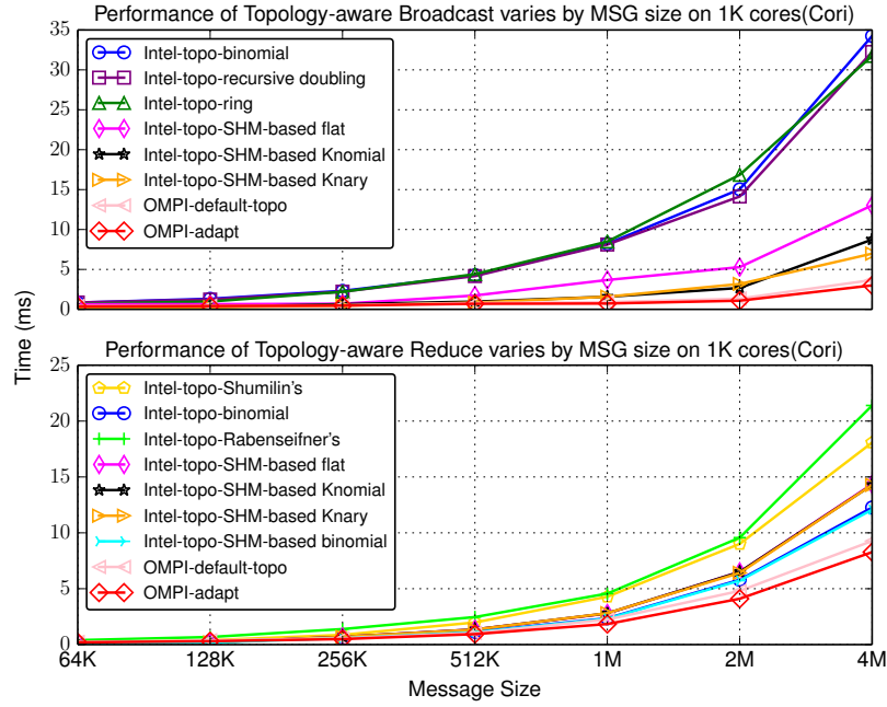
Figure 4.6: Performance of topology-aware MPI_Bcast and MPI_Reduce (1K cores, Cori)
