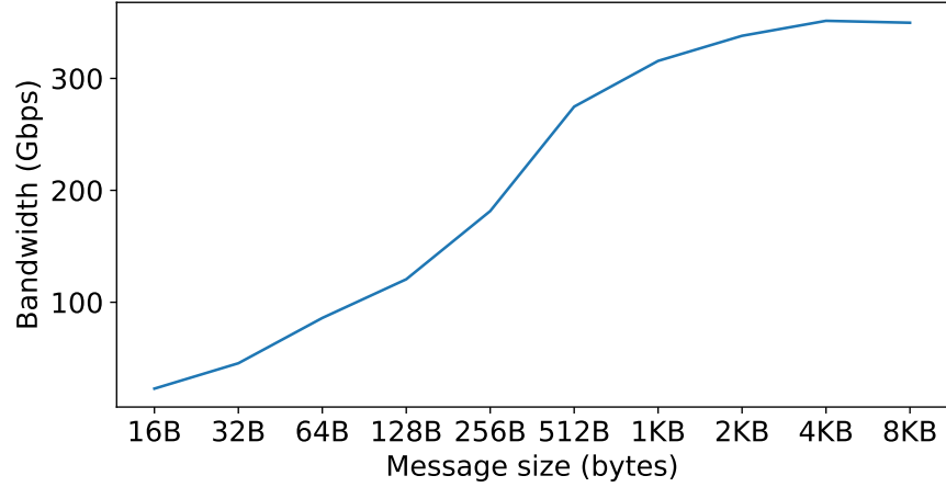
Figure 5.5: Malloc bandwidth on Saturn
