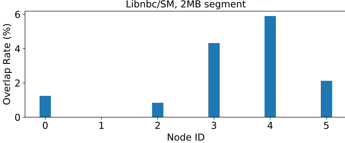
Figure 5.10: Overlap Rate of Concurrent Intra-node and Inter-node Collective Operations (6 nodes, 12 ppn, SM module)
