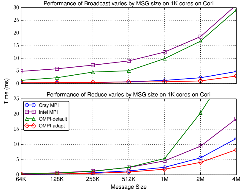
Figure 4.8: Performance of MPI_Bcast and MPI_Reduce varies by message size (1K cores, Cori)
