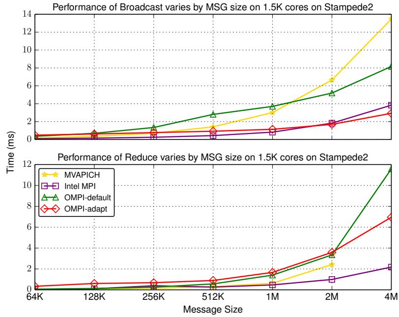
Figure 4.9: Performance of MPI_Bcast and MPI_Reduce varies by message size (1.5K cores, Stampede2)
