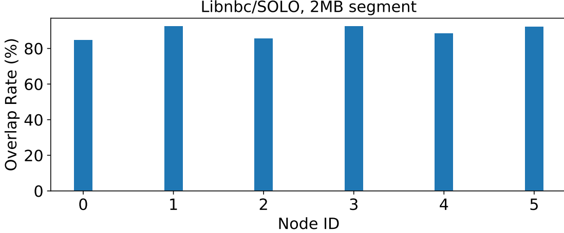
Figure 5.11: Overlap Rate of Concurrent Intra-node and Inter-node Collective Operations (6 nodes, 12 ppn, SOLO module)
