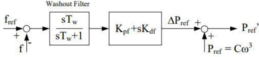
Figure 2.3: Control scheme to provide frequency regulation through inertial response
