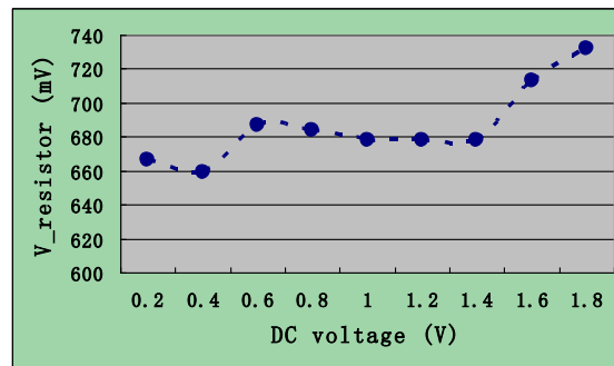
Figure 6-5 The voltage reading from a 120\Omega resistor in series with fluidic system
