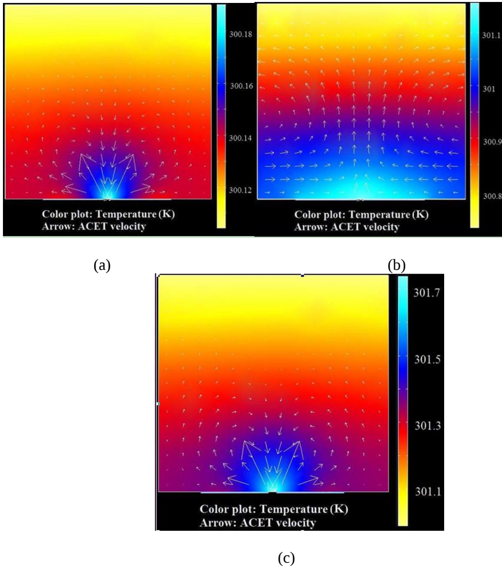
Figure 5-6 Numerical simulation results for solution B, (a) when no surface heating is included at f=1 kHz, the fluid keeps temperature maxima inside it by generating uneven Joule heating. ( V_{rms}=1.8V , Q=0 ) (b) surface heating is included at f=1 kHz (arrow length not to scale). Higher power consumption at surface in tap water solution drags down the temperature peak and causes the flow reversal. ( V_{rms}=1.8V , Q=3125W/m^2 ) (c) at high frequencies ( \sim 10 kHz) Joule heating takes dominance again even when surface heating is considered. Flow exhibits regular pattern. ( V_{rms}=4.84V , Q=1172 W/m^2 )
