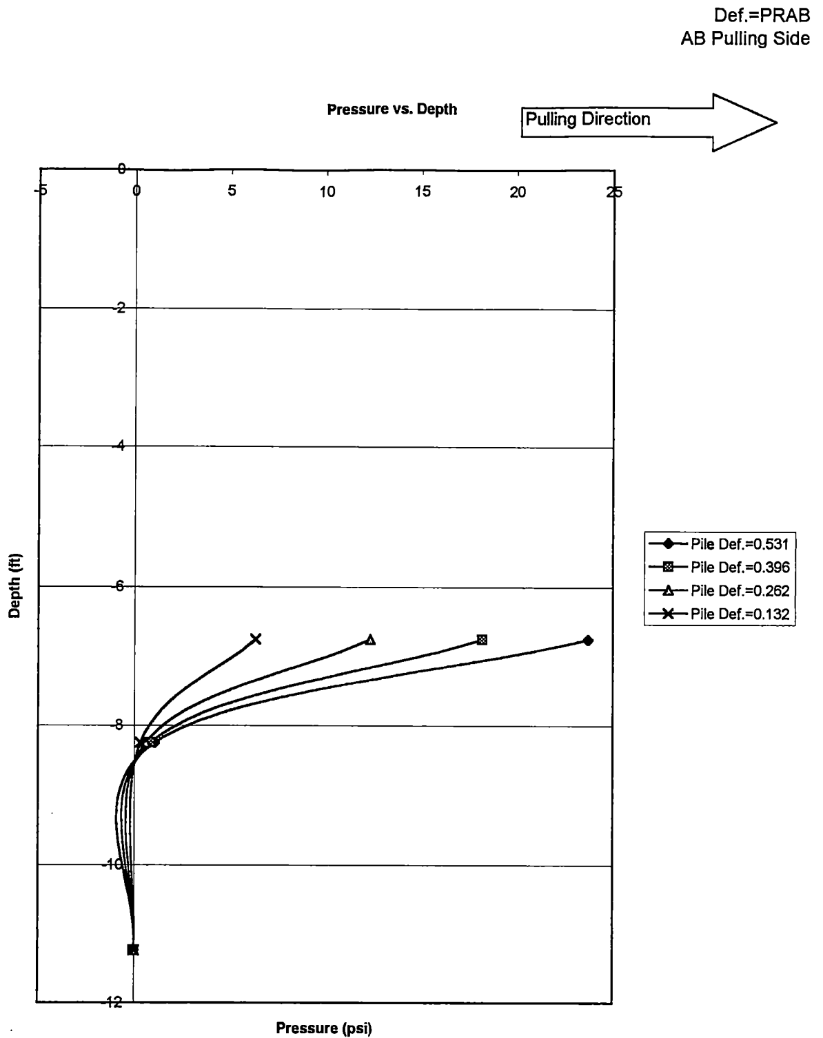
Figure A-12 Pressure vs Depth for pile # 3, pulling west. Second 1/2" test, Oct,9,1999. AB Side
