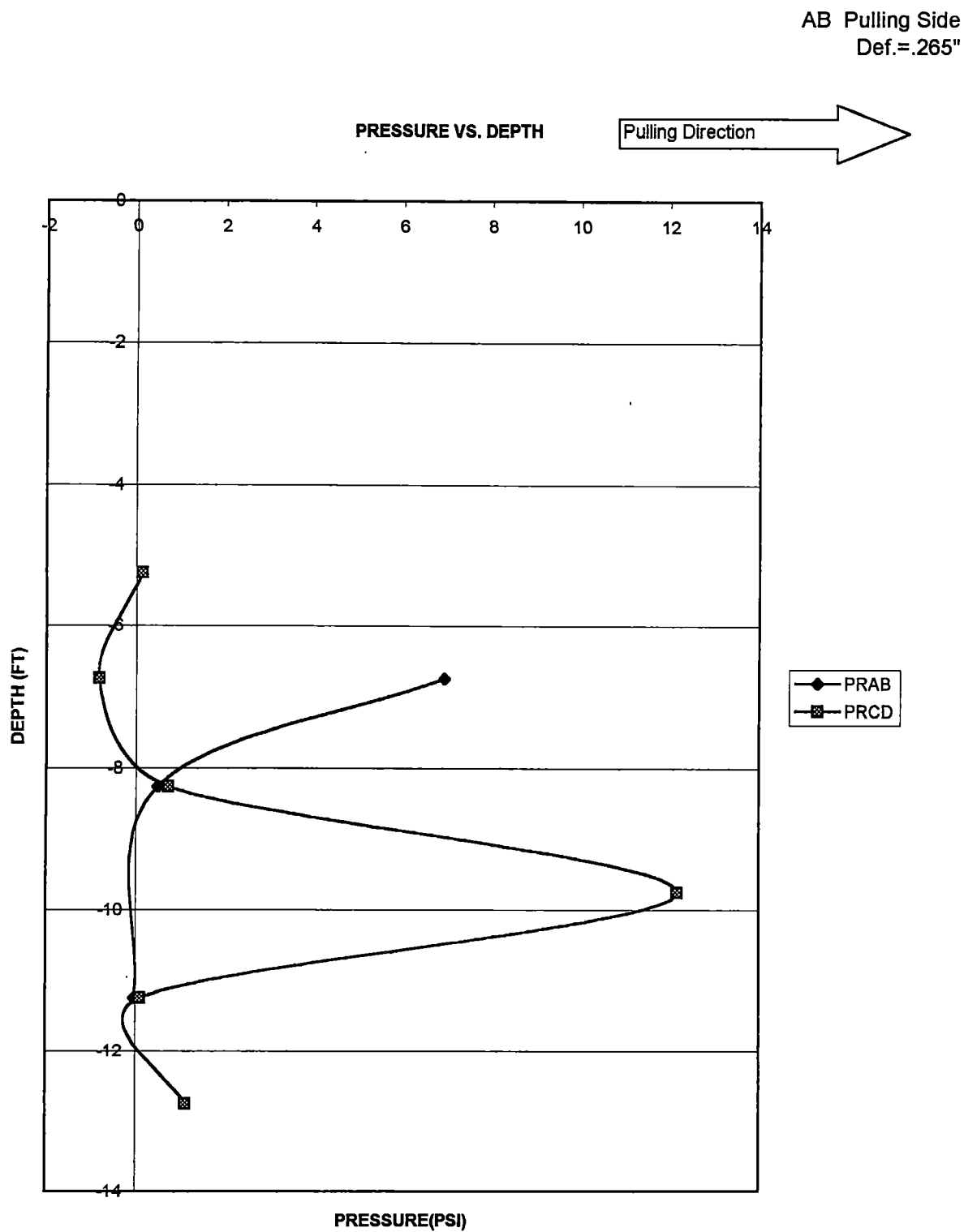
Figure A-2 Pressure vs Depth for pile # 3, pulling west. First 1/2" test, Oct,05,1999. Deflection of the pile=.265"
