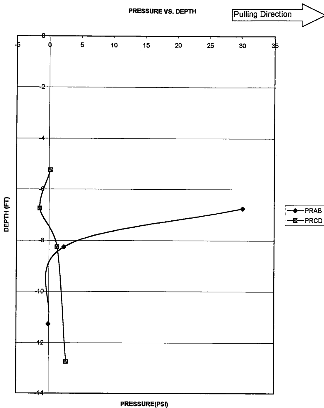
Figure A-30. Pressure vs Depth for pile # 3, pulling west. Second 1" test, Oct,30,1999. Deflection of the pile=.764"
