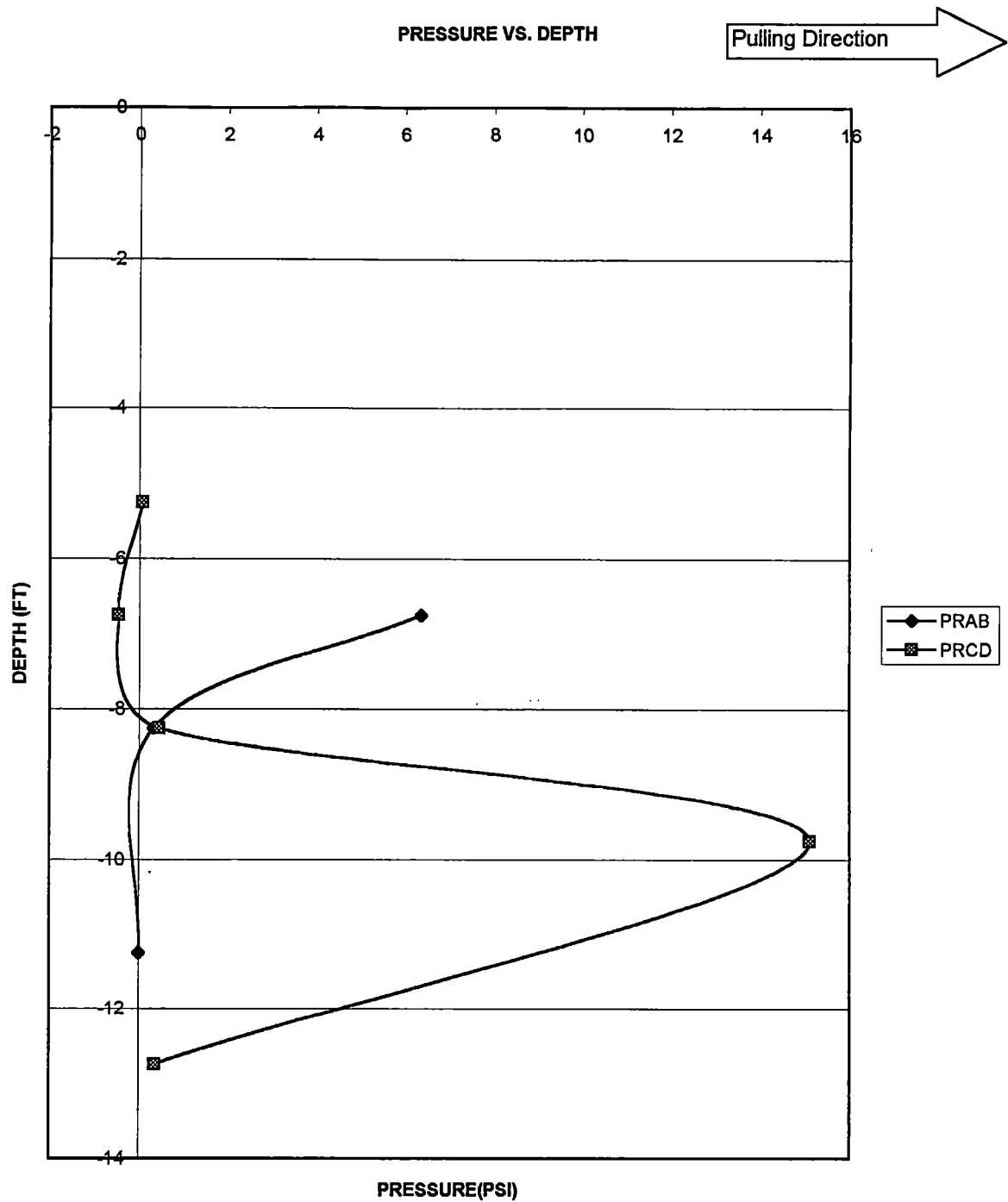
Figure A-7 Pressure vs Depth for pile # 3, pulling west. Second 1/2" test, Oct,9,1999. Deflection of the pile=.132"
