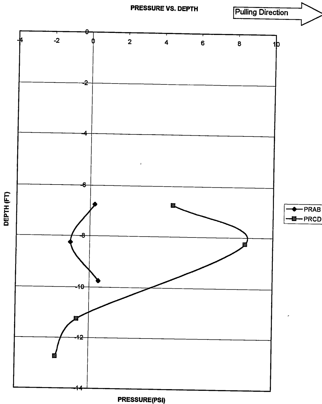
Figure A-44. Pressure vs Depth for pile # 3, pulling east. Second 1/2" test, Feb,5,1999 Deflection of the pile=.247"
