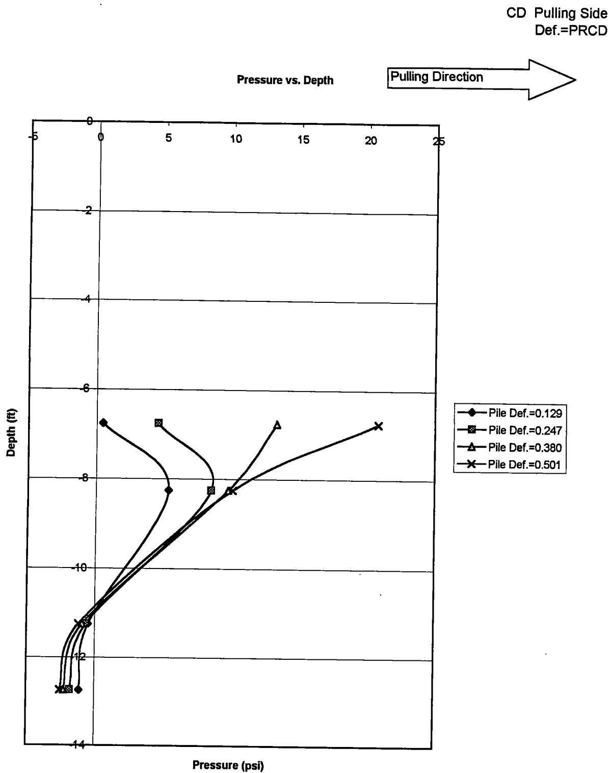
Figure A-47. Pressure vs Depth for pile # 3, pulling east. Second 1/2" test, Feb,5,1999 CD Side
