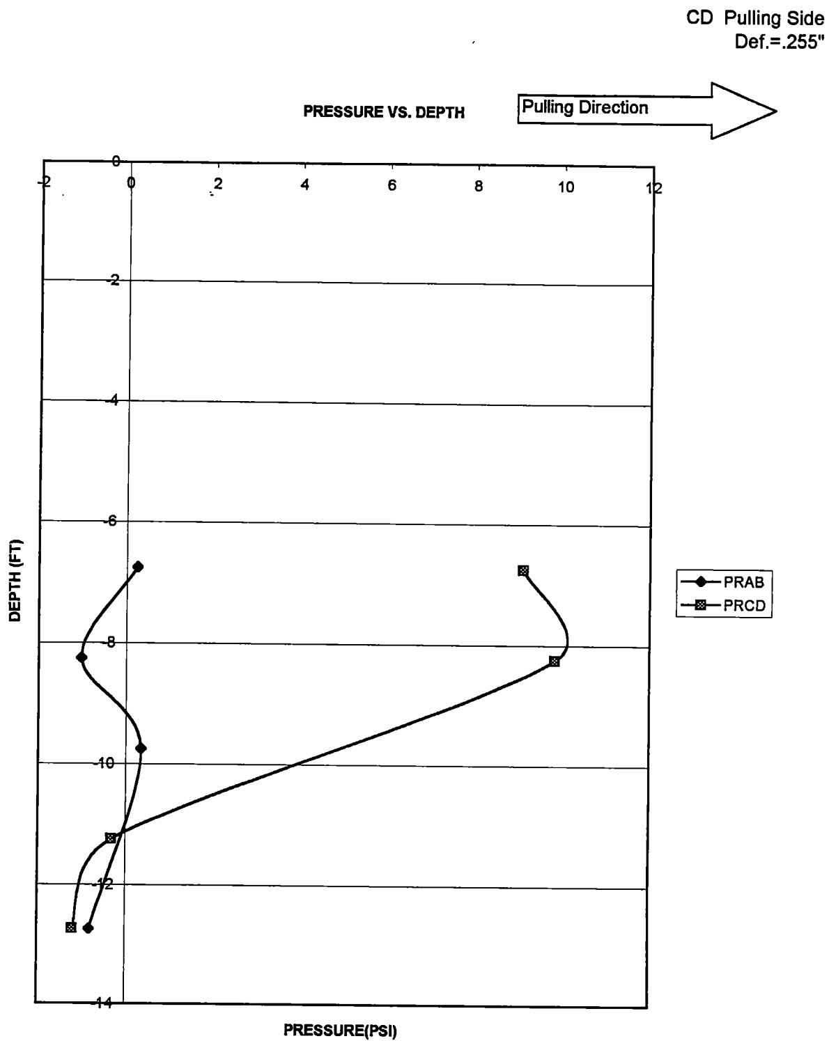
Figure A-49. Pressure vs Depth for pile # 3, pulling east. First 1" test, Feb,26,1999. Deflection of the pile=.255"
