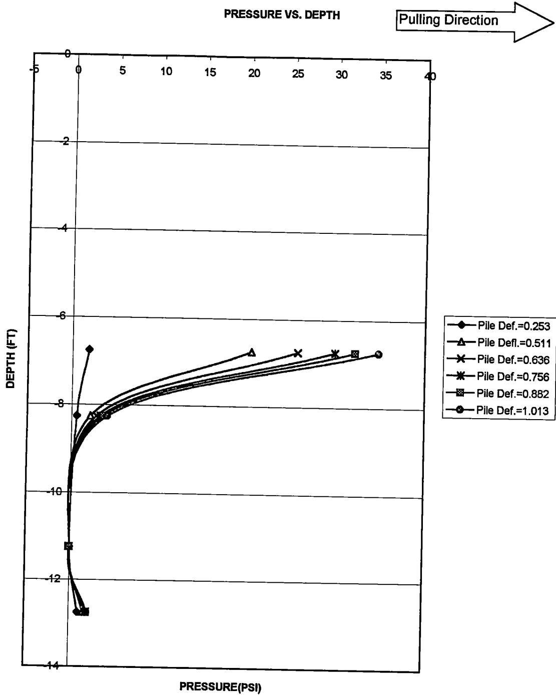
Figure A-41. Pressure vs Depth for pile # 3, pulling west. Third 1" test, Nov,6,1999. AB Side
