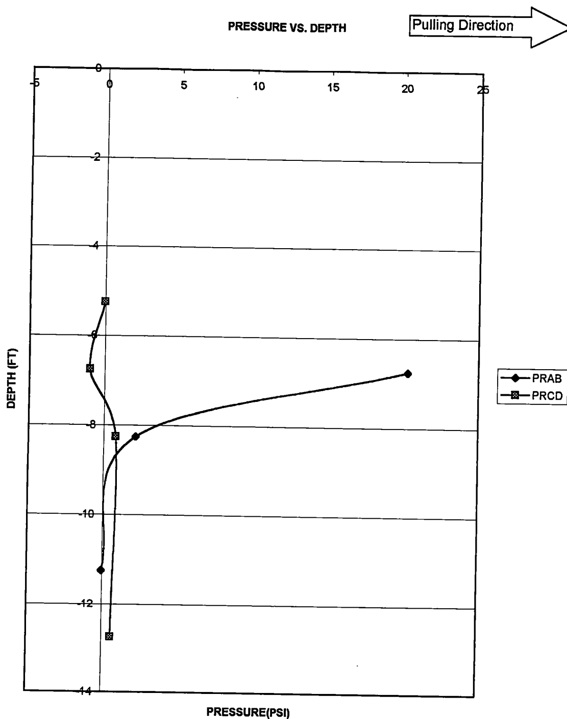
Figure A-36. Pressure vs Depth for pile # 3, pulling west. Third 1" test, Nov,6,1999. Deflection of the pile=.511"
