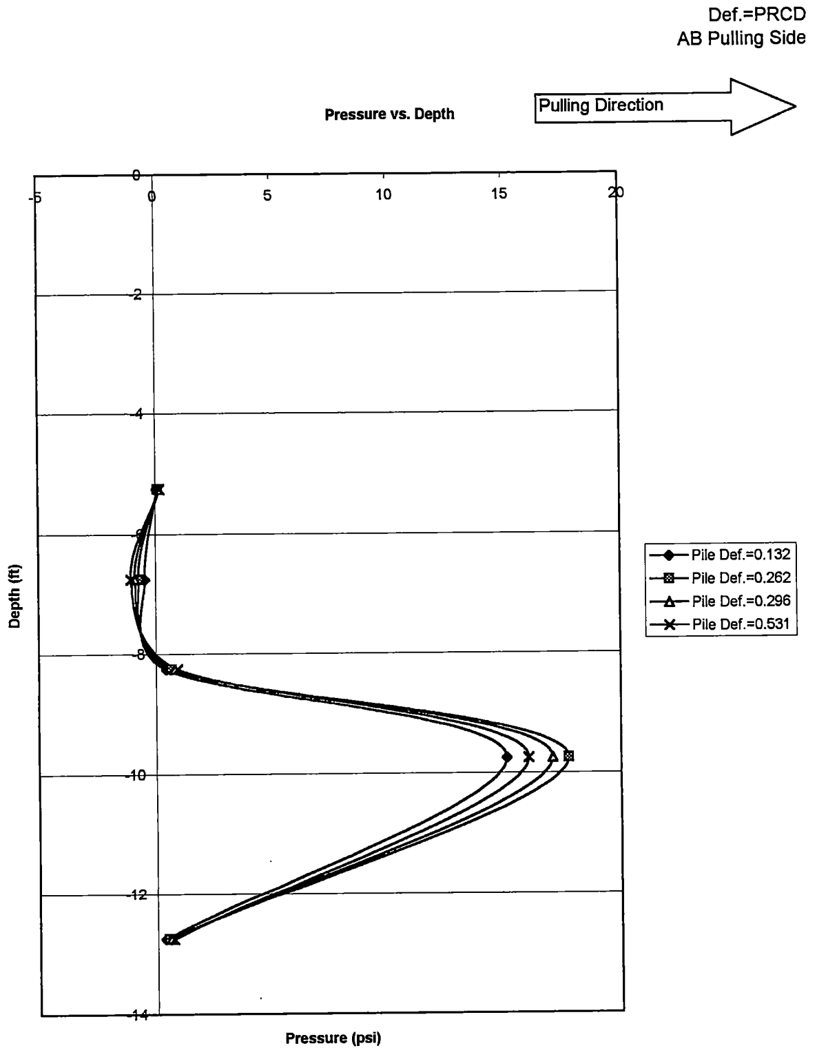
Figure A-11 Pressure vs Depth for pile # 3, pulling west. Second 1/2" test, Oct,9,1999. CD Side
