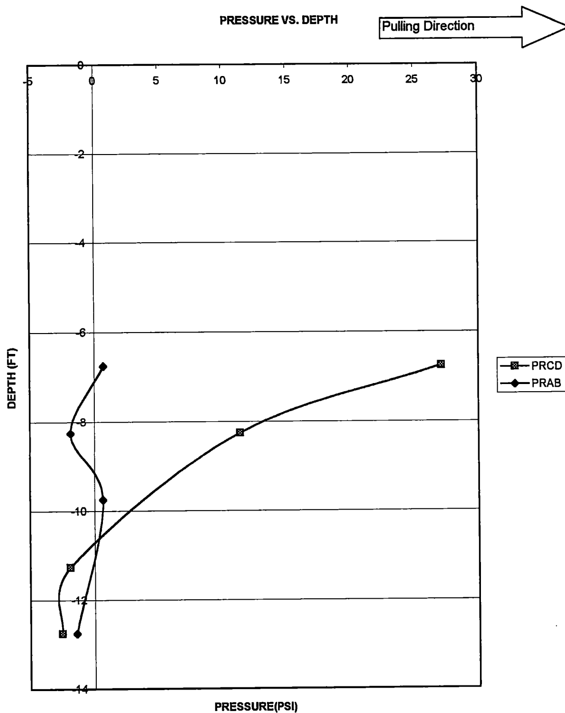
Figure A-51. Pressure vs Depth for pile # 3, pulling east. First 1" test, Feb,26,1999. Deflection of the pile=.652"
