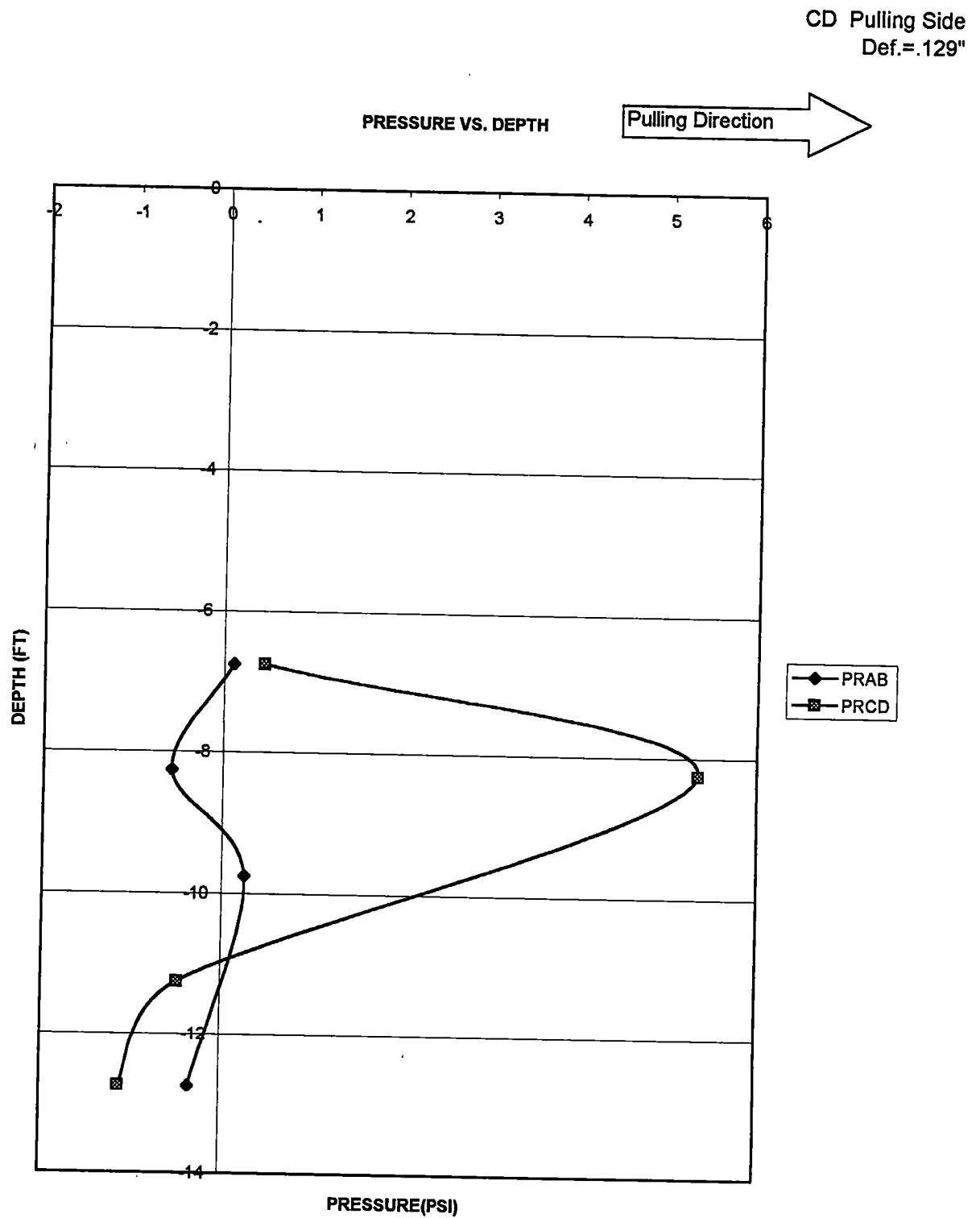
Figure A-43. Pressure vs Depth for pile # 3, pulling east. Second 1/2" test, Feb,5,1999 Deflection of the pile=.129"
