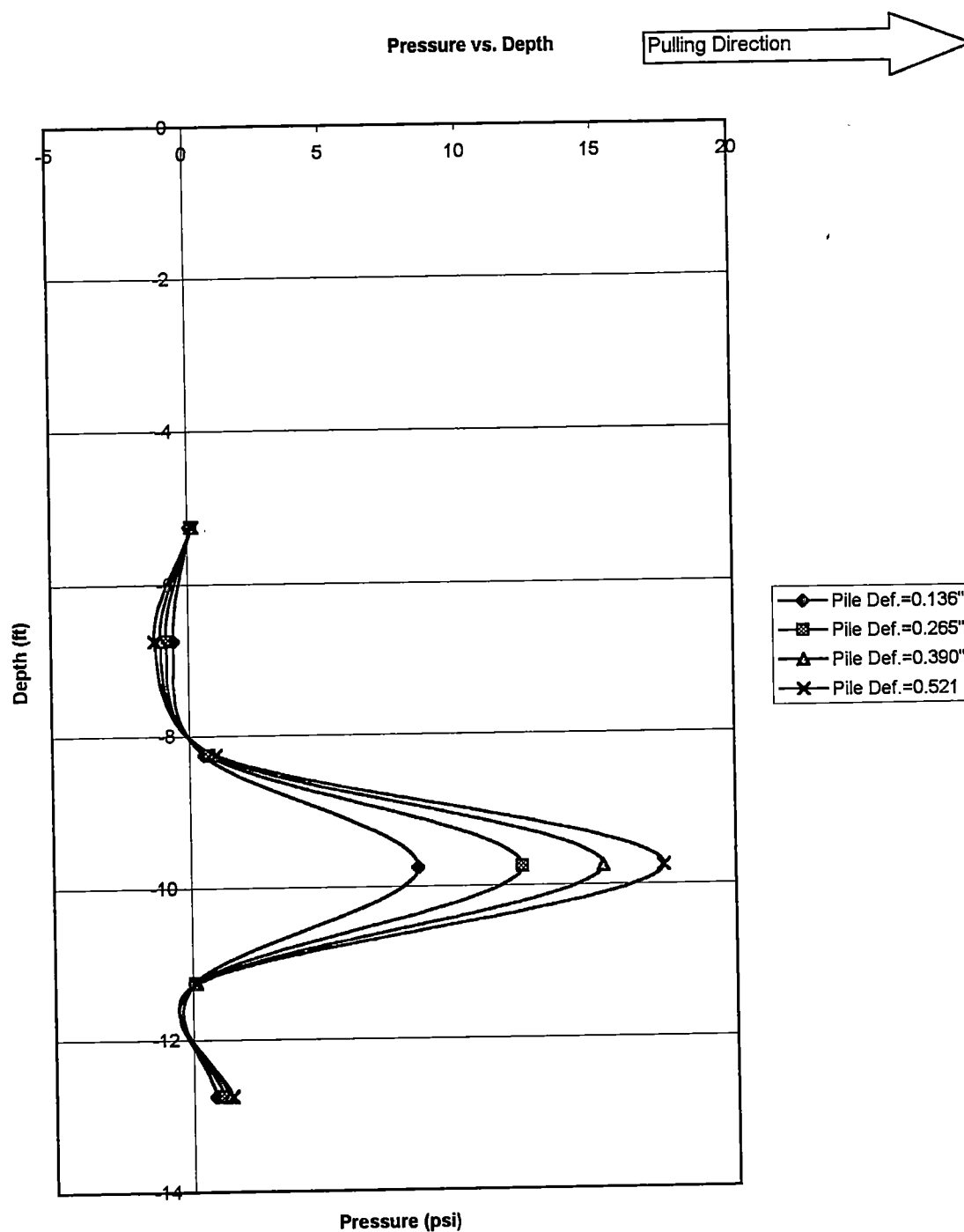
Figure A-5 Pressure vs Depth for pile # 3, pulling west. First 1/2" test, Oct,05,1999. CD Side
