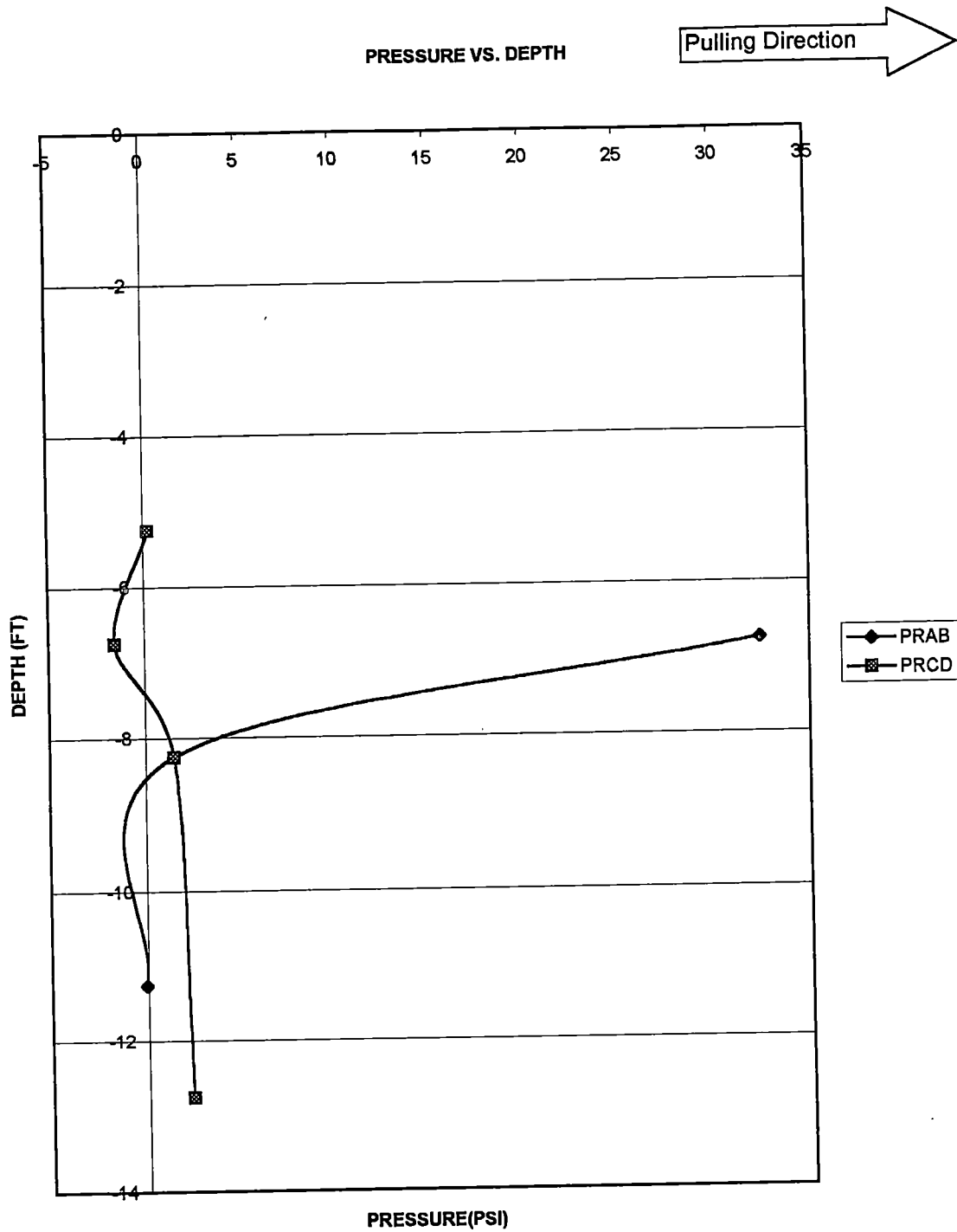
Figure A-24. Pressure vs Depth for pile # 3, pulling west. First 1" test, Oct,23,1999. Deflection of the pile=1.031"
