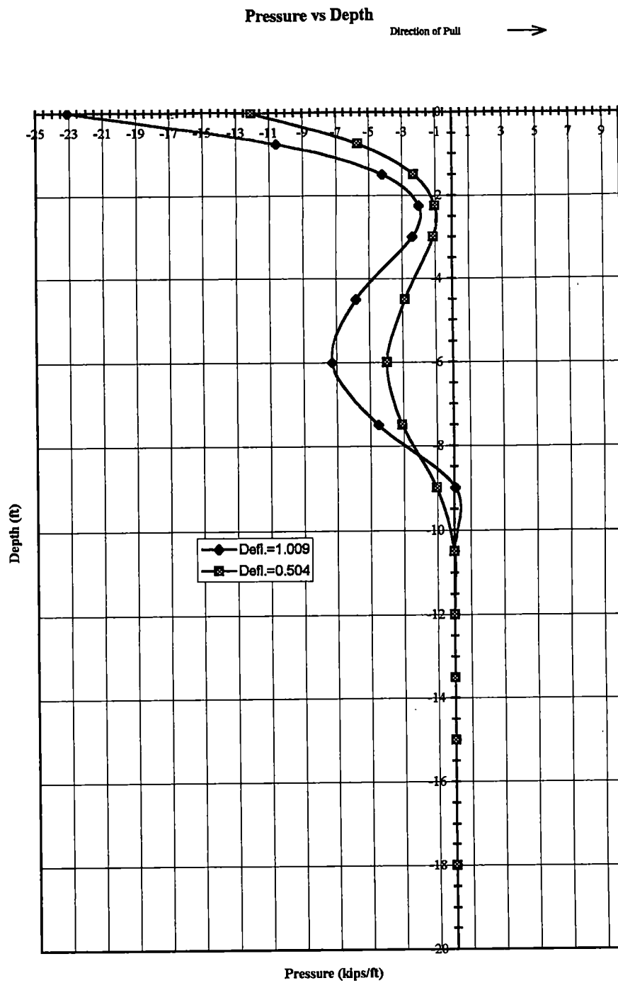
Figure (B-16). Pressure vs Depth from Strain Gage Data. First 1" test, Feb, 26, 1999 Strain gage data
