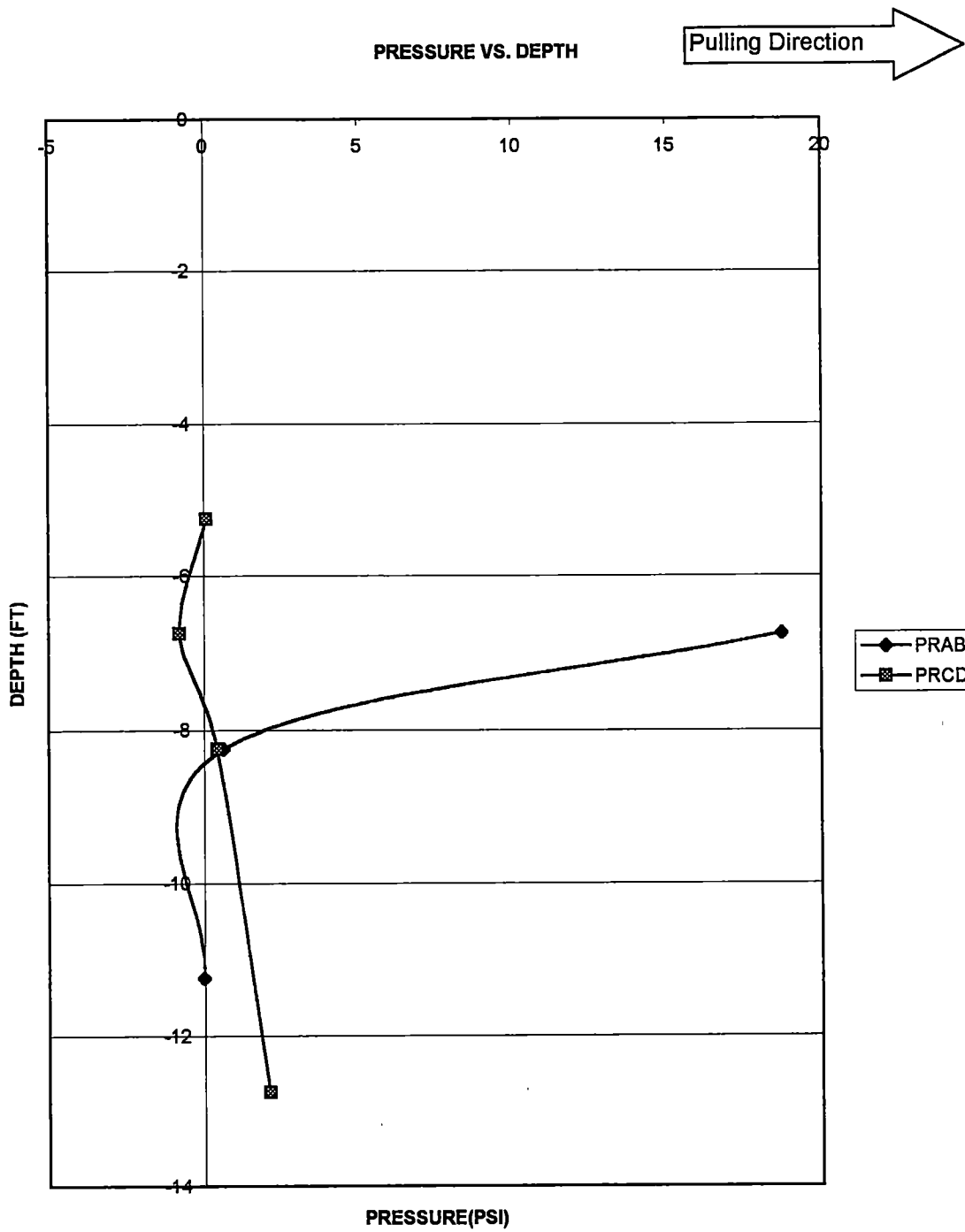
Figure A-19. Presure vs Depth for pile # 3, puling west. First 1" test, Oct,23,1999. Deflection of the pile=.255"
