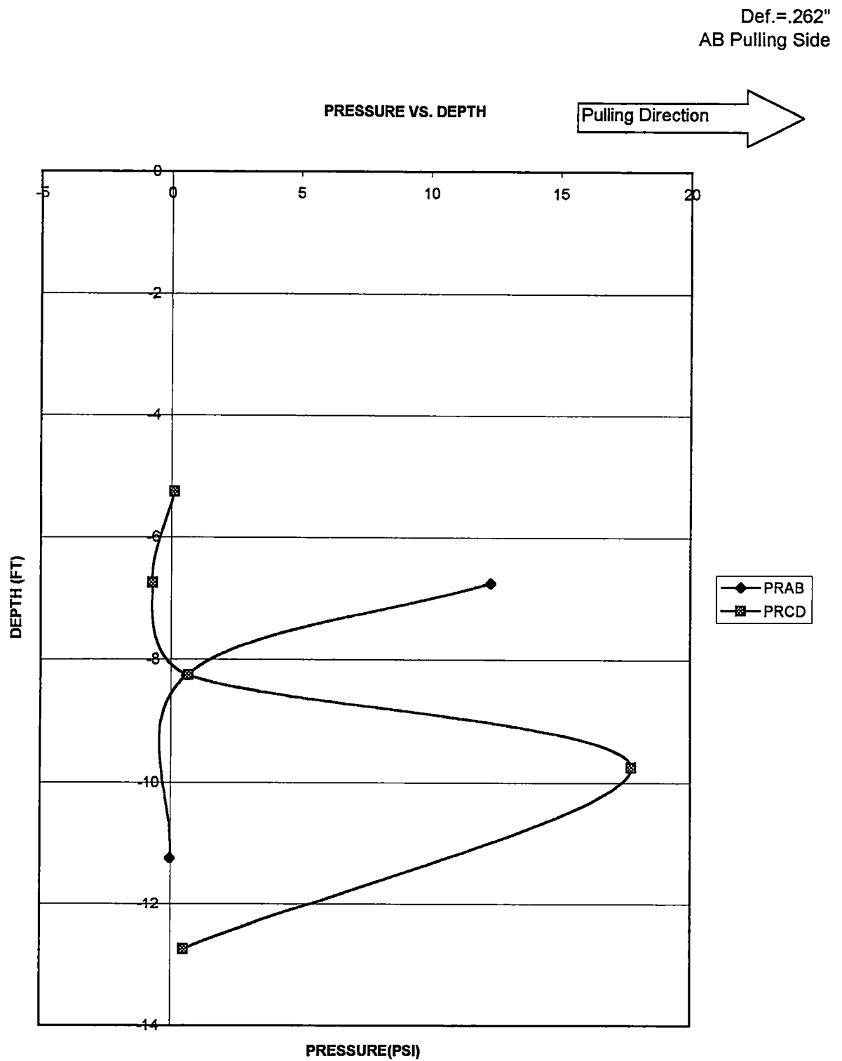
Figure A-8 Pressure vs Depth for pile # 3, pulling west. Second 1/2" test, Oct,9,1999. Deflection of the pile=.262"
