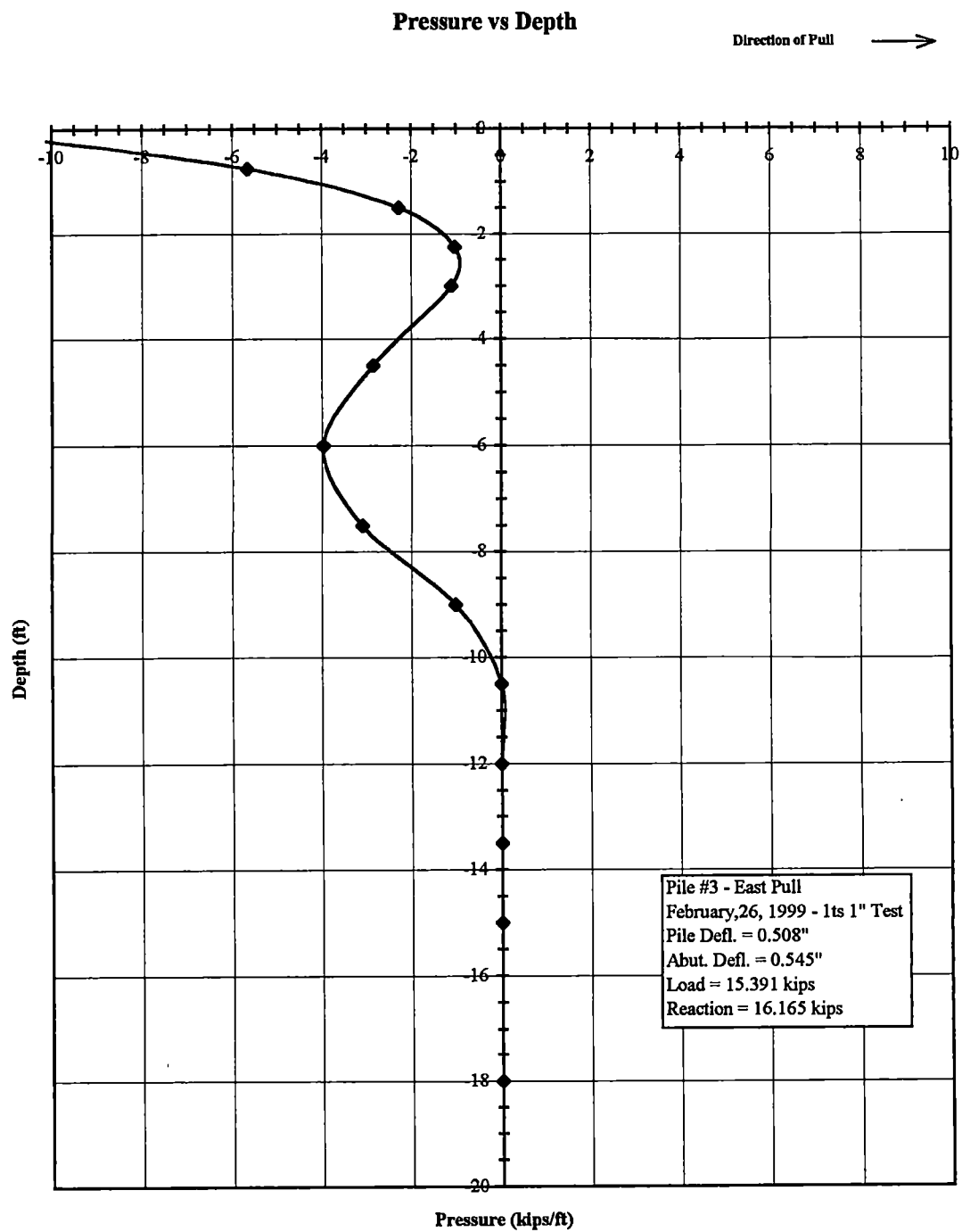
Figure (B-14), Pressure vs Depth from Strain Gage Data. First 1" test, Feb, 26, 1999 Strain gage data, deflection of the pile=0.5"
