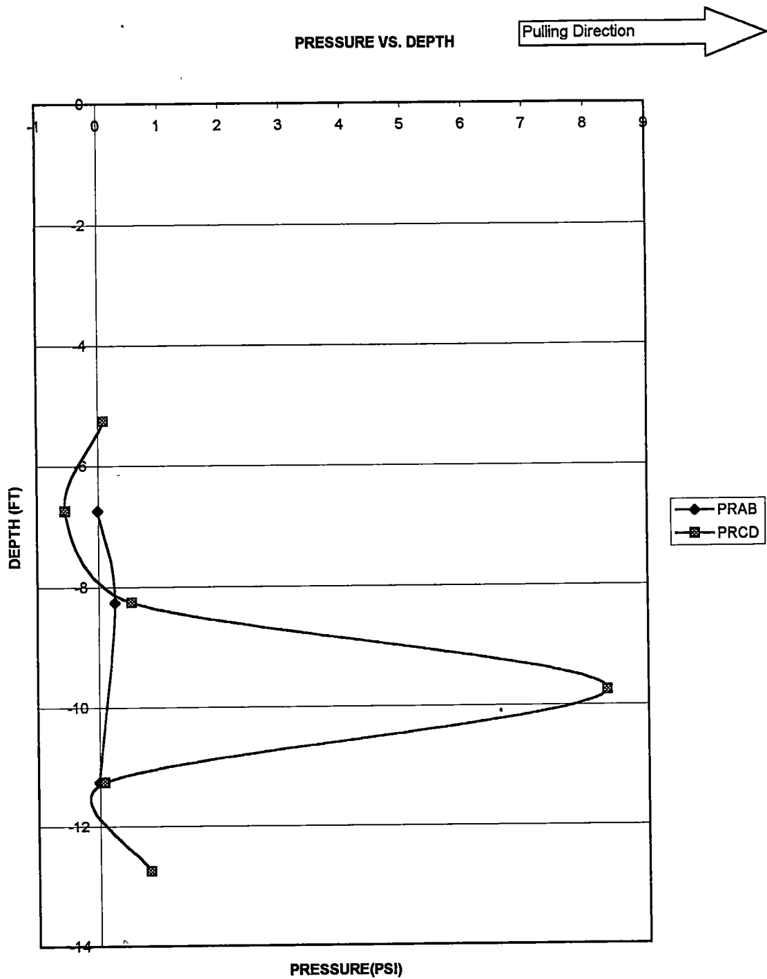
Figure A-1 Pressure vs Depth for pile # 3, pulling west. First 1/2" test, Oct,05,1999. Deflection of the pile=.136"
