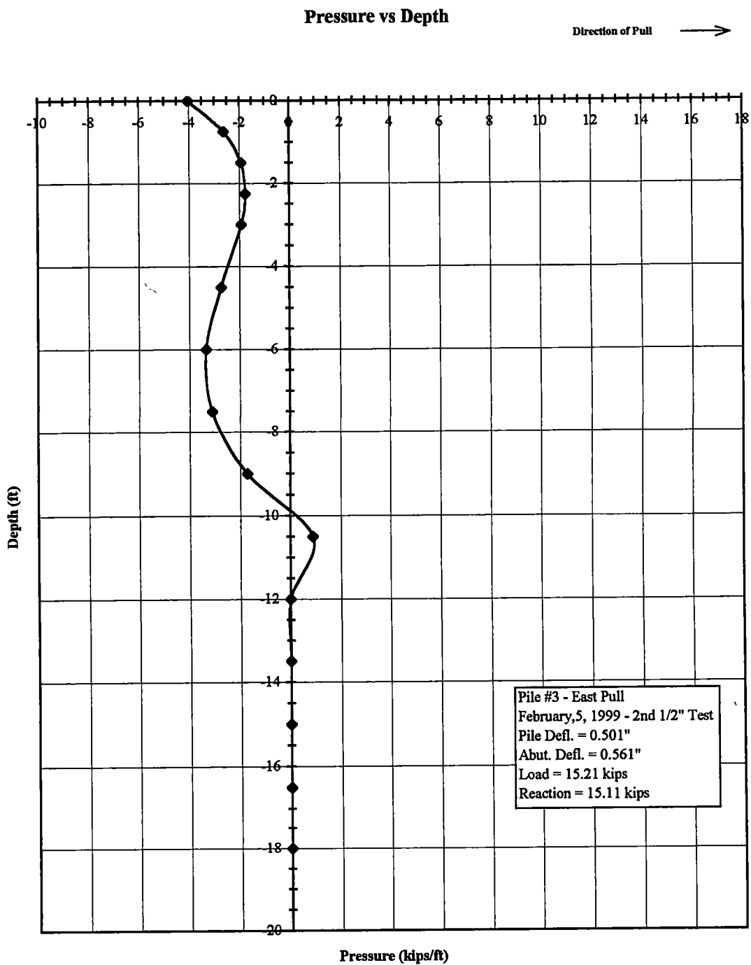
Figure (B-13). Pressure vs Depth for pile # 3, pulling east. Second 1/2" test, Feb, 05, 1999 Strain gage data
