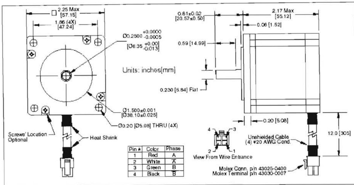
Figure 6: STP-MTR-23055 Motor Dimensions (image courtesy of automationdirect.com )
