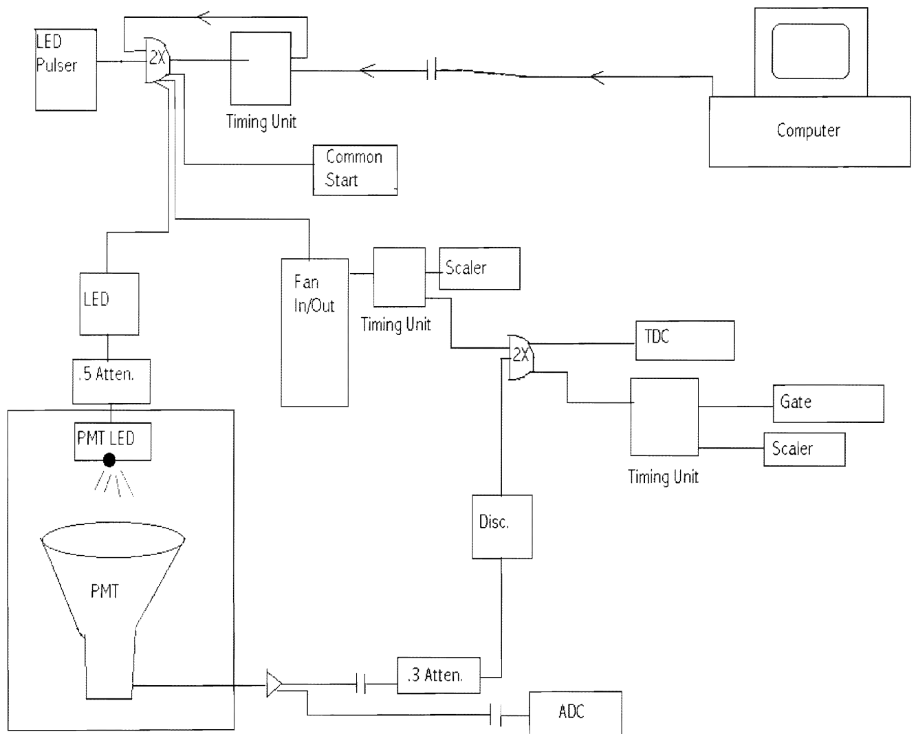
Fig. 6 “NIM/CAMAC-based Data Acquisition”
