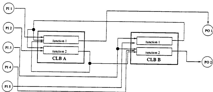
Figure 4.4: Two-function CLBs
