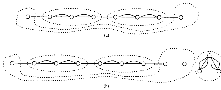
Figure 5.5: Partitioning the graphs of Figures 5.4(a)
