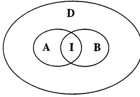
Figure 2.4: C1 = A \cup I, C2 = B \cup I
