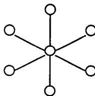
Figure 2.2: A star graph with six rays
