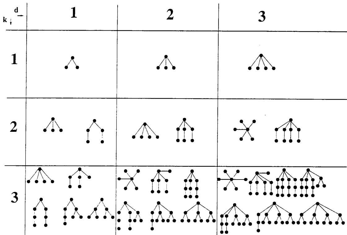
Figure 2.7: kdq -trees
