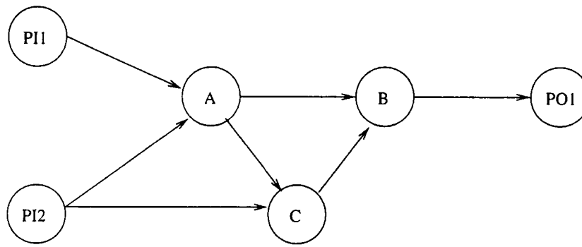
Figure 4.3: A connection graph
