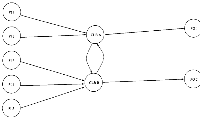
Figure 4.6: A cyclic connection graph
