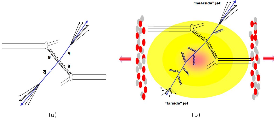
Figure 1.6: (a) A production of a pair of jets in a nucleon-nucleon collision. (b) An illustration of the associated pair of jets traveling through the dense deconfined medium created as a result of the collision of two heavy ions.
