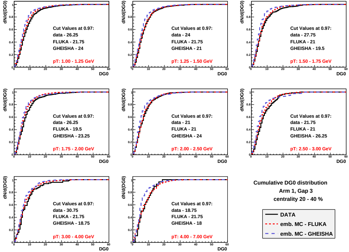
Figure 4.8: Comparison of data and simulation for the corresponding cumulative distribution, f(DG0) , calculated using Equation 4.5 for each p_T bin.
