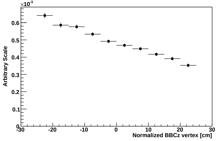
Figure 4.2: Distribution of the vertex position along the beam pipe (z-coordinate) of the muon candidate tracks in the north arm (situated in the positive z-direction) normalized with the event vertex z-coordinate distribution, BBCz.
