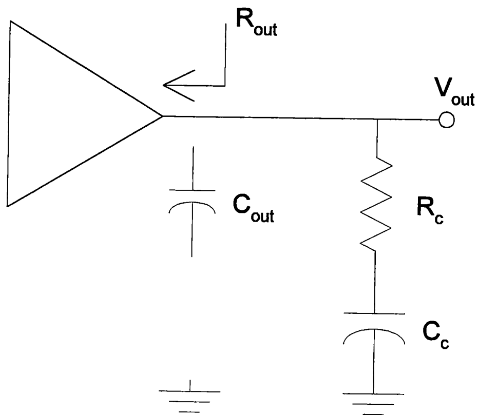
Figure 38 – Lead Compensation
