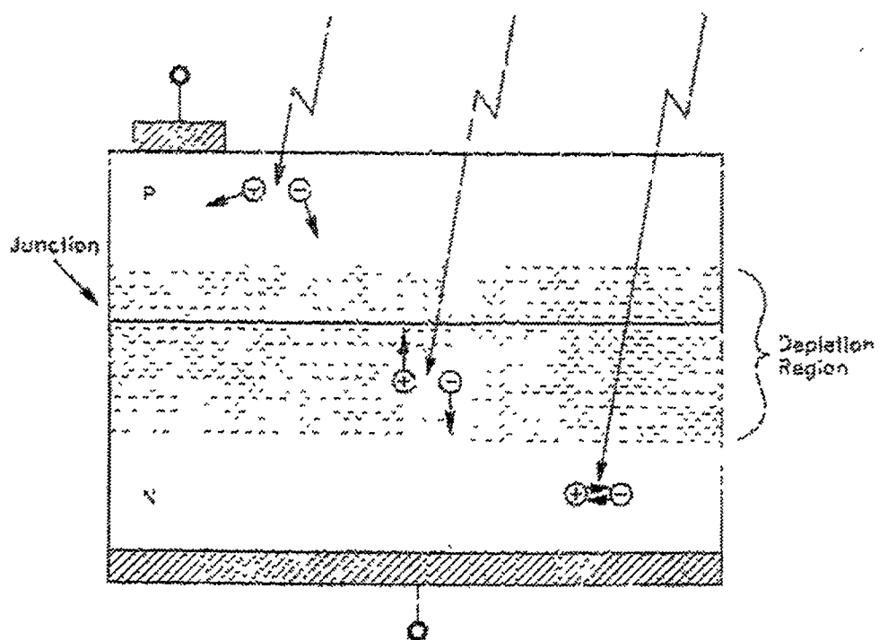
Figure 3 - Photodiode Operation
