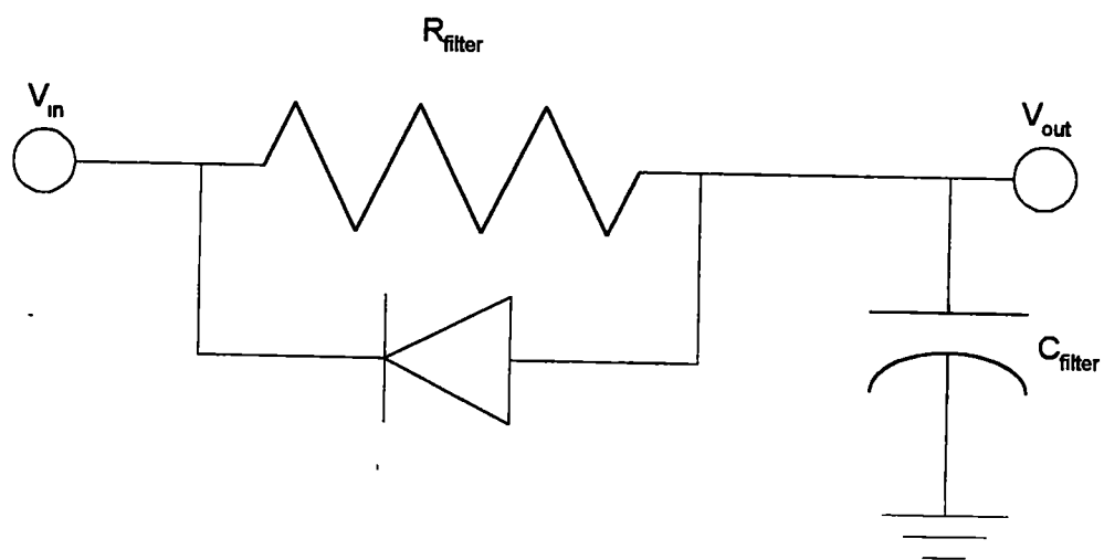
Figure 17 - Low-pass Filter
