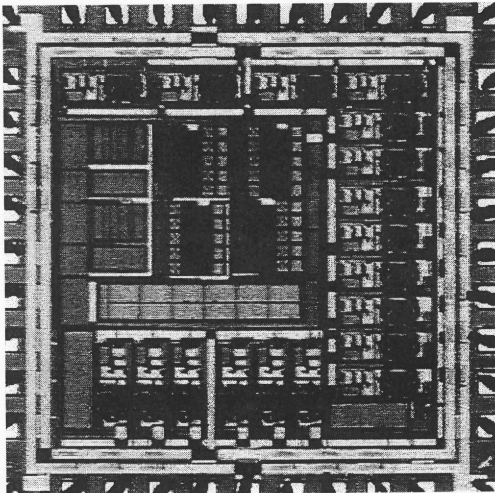
Figure 8 - CMOS Photodetector Evaluation Test Chip
