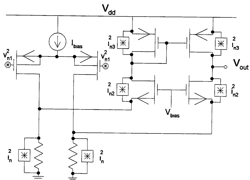
Figure 37 – Folded Cascode Amplifier with Noise Sources
