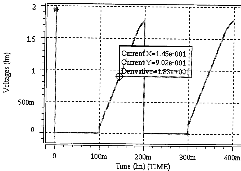
Figure 42 – Gain Error Measurement (Switched Integrator Output)
