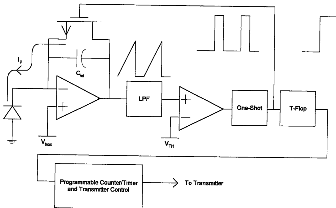
Figure 10 - Light-to-Frequency Converter
