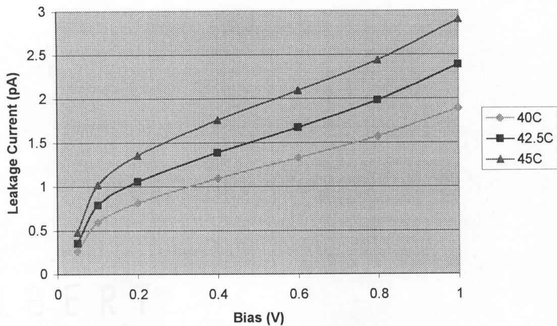
Figure 57 – Detector Leakage vs. Temperature and Bias
