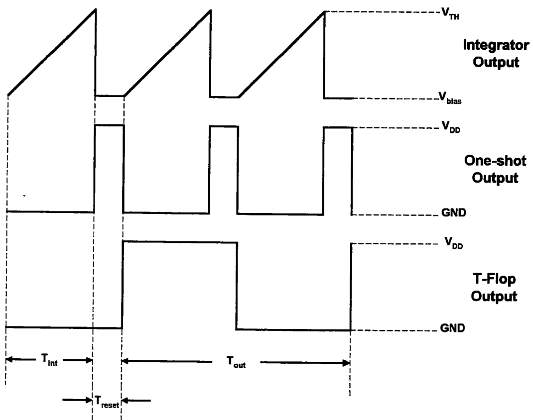
Figure 11 - System Timing
