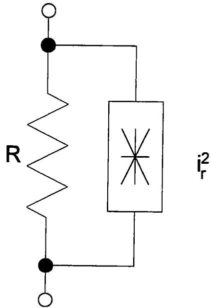
Figure 35 – Resistor Noise Model
