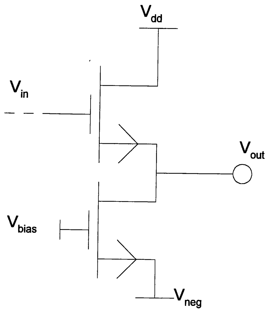
Figure 34 – Output Buffer
