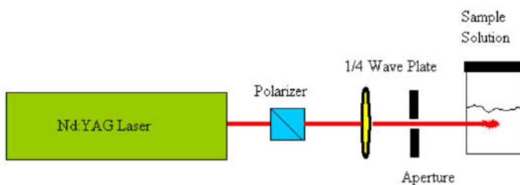
Figure 21. The experimental setup for the laser-induced crystallization of glycine using unfocused laser light.
