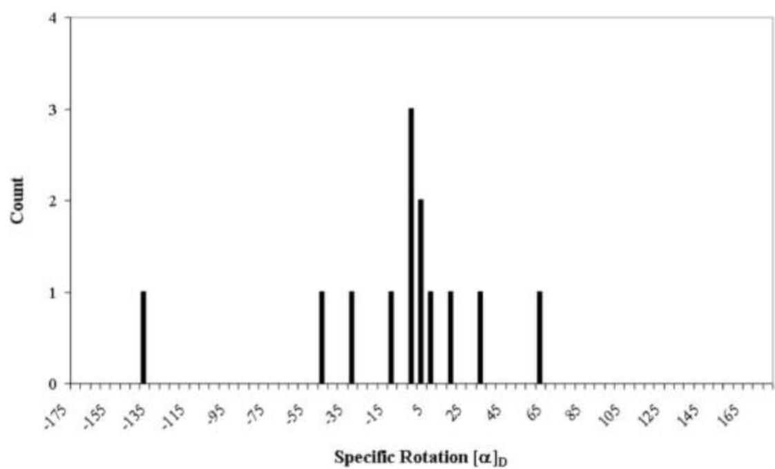
Figure 12. The frequency of specific rotations for the thirteen 1,1'-binaphthyl samples not placed under the \text{Sr}^{90} beta source.
