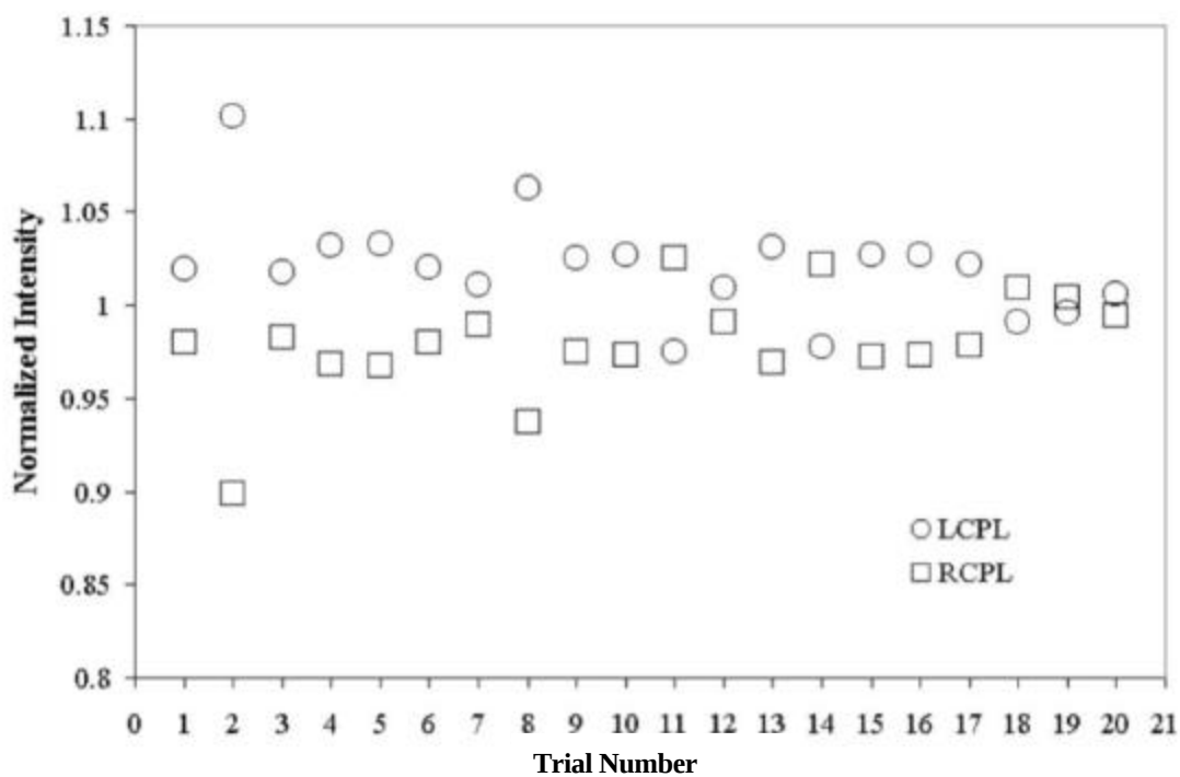
Figure 9. The normalized signal intensities for the (2+1) REMPI of (R)-(+)-3-methylcyclopentanone using left and right circularly polarized light with a wavelength of 397.5nm. The LCPL and RCPL refer to left and right circularly polarized light respectively.
