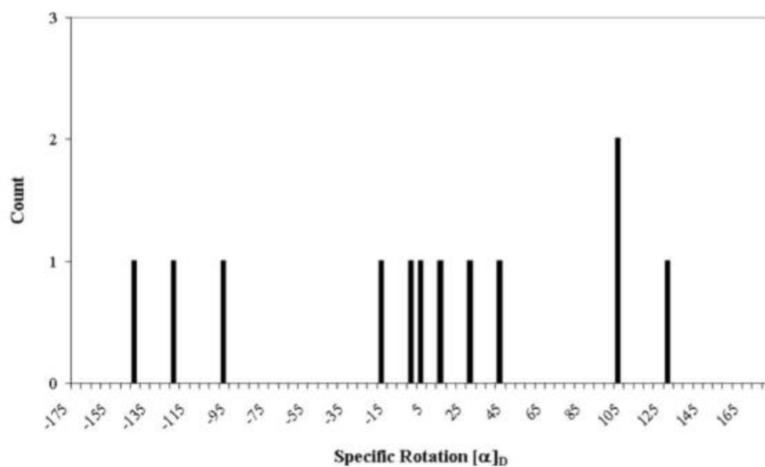
Figure 13. The frequency of specific rotations for the twelve 1,1'-binaphthyl samples placed under the \text{Sr}^{90} beta source.
