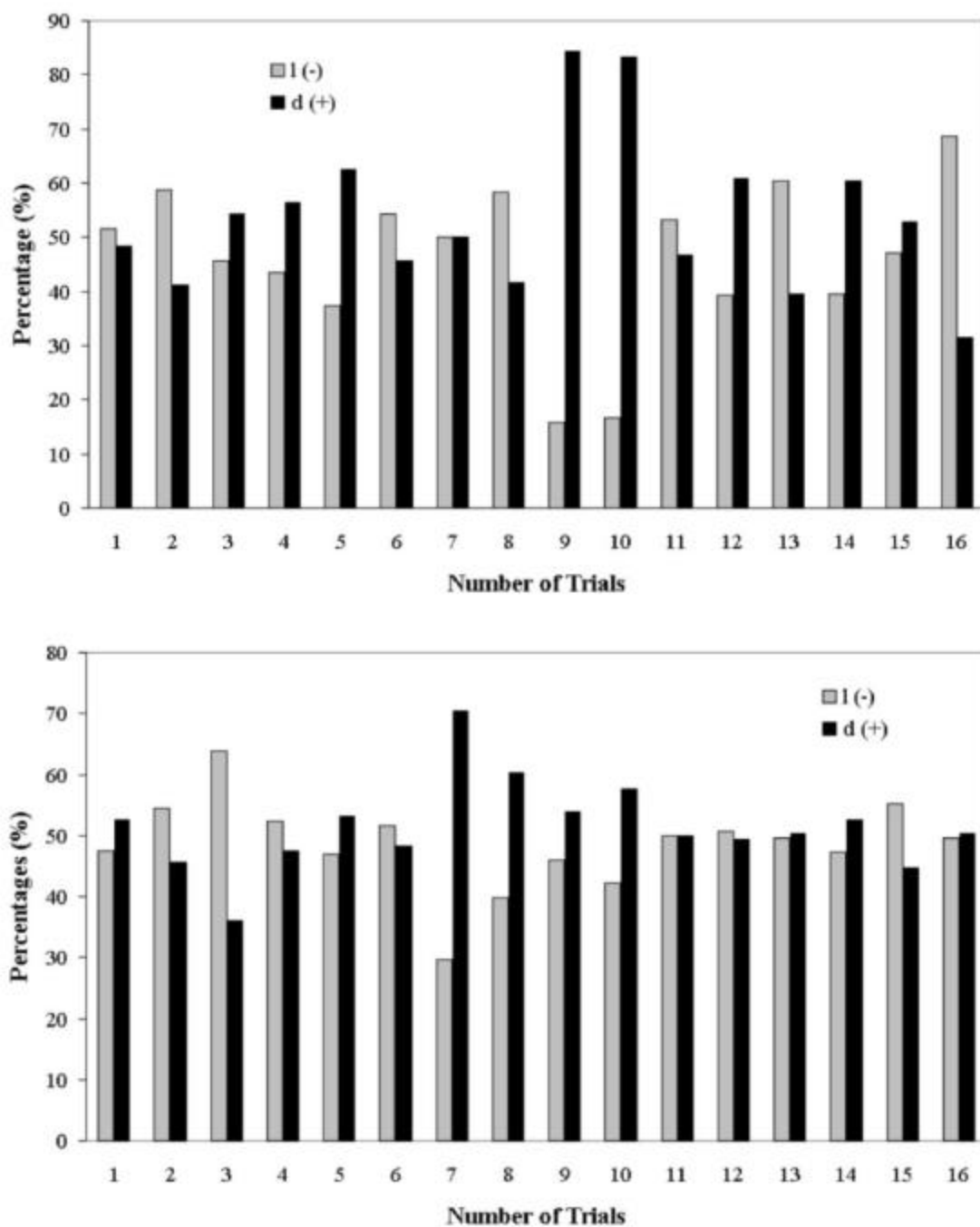
Figure 17. Histograms for the laser induced crystallization of sodium chlorate crystals grown in Petri dishes from the irradiation of right circularly polarized light (top) and from the crystallization of controlled sodium chlorate crystals (bottom).
