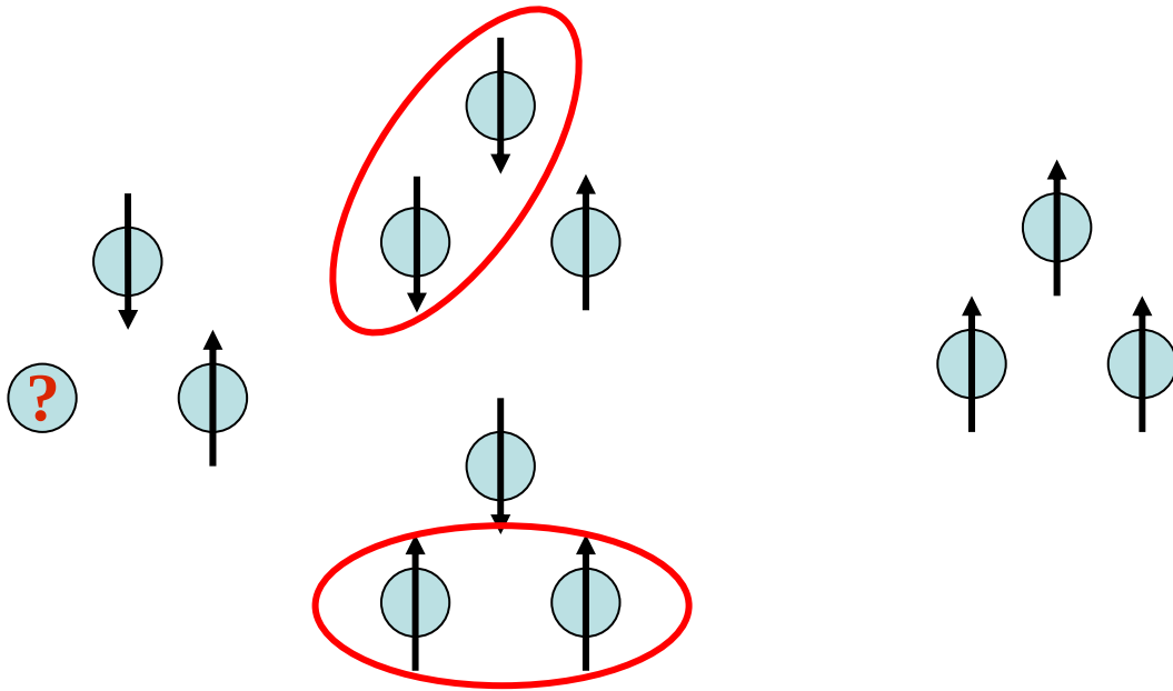
Fig. 8. Magnetic moment orientation in a triangular lattice. Left: Ambiguity and subsequent geometric frustration with anti-ferromagnetic exchange interactions. Right: Absence of geometric frustration when ferromagnetic interactions are observed.
