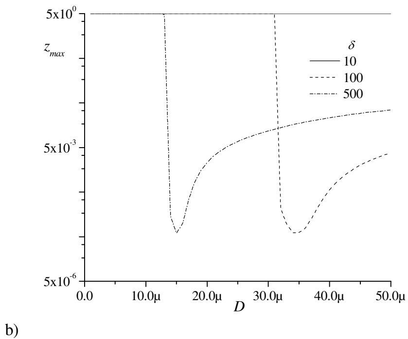
Figure 5-8 Maximum radial and axial distances travelled by particles in a BDVE for different density ratios.
