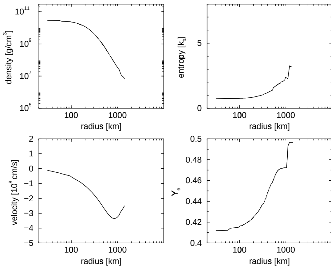
Figure 7.1: Initial conditions for the Nomoto-Hashimoto 15M_{\odot} model
