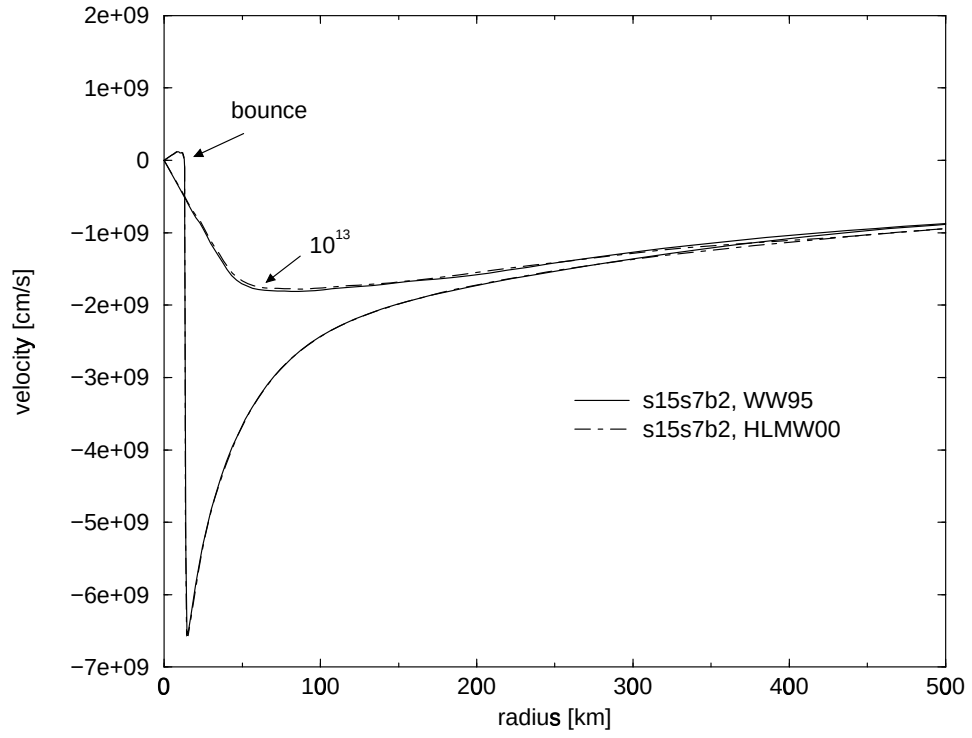
Figure 6.7: Velocity profiles for central densities of 1 \times 10^{13} and 2.96 \times 10^{14} \text{ g/cm}^3
