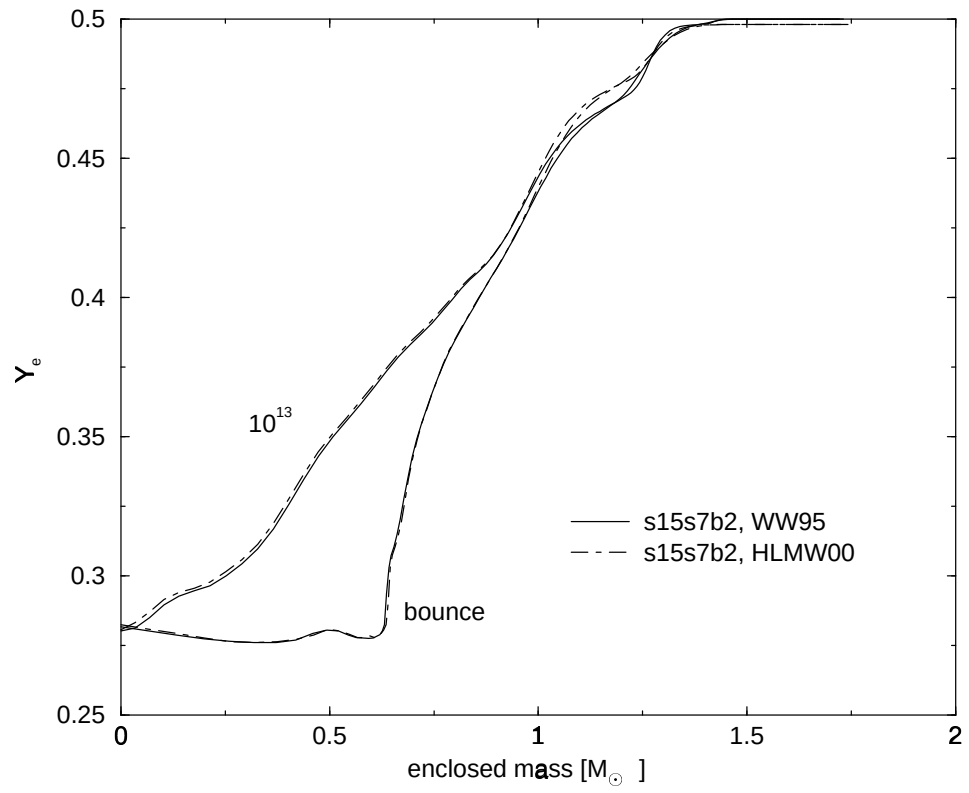
Figure 6.5: Y_e profiles for central densities of 1 \times 10^{13} and 2.96 \times 10^{14} g/cm^3
