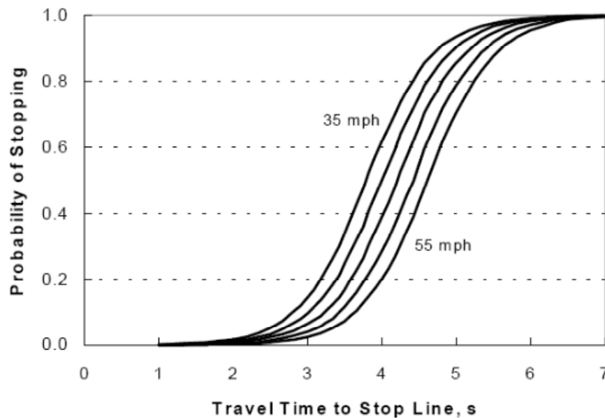
Figure 4.3 Probability of stopping as a function of travel time to stop line in different speeds ( Bonneson et al., 2001 )
