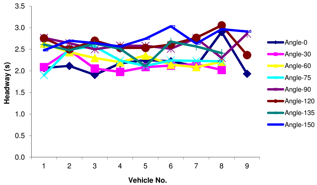
a) Tangent = 0
