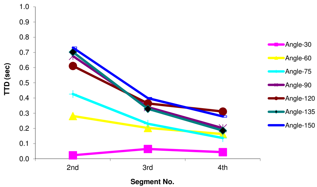
a) Tangent = 0
