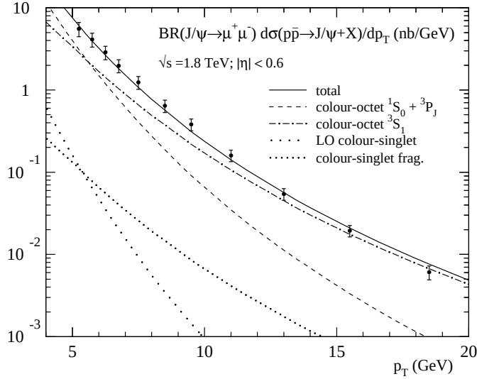
Figure 2.5: Color Octet Model contributions to J/\psi production at high p_T [7].
