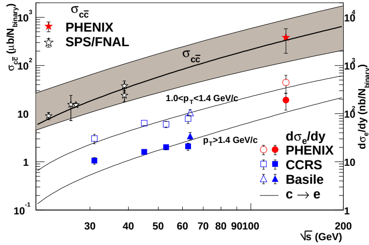
Figure 5.7: Single electron production at RHIC and ISR experiments [19]. Open and closed symbols are for 1.0 < p_T < 1.4 GeV/ c and p_T > 1.4 GeV/ c respectively (right-hand scale). The left-hand scale indicates the charm contribution derived from PYTHIA.
