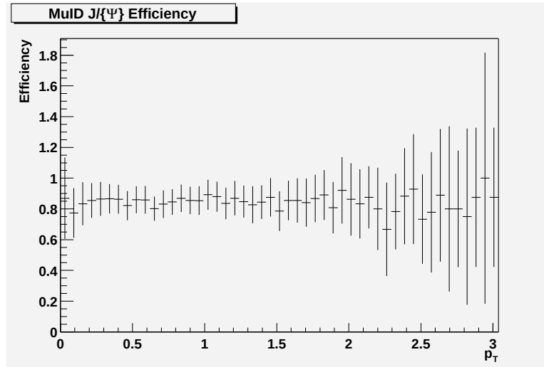
Figure 4.13: Transverse momentum dependance of MuID reconstruction efficiency of the J/\psi within the Muon Tracker acceptance using realistic MuID hardware efficiencies.
