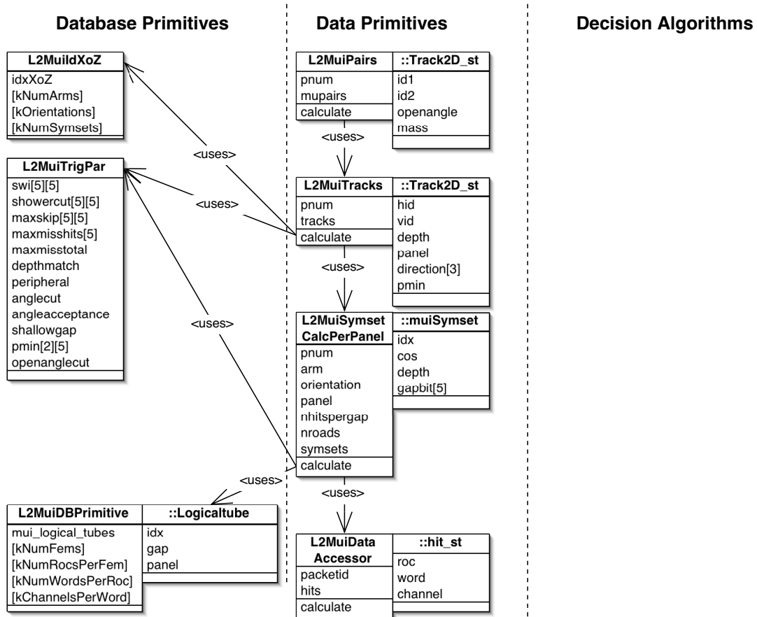
Figure 3.17: Muon Level 2 Trigger Overview
