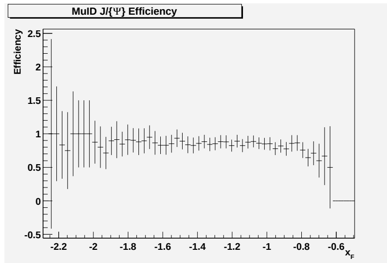
Figure 4.14: Longitudinal momentum dependance of MuID reconstruction efficiency of the J/\psi within the Muon Tracker acceptance using realistic MuID hardware efficiencies.
