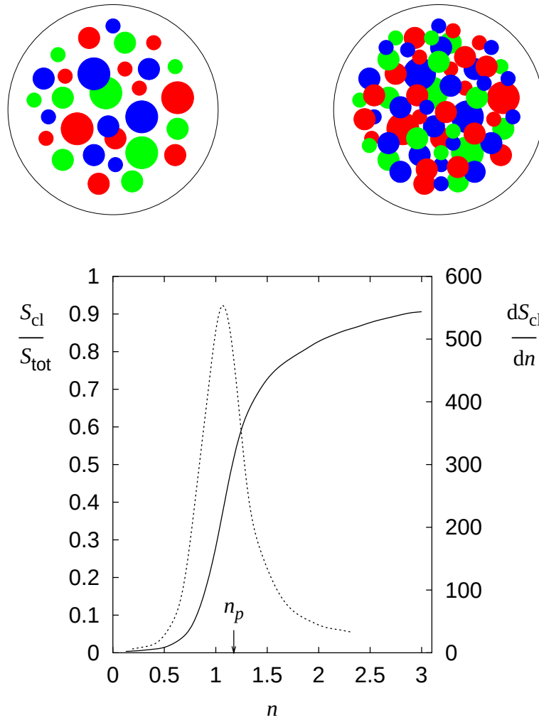
Figure 2.8: The overlap of colored clusters in low density (upper left) and in high density (upper right). The average cluster size (solid) and its derivative (dotted) as a function of the cluster density.[10]
