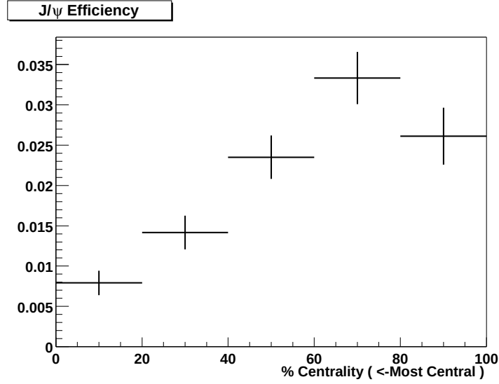
Figure 4.26: The centrality dependence of the Acceptance×Efficiency of J/\psi 's with rapidity -2.2 < y < -1.1 into the south spectrometer. Efficiency is calculated by embedding simulated decay muons into a real Au+Au collision.
