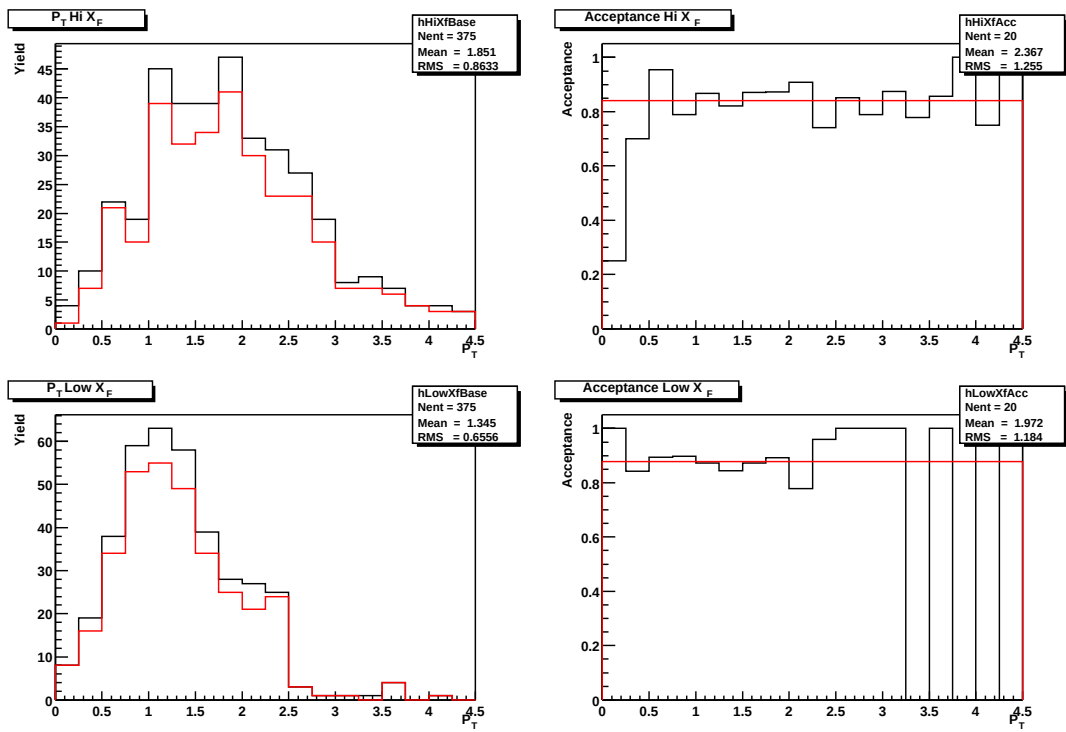
Figure 3.18: Muon Level 2 Acceptance for J/\psi requiring deeply penetrating muons.
