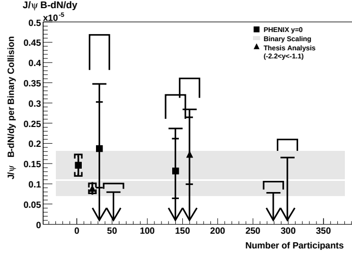
Figure 5.9: The J/\psi invariant yield per binary collision is shown from proton+proton reactions and three exclusive centrality ranges of Au+Au reactions all at \sqrt{S_{NN}} = 200 GeV for both mid-rapidity and forward rapidity measurements. (The values of the forward rapidity have been shifted by +20 units along the x-axis for clarity.)
