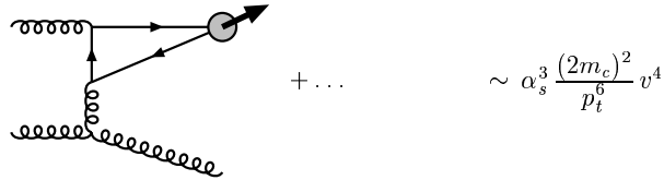
Figure 2.4: Production diagrams for J/\psi and \psi' and there corresponding p_T dependence [7].
