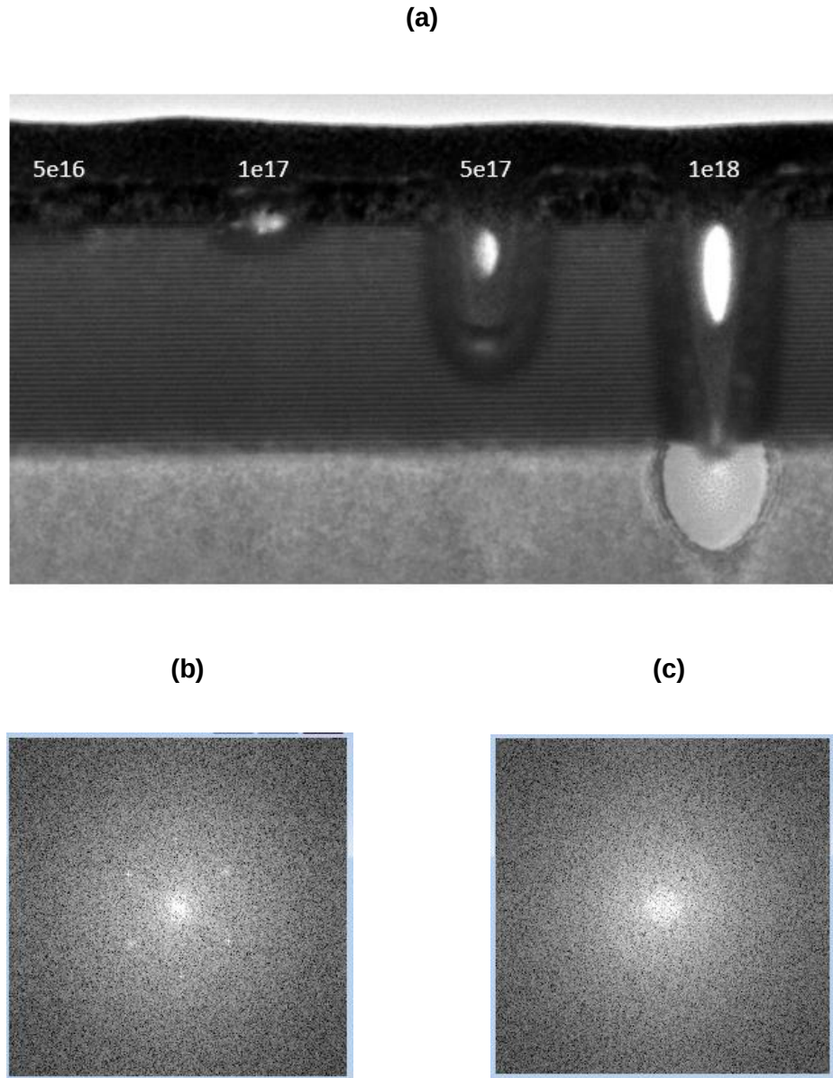
Figure 2.31. For a \text{Ne}^+ beam energy of 22.5 keV, the exposures from 5 \times 10^{16} to 1 \times 10^{18} \text{ Ne}^+/\text{cm}^2 . In b) below, the diffraction pattern for the silicon substrate, and in c) the same but within the region affected by the beam after a 1 \times 10^{18} \text{ Ne}^+/\text{cm}^2 on the structure.
