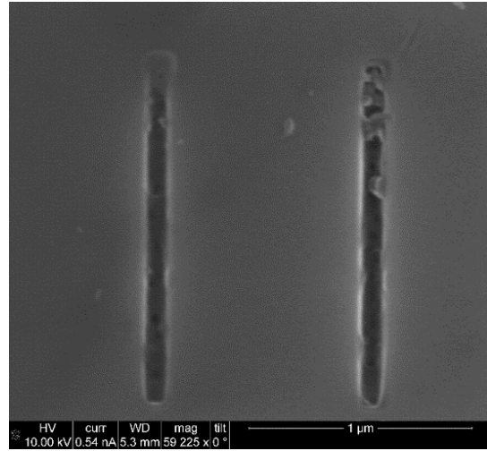
Figure 2.16. Top Ne-HIM view of etched lines (a), and top SEM view for two etched lines (b).
