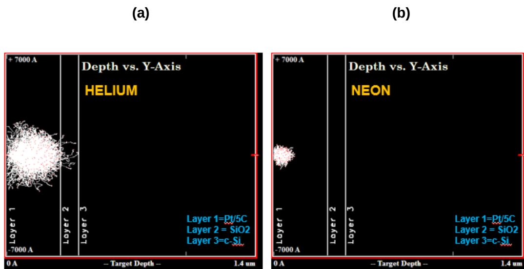
Figure 1.15. Interaction volumes for 1,000 ions of 30 keV helium (in a) and for neon (in b) in the Pt/C structure (300 nm). Layers 2 and 3 are SiO 2 (100 nm) and Si, respectively.
