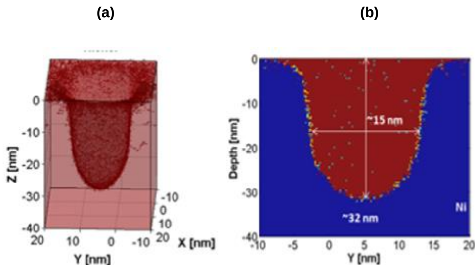
Figure 2.25. 3- (a) and 2-D (b) sputter profiles for \text{Ne}^+ in Ni at 30 keV and \sim 2 \times 10^{17} ions/cm 2 (using a 10nm x 10nm exposure area).
