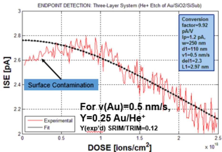
Figure 3.31. Experimental and fit ISE vs. Dose data for He + on Au/SiO 2 /Si.
