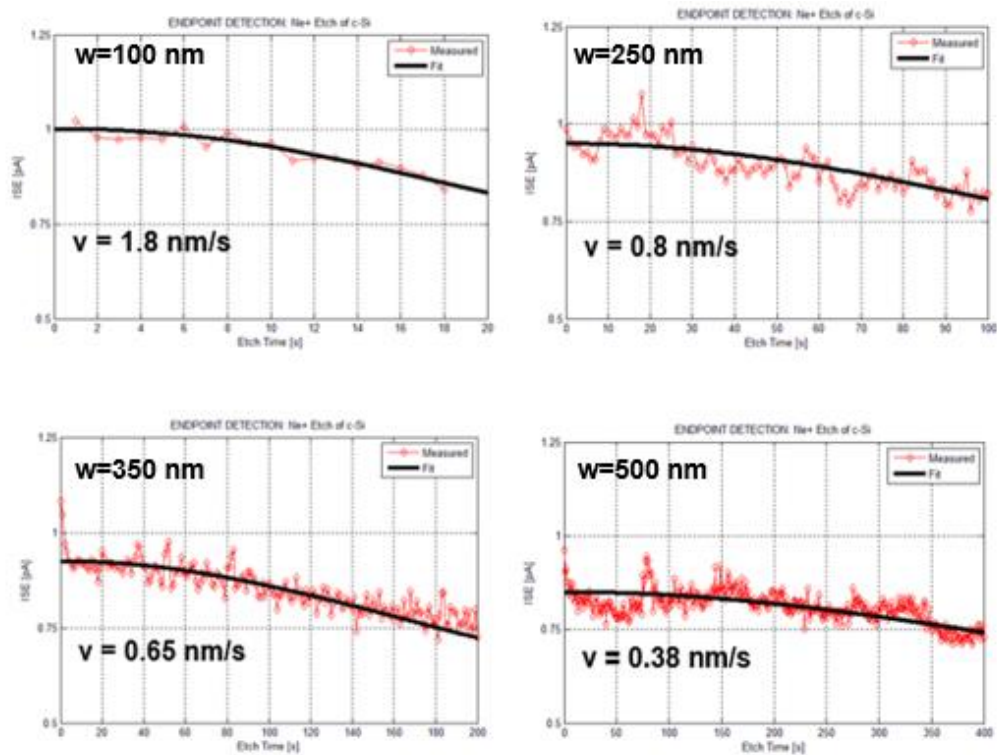
Figure 3.12. Actual measured data and fits for four (4) silicon box widths profiled at the same voltage (24 keV Ne + ), current (1.0 pA) and final dose ( 1 \times 10^{18} ions/cm 2 ).
