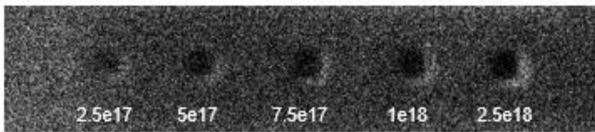
Figure 3.34. NIM image for a dose study of neon in a copper structure (Cu/SiO 2 /Si).
