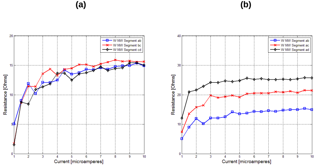
Figure 1.11. On left (a), resistances measured for equal length segments of W NW via 4-pt probing and between each test pad at 10 \mu s. On right (b), resistances measured for increasing length segments of W NW via 4-pt probing also at 10 \mu A.
