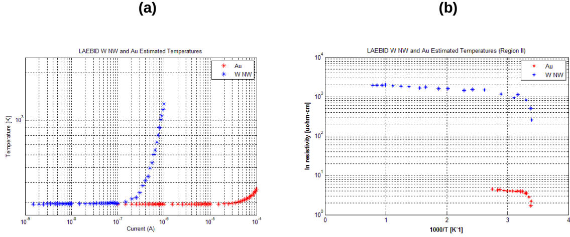
Figure 1.27. On left (a), the estimated temperature as a function of the applied current, and on the right (b), the estimated resistivity dependence on temperature. Both, the W NW (in blue) and Au reference (in red) shown.
