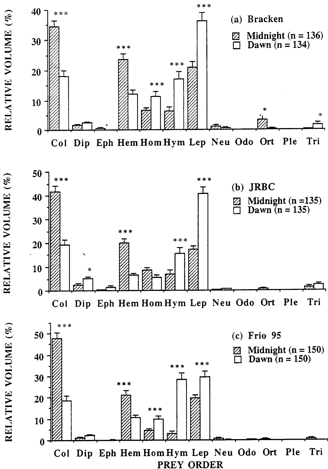
Figure 2.4 (see the previous page for the legend).
