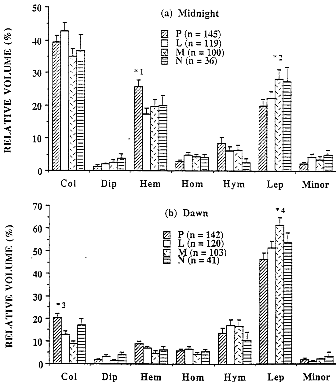
Figure 2.7. Dietary differences between pregnant (P), lactating (L), non-reproductive (N) females, and males (M) in (a) midnight and (b) dawn samples, during late May-mid July. Asterisks indicate prey orders where significant differences occurred. The significance level of all paired comparisons was 0.05. *1: F = 3.59 , P < 0.05 , P - L = 8.3 , PLSD = 5.2 , P - M = 5.93 , PLSD = 5.46 ; *2: F = 2.58 , P < 0.05 , M - P = 8.4 , PLSD = 6.43 ; *3: F = 8.77 , P < 0.001 , P - L = 7.44 , PLSD = 4.38 , P - M = 11.34 , PLSD = 4.57 ; *4: F = 3.96 , P < 0.01 , M - P = 14.75 , PLSD = 8.47 , M - L = 9.71 , PLSD = 8.79 .
