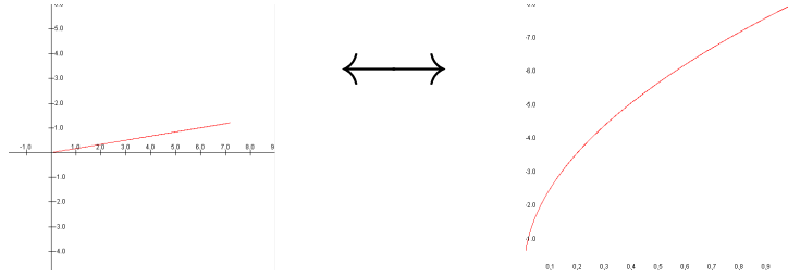
Figure 2: \lambda(t) = 8\sqrt{t} is shown on the right. The corresponding Loewner curve is shown on the left.
