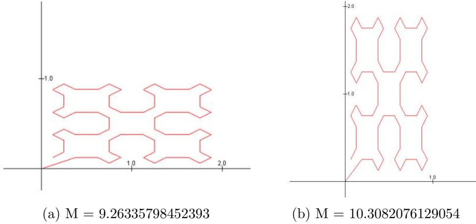
Figure 13: Lip(1/2) Norms when x and y are multiplied by 2
