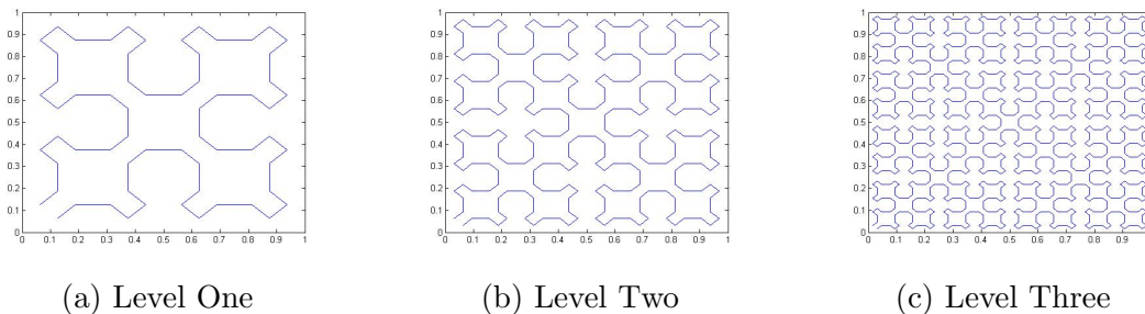
Figure 6: Sierpiński curve created in MATLAB
