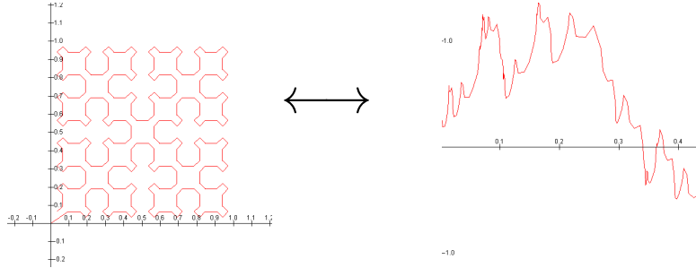
Figure 8: Level Two Sierpiński curve and corresponding driving function
