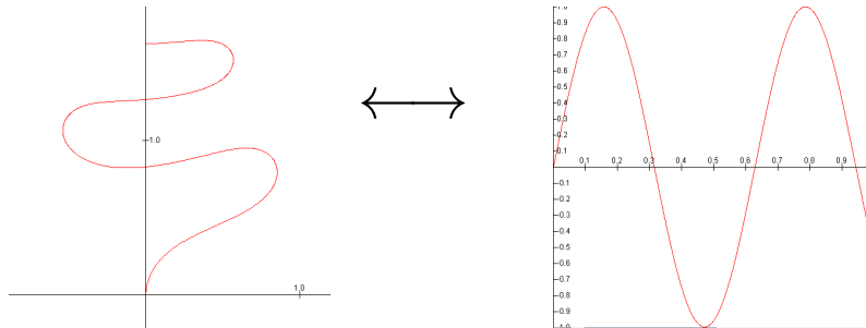
Figure 1: \lambda(t) = \sin(10t) is shown on the right. The corresponding Loewner curve is shown on the left.
