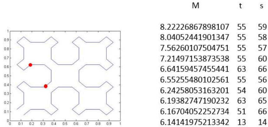
Figure 11: Top 10 M Values for Level One of the Sierpiński Curve
