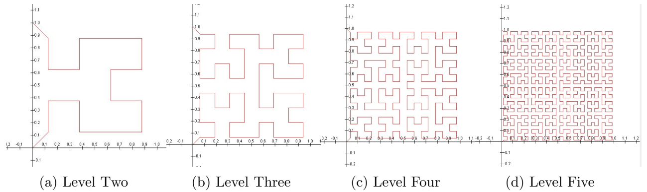
Figure 7: Plots of Hilbert Curve
