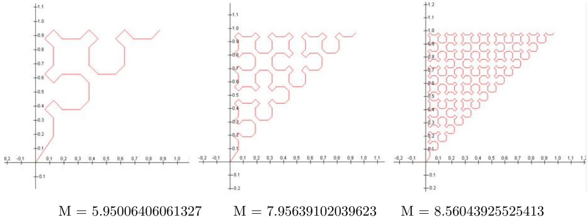
Figure 12: Lip(1/2) Norms of half of the Sierpiński curve generated in reverse
