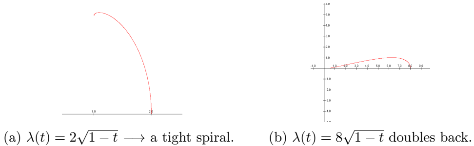
Figure 3: The different results generated using \lambda(t) = c\sqrt{1-t} .
