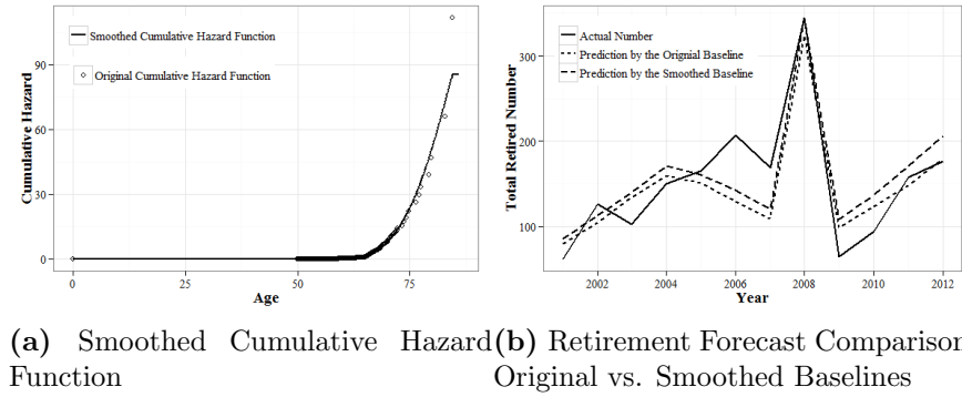
Figure 3.19: Retirement Model's Smoothed Baseline Plot and Forecast Comparison by Original and Smoothed Baselines
