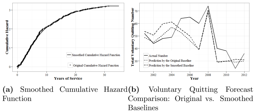
Figure 3.20: Voluntary Quitting Model Smoothed Baseline Plot and Forecast Comparison by Original and Smoothed Baselines
