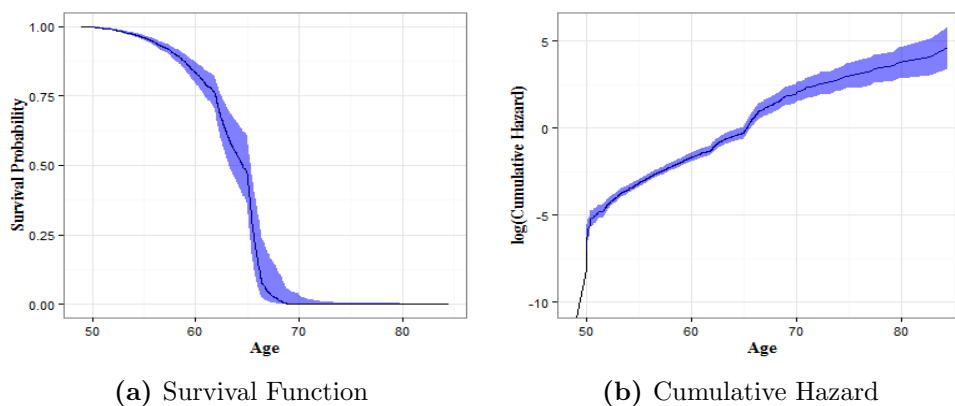
Figure 3.9: Baselines with 95% Confidence Intervals
