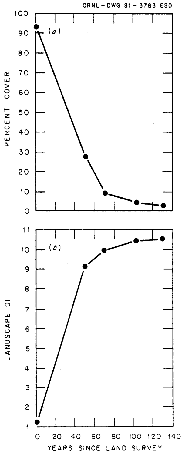
Fig. 17. Changes in two landscape parameters of Cadiz township, Green County, Wisconsin after the General Land Office Survey of 1831.
