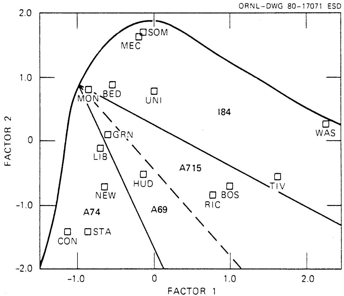
Fig. 10. Overlay of soil type on the basic site ordination of Ohio landscapes.
