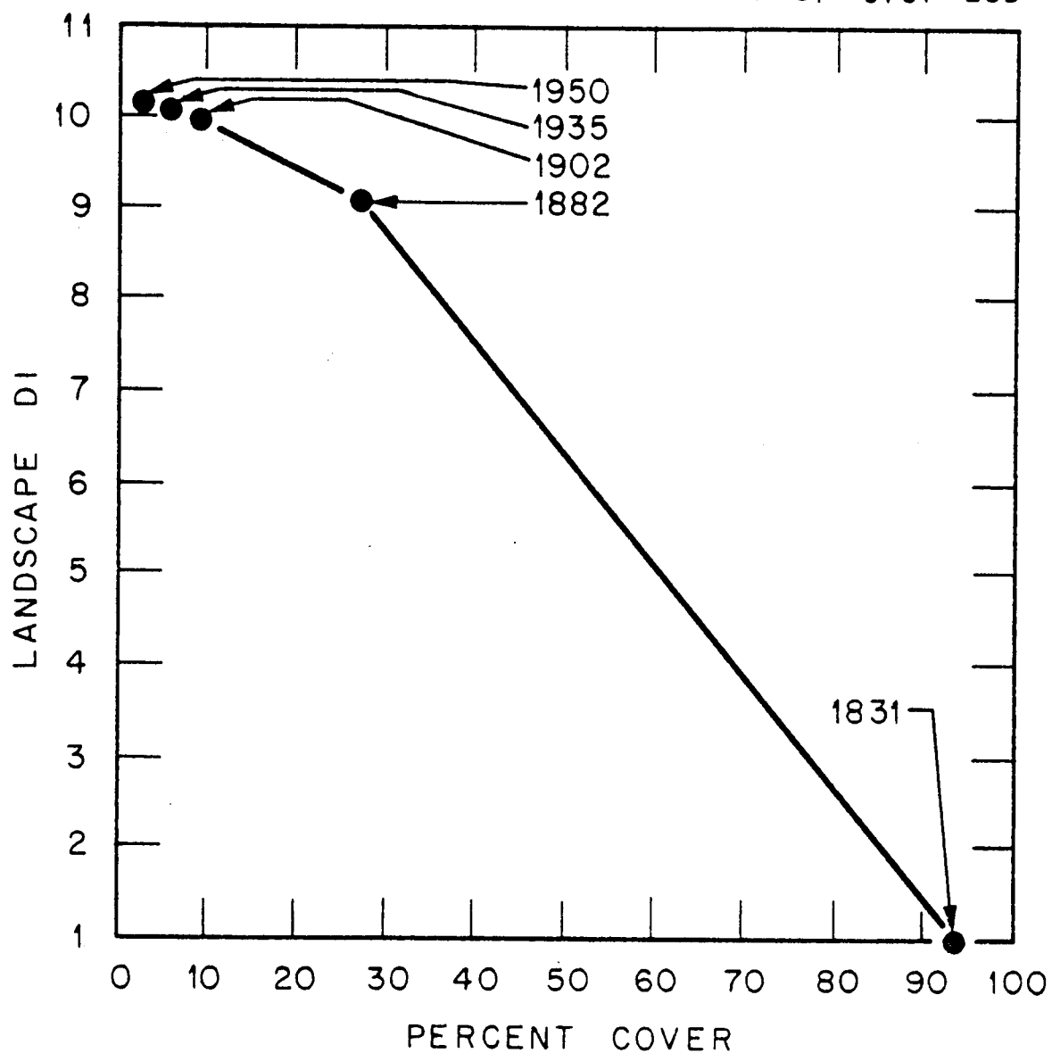
Fig. 18. Changes in the forest pattern of Cadiz township, Green County, Wisconsin portrayed as a vector in a two dimensional space defined by the variables percent cover and landscape DI.
