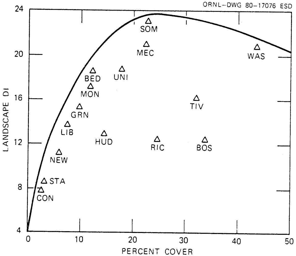
Fig. 8. Second alternative site ordination of 15 Ohio landscapes. Axes are the variables percent cover and landscape DI. The solid line delimits the region where landscapes are possible. The existence of landscapes in the upper right and upper left corners is unlikely.
