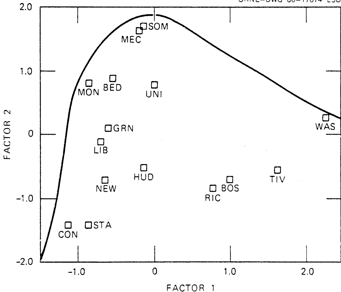
Fig. 6. Basic site ordination of 15 Ohio landscapes. Axes are derived from a factor analysis using seven continuous variables relating to forest island pattern. The solid line delimits the region where landscapes are possible. The existence of landscapes in the upper right and upper left corners is unlikely.
