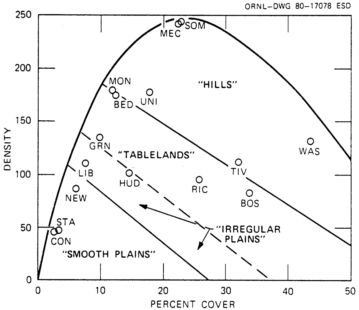
Fig. 14. Overlay of land surface form classes on the first alternative site ordination of Ohio landscapes. Axes are the variables percent cover and island density.
