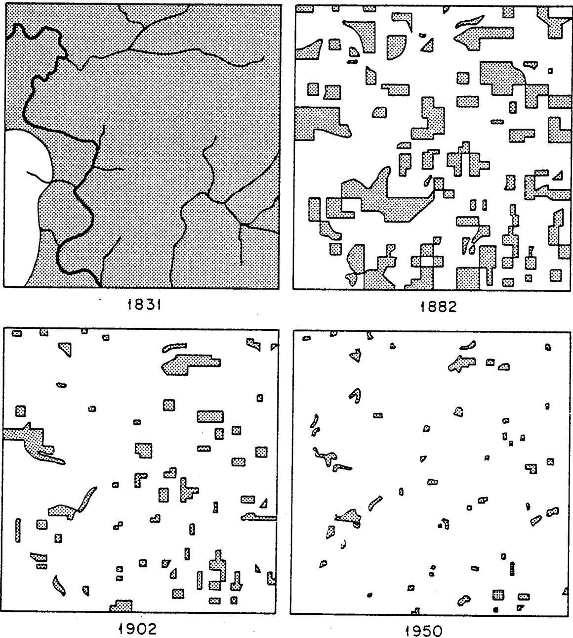
Fig. 1. Changes in wooded area of Cadiz Township, Green County, Wisconsin (89 54' W., 43 30' N.), during the period of European settlement. The shaded areas represent the land remaining in or reverting to forest in 1882, 1902, and 1950.
