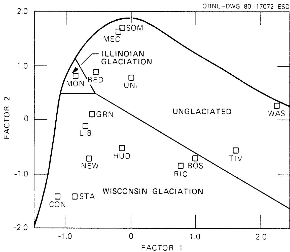
Fig. 11. Overlay of glacial history on the basic site ordination of Ohio landscapes.
