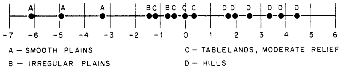
Fig. 16. One dimensional site ordination of 15 Ohio landscapes. Axes are derived from a discriminant analysis based on seven landscape variables and using land form as the discriminant criterion.
