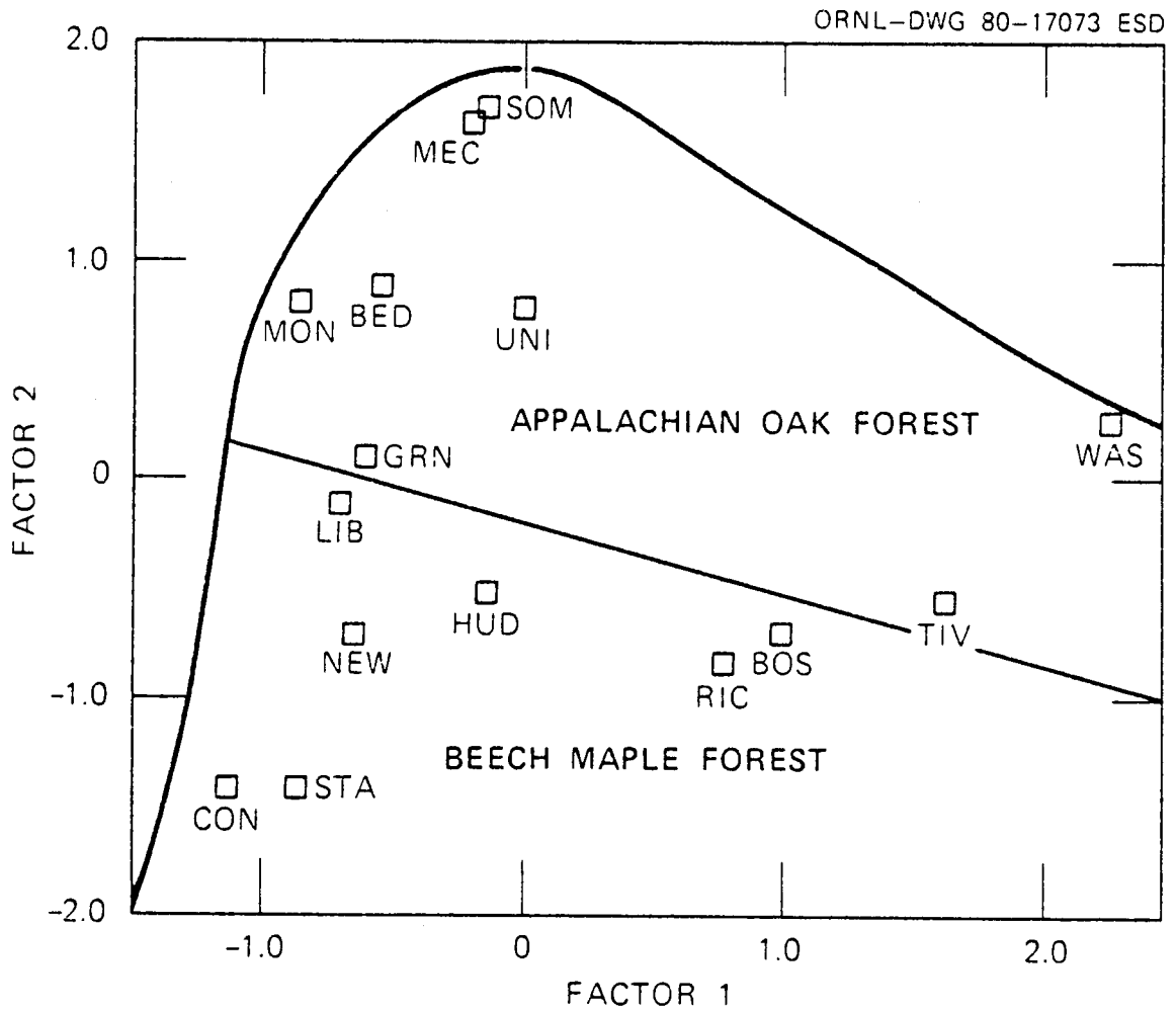
Fig. 12. Overlay of potential natural vegetation types on the basic site ordination of Ohio landscapes.
