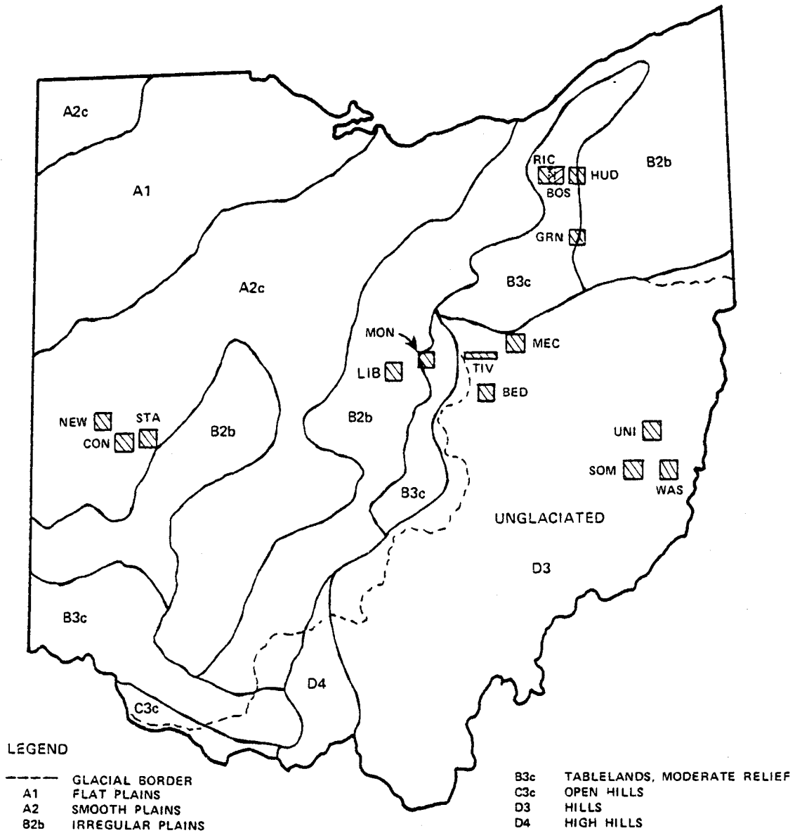
Fig. 2. Distribution of study areas in Ohio with respect to land surface form and glacial history. Study areas are assigned three letter identifiers.
