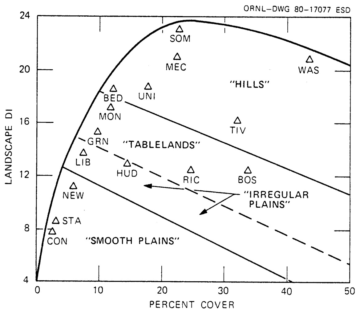
Fig. 15. Overlay of land surface form classes on the second alternative site ordination of Ohio landscapes. Axes are the variables percent cover and landscape DI.
