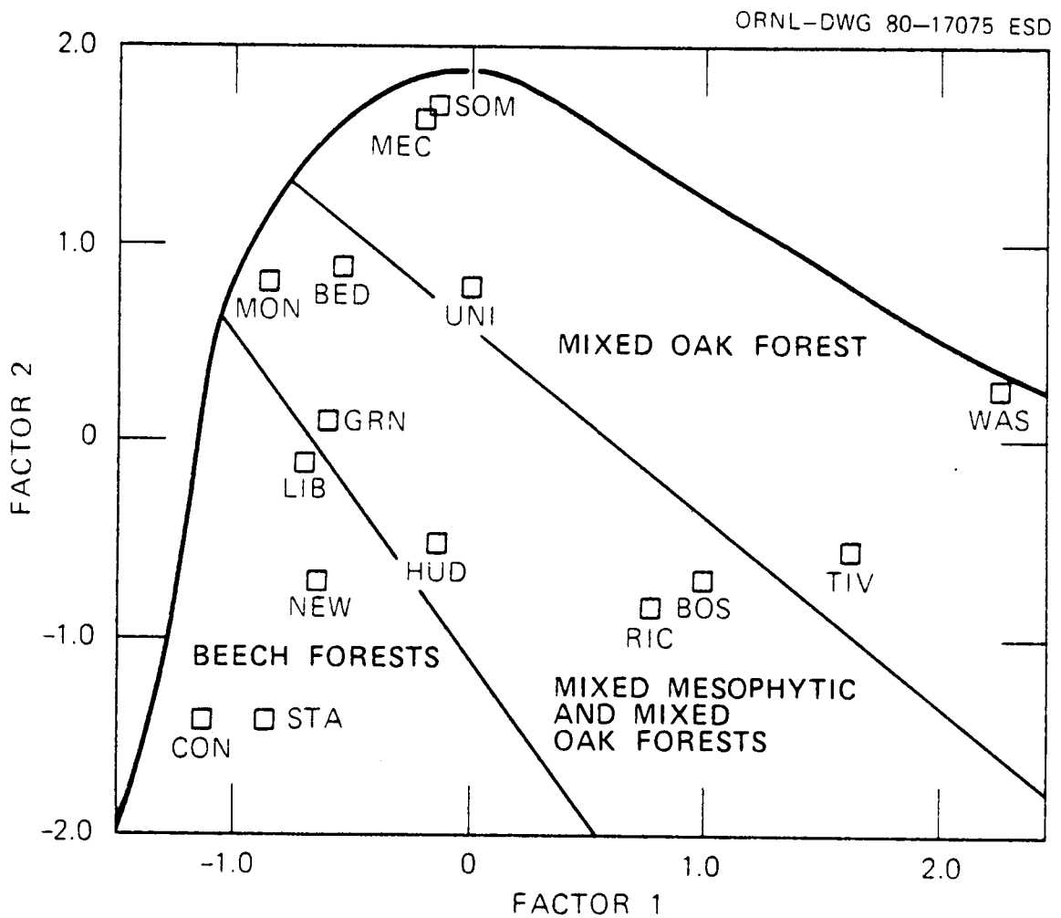
Fig. 13. Overlay of original forest types on the basic site ordination of Ohio landscapes.
