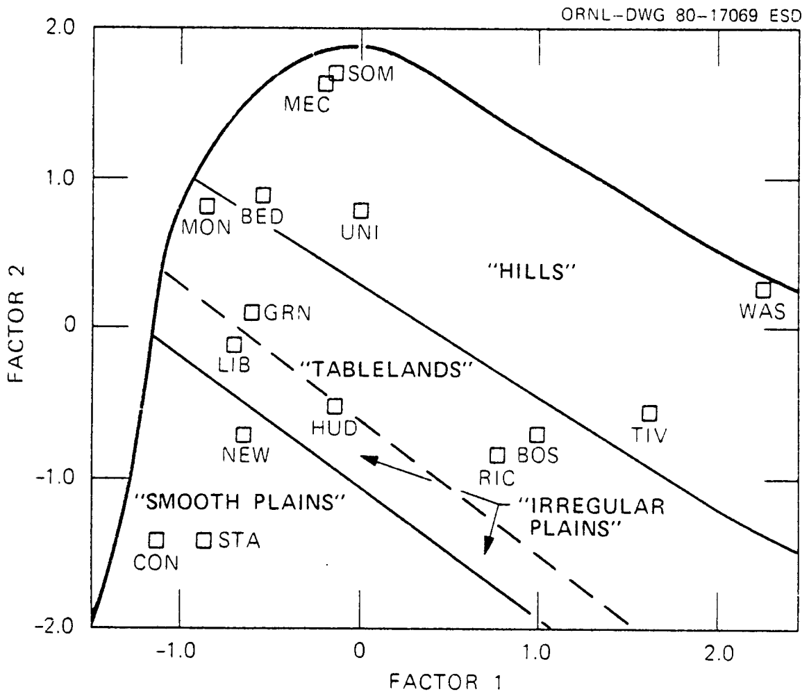
Fig. 9. Overlay of land surface form classes on the basic site ordination of Ohio landscapes.
