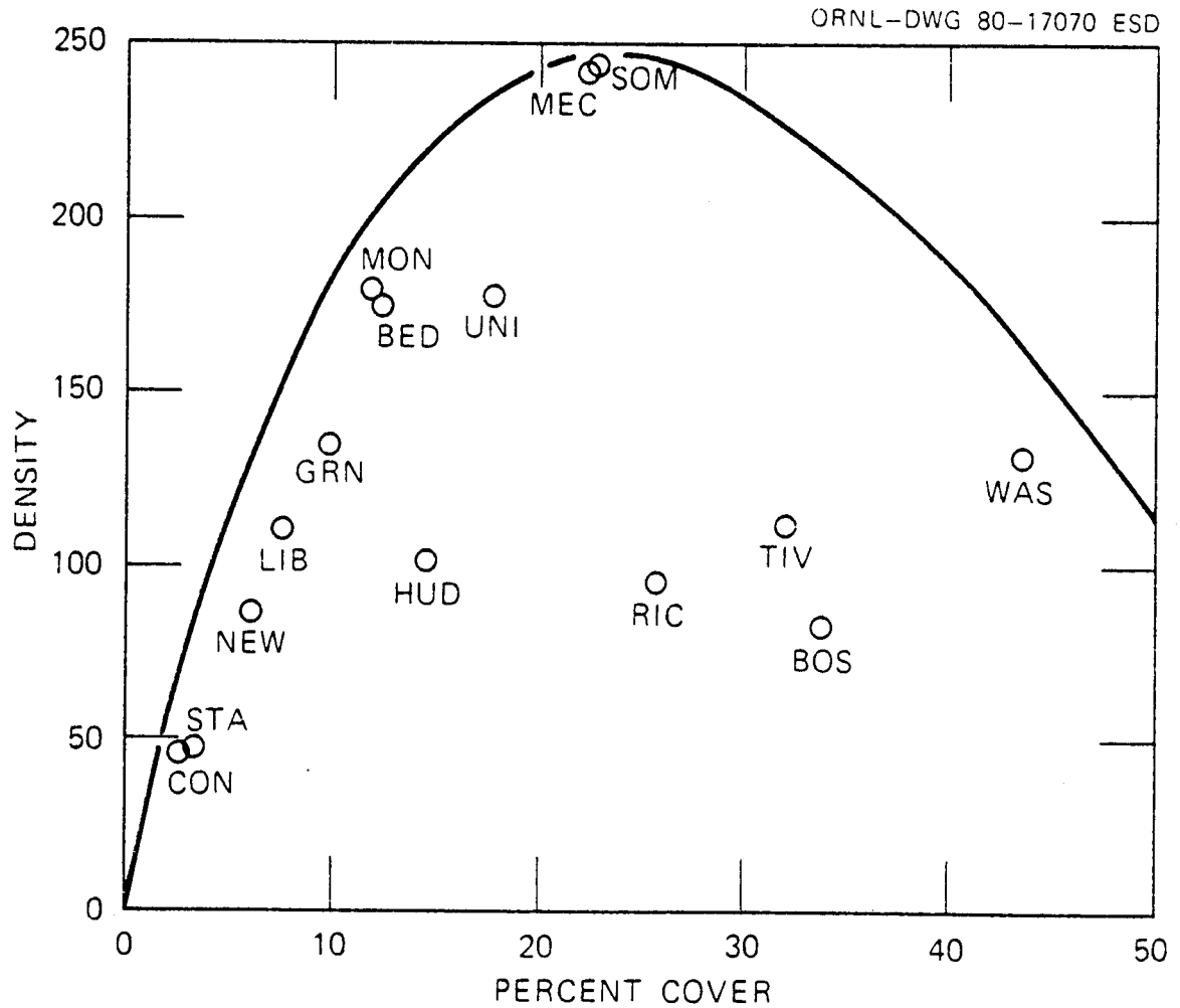
Fig. 7. First alternative site ordination of 15 Ohio landscapes. Axes are the variables percent cover and island density. The solid line delimits the region where landscapes are possible. The existence of landscapes in the upper right and upper left corners is unlikely.
