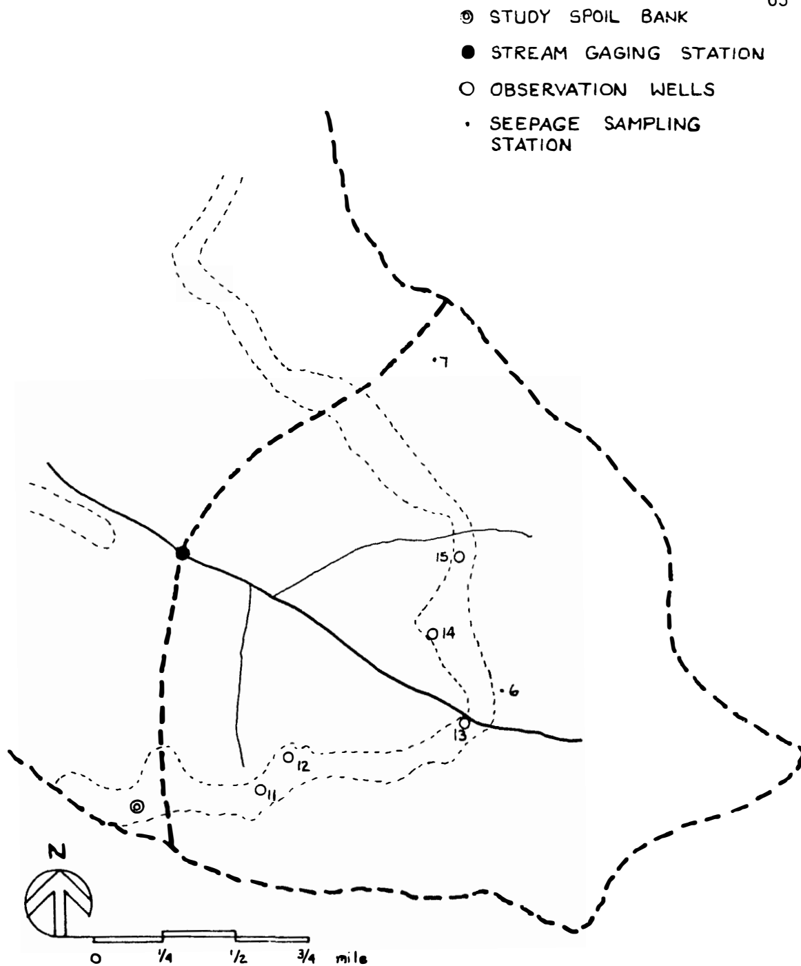
Figure 11. Bills Branch Study Basin with Mining Disturbance and Locations of Study Spoil Bank, Stream Gaging Station, Observation Wells, and Seepage Sampling Points.
