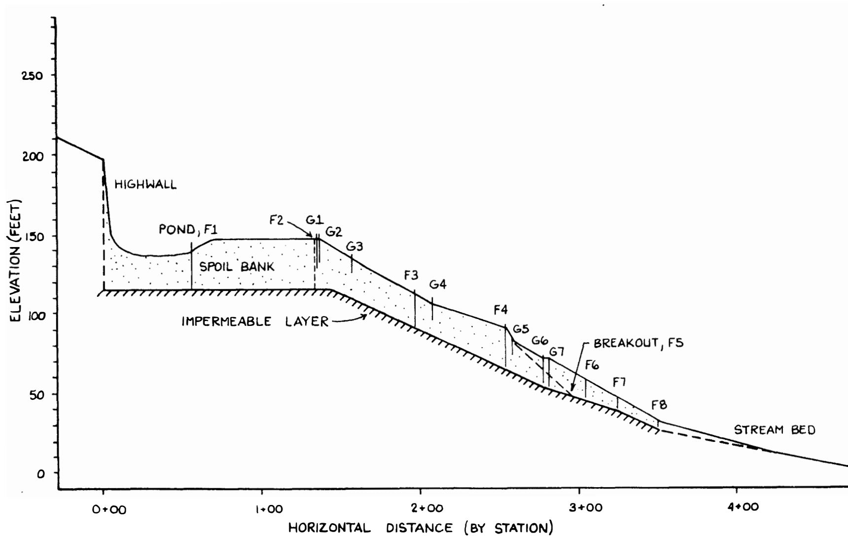
Figure 12. Profile, Indian Fork Study Spoil Bank.
