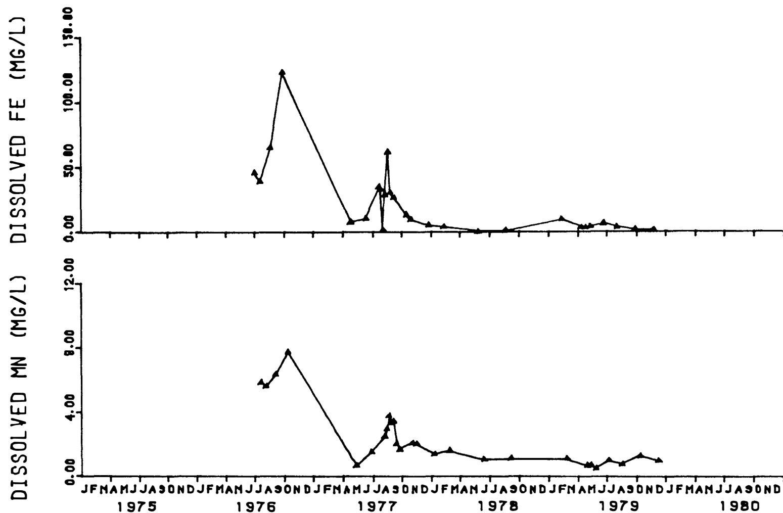
Figure 26. Response of Dissolved Iron and Manganese with Time at the Indian Fork F3 Well.
