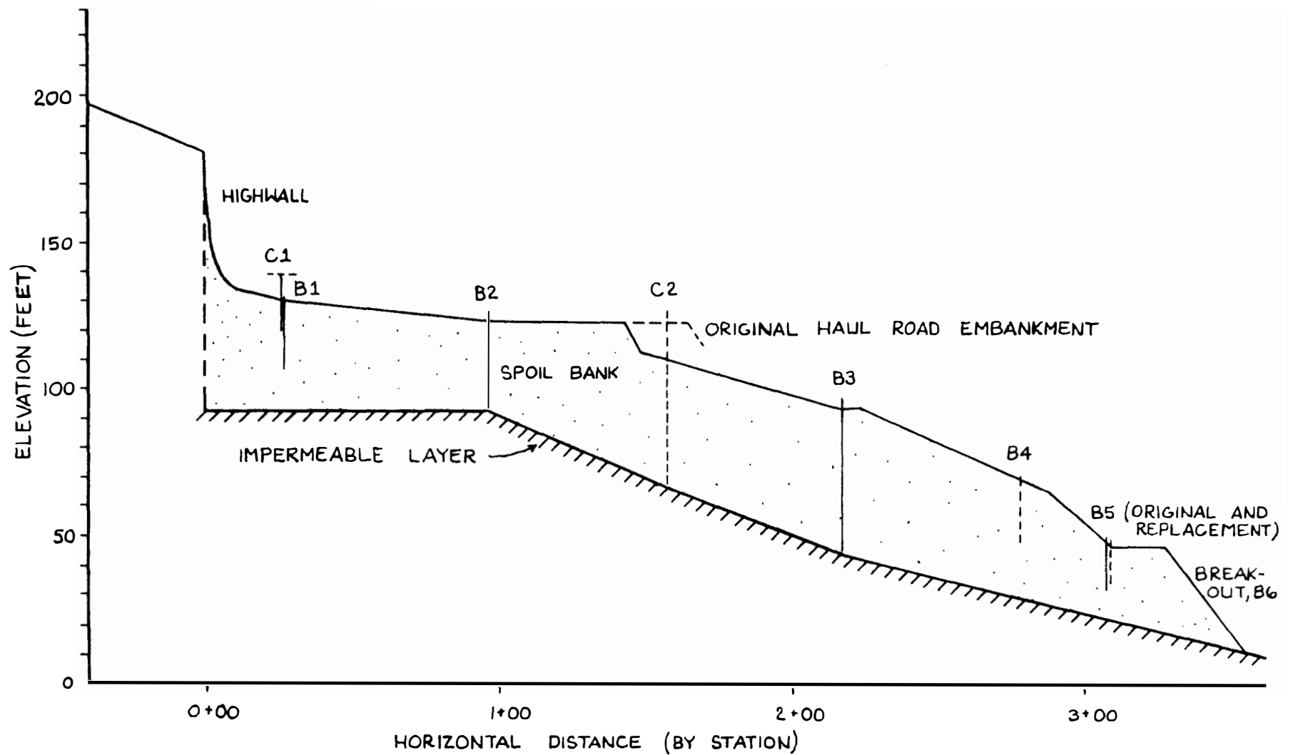
Figure 14. Profile, Bills Branch Study Spoil Bank.
