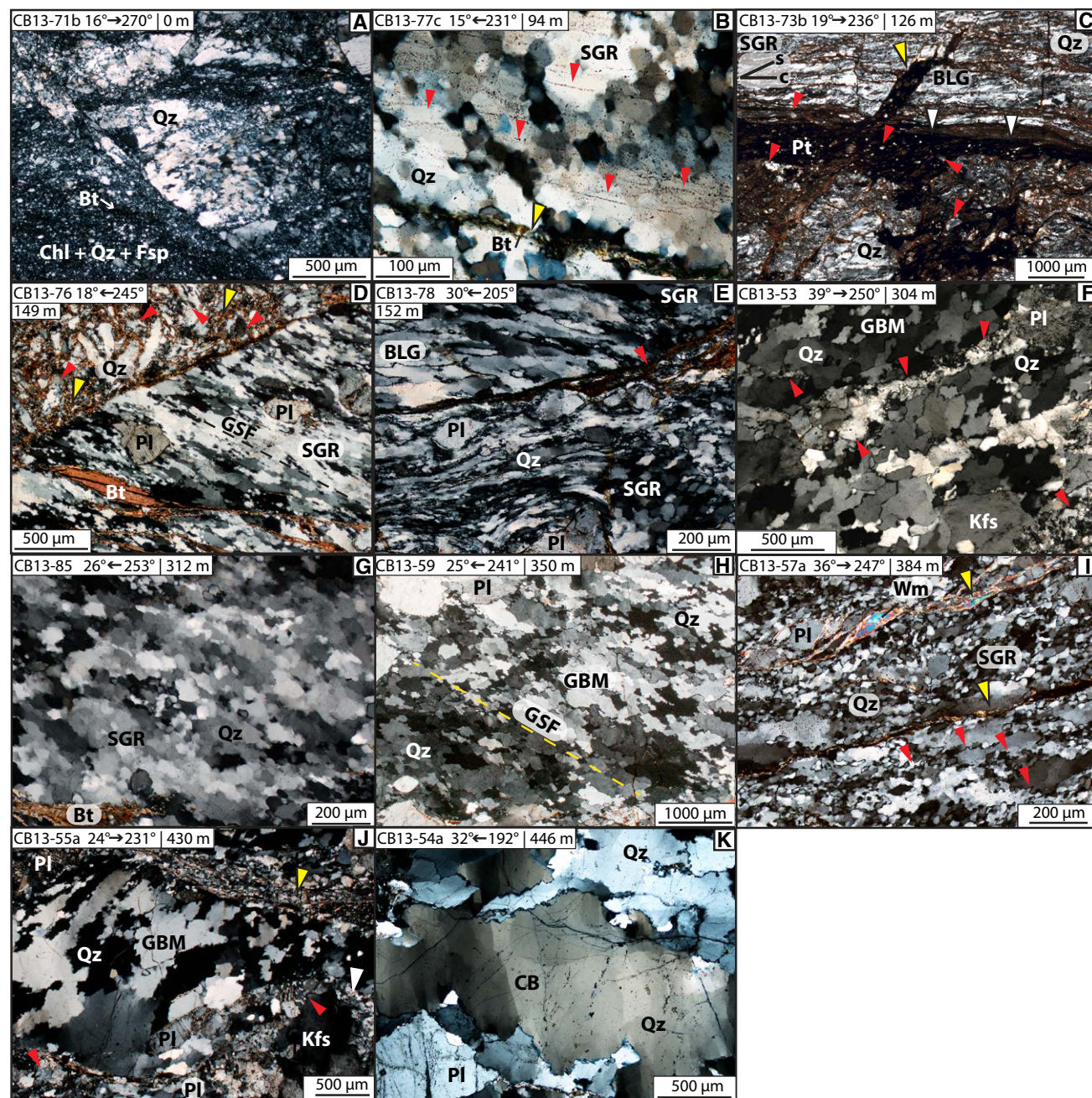
Figure 6. Cross-polarized light photomicrographs of quartz microstructures. Labels denote trend and plunge of lineation, with arrow pointing down-plunge and structural depth below the Cordillera Blanca detachment (in meters); arrowhead indicators are specified below as (color). Bt—biotite; Chl—chlorite; Fsp—feldspar (undifferentiated); Kfs—K-feldspar; Pl—plagioclase; Qz—quartz; Wm—white mica. Quartz recrystallization microstructures: BLG—bulging; SGR—subgrain rotation; GBM—grain boundary migration. (A) Microfaults truncating mylonitic foliation at high angles. Mylonitic fabric records SGR and BLG recrystallization in quartz. (B) Quartz SGR overprinted by fluid inclusion planes (red) oriented subparallel to shear bands (yellow). (C) Pseudotachylyte injection vein (yellow) and pseudotachylyte layer oriented parallel to mylonitic foliation (white), containing deformed mylonitic clasts and plagioclase feldspar grains (red). Relative orientation of mylonitic S-C fabric shown at upper left. (D) Quartz SGR with grain-shape fabric (GSF), truncated by cataclasis with biotite-rich matrix (yellow) and mylonitic clasts (red). (E) BLG and SGR recrystallization in quartz and SGR in quartz affected by nearby feldspar porphyroclasts (lower part of image). Biotite-rich shear band is present (red). (F) GBM in quartz domains adjacent to recrystallized feldspar. Some quartz grains are pinned at feldspar-quartz grain boundaries (red). (G) SGR in quartz. (H) GSF in quartz exhibiting GBM recrystallization microstructure. (I) BLG (red) and SGR in quartz. White mica forms fish and shear bands (yellow). (J) Quartz exhibiting GBM, deflecting into fine-grained quartz-feldspar-mica shear bands (yellow). Myrmekite (red) grows into K-feldspar porphyroclasts and within matrix. Recrystallized feldspar occurs along plagioclase and K-feldspar porphyroclast edges (white). (K) Orthogonal subgrain boundaries forming chessboard extinction (CB) in quartz.
