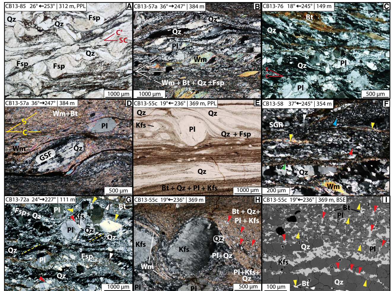
Figure 8. Photomicrographs of microfabrics. Images are cross-polarized light (XPL) unless otherwise noted. Labels denote trend and plunge of lineation, with arrow pointing down-plunge and structural depth below the Cordillera Blanca detachment (in meters); arrowhead indicators are specified below as (color). Bt—biotite; Fsp—feldspar (undifferentiated); Kfs—K-feldspar; Pl—plagioclase; Qz—quartz; Wm—white mica. (A) Plane polarized light (PPL) image of type I S-C mylonite. S-surfaces anastomose in and out of C-surfaces. C' bands are defined by biotite and finely recrystallized quartz and feldspar. (B) Type I S-C mylonite. S-surfaces defined by mica fish and quartz anastomose into C-surfaces. (C) Type II S-C mylonite. S-surfaces are defined by biotite fish fabric and quartz grain-shape fabric (GSF). Biotite tails define C-surfaces. (D) White mica + biotite shear bands deflecting around recrystallized quartz and plagioclase porphyroclasts. GSF in quartz porphyroclast is aligned with S-plane defined by micas. (E) PPL image of banded mylonite with biotite-rich and biotite-poor, quartz-rich layers. (F) Compositionally banded mylonite with discontinuous mono- and polyphase layers. Monophase layers consist of quartz (white) or white mica (yellow); polyphase layers consist of quartz + plagioclase + K-feldspar (blue), K-feldspar + plagioclase (red), or white mica + quartz + plagioclase + K-feldspar (green). SGR—subgrain rotation. (G) Banded mylonite with continuous quartz layers and feldspar + quartz ± biotite (white) layers deflecting around fractured (red) and partially recrystallized (yellow) plagioclase porphyroclasts. Quartz exhibits oblique GSF (yellow dashed lines). (H) Recrystallization along rim of K-feldspar and plagioclase grains and within tails. Tails disaggregate into fine-grained biotite + quartz + plagioclase + K-feldspar matrix (red). (I) Backscattered electron (BSE) image of intermixed fine-grained polyphase matrix. K-feldspar occupies dilatant sites between plagioclase and quartz grains (red). Biotite and K-feldspar occupy grain boundaries and triple junctions (yellow). Black is result of holes and/or poor polish.
