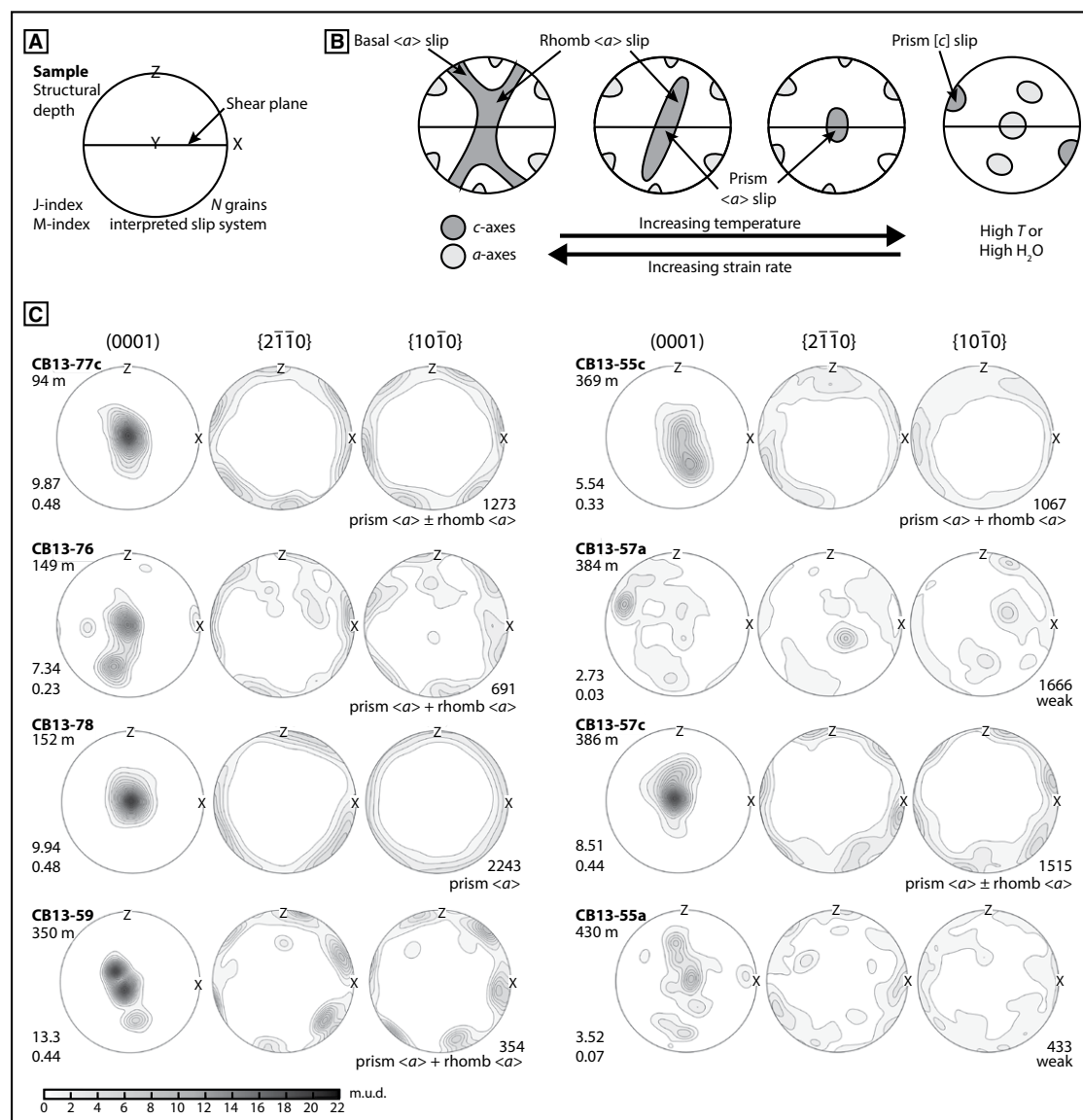
Figure 9. Quartz crystallographic preferred orientations (CPOs). (A) Orientation of quartz CPO pole figures relative to shear plane and X - Z thin section, with key to labels for panel C. J-index (Bunge, 1982) and M-index (Skemer et al., 2005) indicate fabric strength. N —number of grains. (B) Schematic c - and a -axis pole figures of quartz CPOs for different quartz slip systems with changing temperature ( T ), strain rate, and H_2O conditions (after Passchier and Trouw, 2005). (C) Equal-area lower-hemisphere pole figures of quartz c - (0001), a - \{2\bar{1}\bar{1}0\} , and prism-normal- \{10\bar{1}0\} axes. All plots are one point per grain, contoured at 1 m.u.d. (multiple of uniform distribution) intervals, using a 7.5^\circ half-width. Orientation of figures relative to X - Z plane, and labels are as in A.
