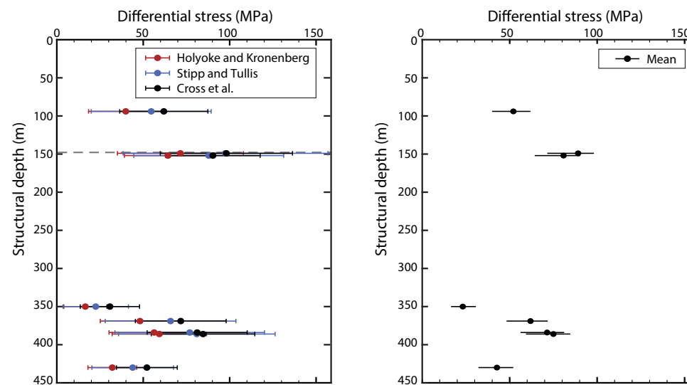
Figure 10. Differential stress estimates with increasing depth below the Cordillera Blanca detachment. (A) Differential stress estimates for Stipp and Tullis (2003), Holyoke and Kronenberg (2010), and Cross et al. (2017b) piezometers, shown relative to structurally deepest observed sample containing throughgoing brittle overprint (gray dashed line). Error bars are standard deviation on root mean square grain size propagated through each piezometer. (B) Mean differential stress of the three piezometers. Error bars are maximum range of stress estimates from the three calibrations.
