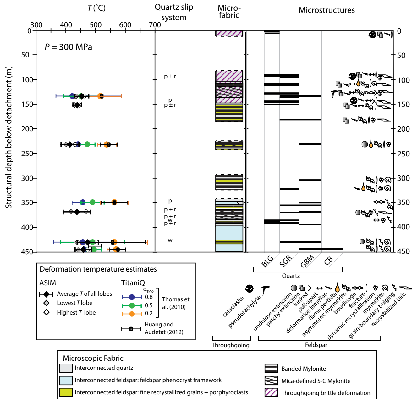
Figure 7. Summary figure of microstructural analysis, geothermometry, and quartz crystallographic preferred orientation results at increasing structural depths below the Cordillera Blanca detachment. Quartz slip systems: p—prism \langle a \rangle ; r—rhomb \langle a \rangle ; w—weak. Deformation temperature ( T ) errors are as reported in Table 2. Error bars for average asymmetric strain-induced myrmekite (ASIM) temperatures do not include the \pm 50^{\circ}\text{C} error on the thermometer. P —pressure; TitaniQ—Ti-in-quartz thermometer; \alpha_{\text{TiO}_2} —Ti activity; BLG—bulging recrystallization; SGR—subgrain rotation recrystallization; GBM—grain-boundary migration recrystallization; CB—chessboard extinction.
