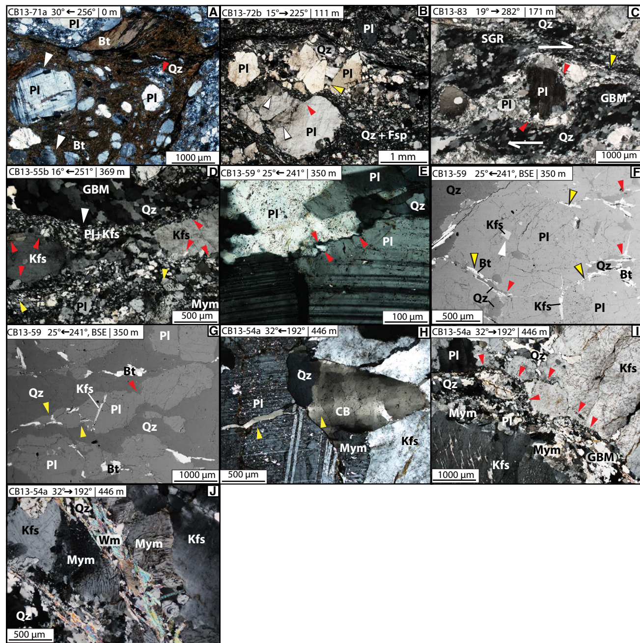
Figure 5. Representative images of feldspar microstructures. Images are cross-polarized light (XPL) photomicrographs unless otherwise noted. Labels denote trend and plunge of lineation, with arrow pointing down-plunge, and structural depth below the Cordillera Blanca detachment (in meters); arrowhead indicators are specified below as (color). Bt—biotite; Fsp—feldspar (undifferentiated); Kfs—K-feldspar; Mym—myrmekite; Pl—plagioclase; Qz—quartz; Wm—white mica. (A) Cataclasite including internally deformed plagioclase clasts (white) and dynamically recrystallized quartz (red) in biotite-rich (left) and biotite-poor (right) quartz-feldspar matrix. (B) Fractured plagioclase phenocrysts with small offset (red) and V-pull-apart structure with quartz infill (yellow). Patchy extinction is present near the offset fracture (white). (C) Dynamically recrystallized plagioclase (red), creating a core-mantle structure. Recrystallized feldspar tail deflects into a quartz-rich shear band; grain size of quartz and plagioclase decreases with deflection into the shear band (yellow). Subgrain rotation (SGR) and grain-boundary migration (GBM) recrystallization microstructures are present in the adjacent quartz domain. (D) Interconnected domain of recrystallized plagioclase and K-feldspar (white) adjacent to quartz domain exhibiting GBM recrystallization microstructure. K-feldspar porphyroclasts contain recrystallized tails and asymmetric strain-induced myrmekite (red). Myrmekite is also present in recrystallized plagioclase + K-feldspar matrix (yellow). (E) New grains formed by bulging recrystallization in plagioclase (red). (F) Back-scattered electron (BSE) image of interconnected plagioclase domain, biotite, and quartz along triple junctions (red). Biotite occupies grain boundaries between plagioclase phenocrysts (yellow). K-feldspar is hosted as inclusions within phenocrysts and as fracture fill (white). (G) BSE image of boudinaged plagioclase within quartz matrix (red). Biotite and quartz occupy dilatant sites in pinch-and-swells structure (yellow). (H) Wedge-shaped K-feldspar fracture filled with quartz exhibiting chessboard extinction (CB) that is continuous crystallographically with quartz within a plagioclase fracture (yellow). Image is rotated 90° counterclockwise from X-Z orientation. (I) Recrystallized plagioclase along K-feldspar grain boundaries and fractures (red). GBM recrystallization microstructure is present in interstitial quartz. (J) Myrmekite growth into K-feldspar, with white mica along the initial K-feldspar grain boundary.
