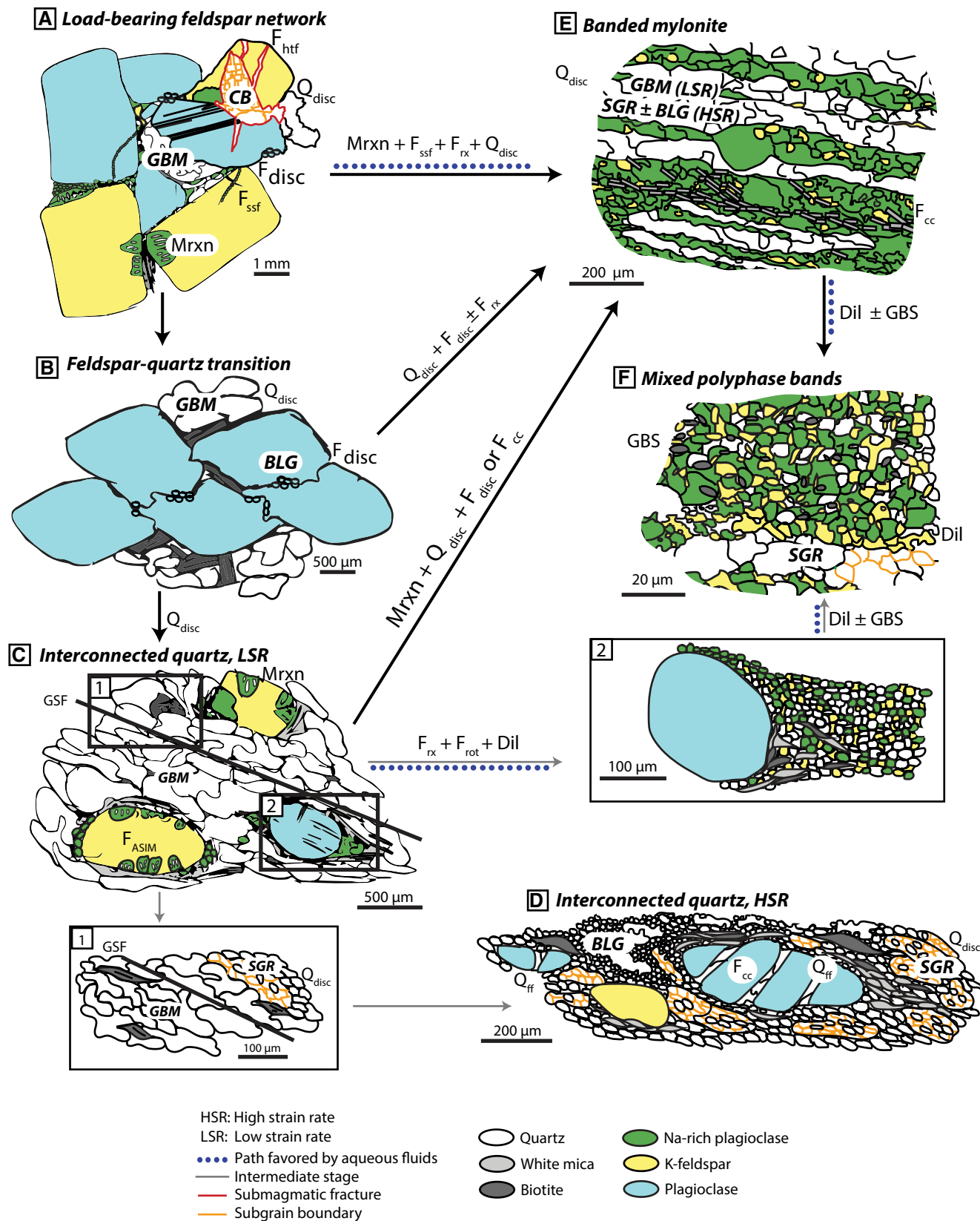
Figure 11. Schematic line drawings summarizing evolution of deformation mechanisms and related microstructures in the Cordillera Blanca shear zone. Arrows denote possible microstructural progressions, labeled with processes facilitating change in microstructure. Gray arrows denote transitional microstructures and processes. Abbreviations: F—feldspar, Q—quartz; htf—high-temperature fracturing; ssf—subsidiary fracturing; disc—dislocation creep; rot—rotation; rx—reaction to Na-rich plagioclase; ff—fracture fill; cc—cataclasis; Mrxn—myrmekite-forming reaction; CB—chessboard extinction; GBM—grain-boundary migration recrystallization; BLG—bulging recrystallization; SGR—subgrain rotation recrystallization; ASIM—asymmetric strain-induced myrmekite; GSF—grain-shape fabric; GBS—grain-boundary sliding; Dil—dilation. Scale bars are approximate. For clarity, grain sizes of quartz in D are depicted as slightly larger than actual. See text for details.
