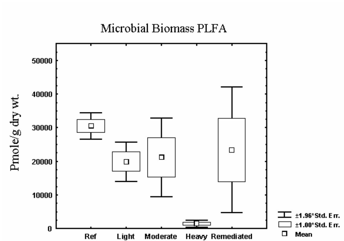
Figure 2-1. Microbial biomass PLFA. Samples were taken from four disturbance categories and areas undergoing remediation. P < 0.05 .
