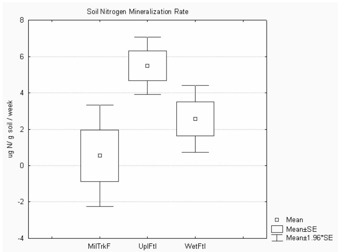
Figure 4-6. Soil nitrogen mineralization rate. Confidence level for mean: 95%. MilTrkF = frequent military tracked vehicles, UplFtl = upland forest infrequent foot traffic, and WetFtl = wetland infrequent foot traffic.
