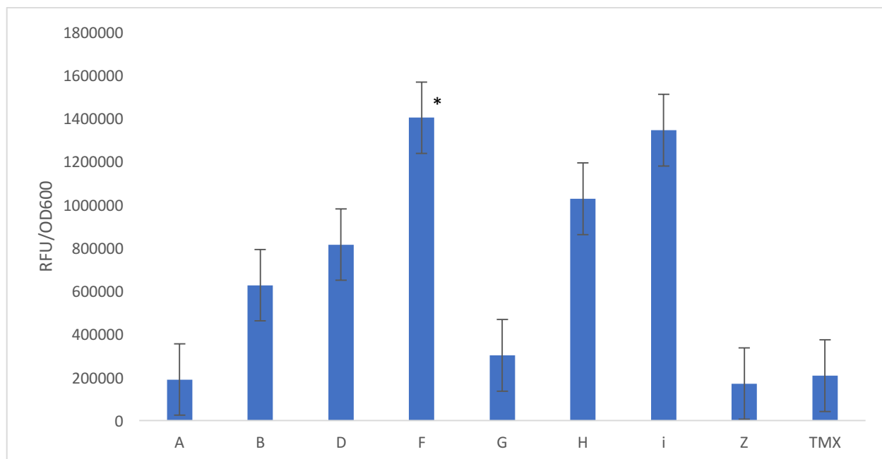
Figure 7. TMX's interaction in the high copy pUT18 with the Fab proteins in relative fluorescent units normalized with the OD 600 . *= p<0.05. Statistical significance relative to negative controls was determined using a T-test from the same assay plate.
