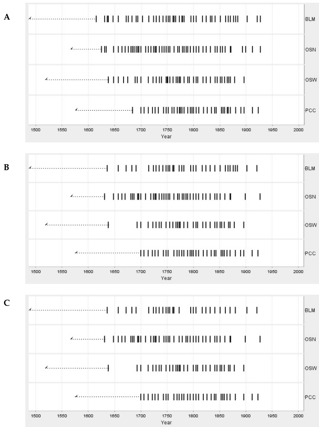
Figure 5.14 Composite filters for each site for (A) all fires (B) fires that scarred at least 10% of the samples, and (C) fires that scarred at least 25% of the samples. Vertical tic-marks represent fire years included in each filter
