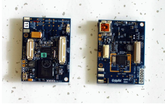
Figure 3-5: The Intel Mote 2 sensor platform
