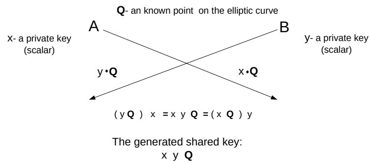
Figure 2-5: Generating a shared secret key using the Diffie Helman method over an elliptic curve
