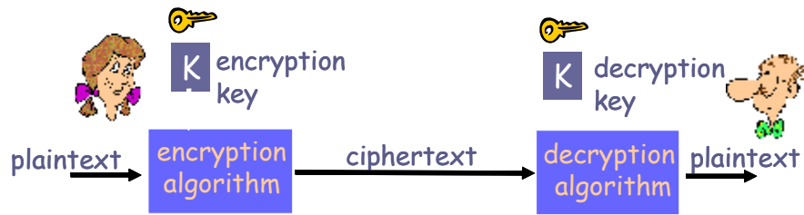
Figure 2-1: The foundations for symmetric cryptography: Alice is encrypting the plain message, and Bob is decrypting the ciphertext, while both use the same shared secret key (redrawn from [42])
