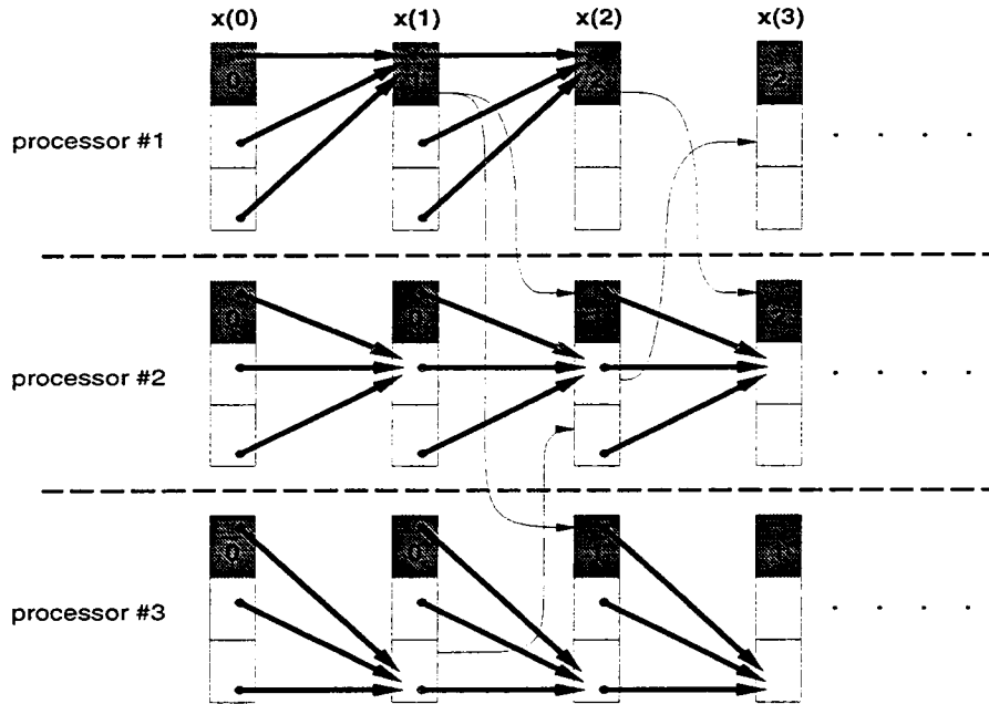
Figure 2.3: Asynchronous algorithm
