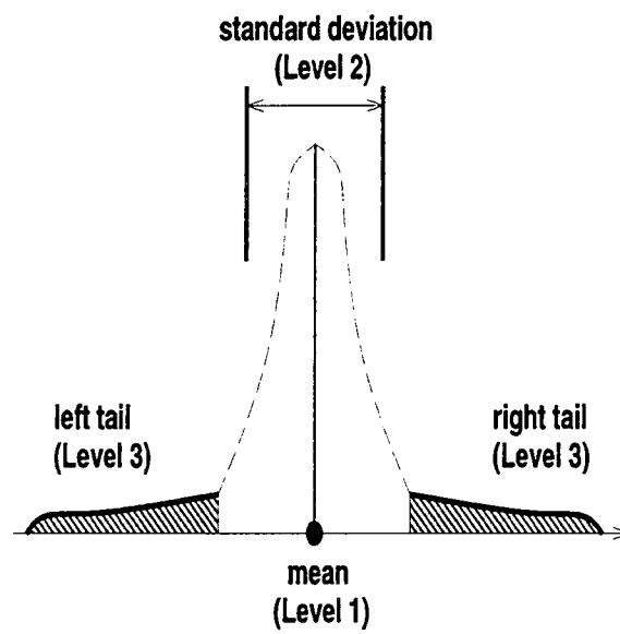
Figure 4.21: Probability distribution of \Theta
