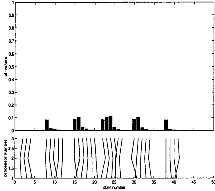
Figure 4.8: Stationary distribution and corresponding wavefront shapes for example 3
