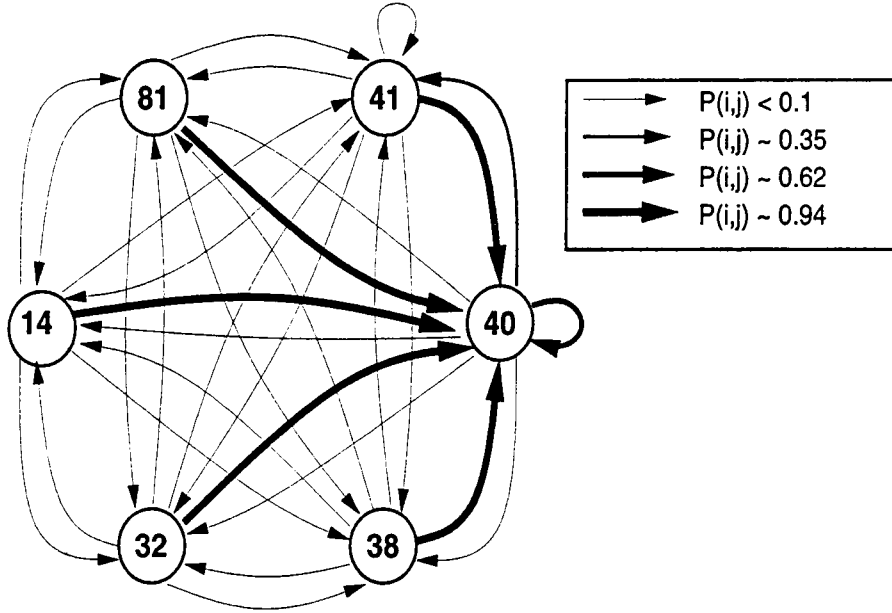
Figure 4.6: Wavefront Markov chain diagram for example 2
