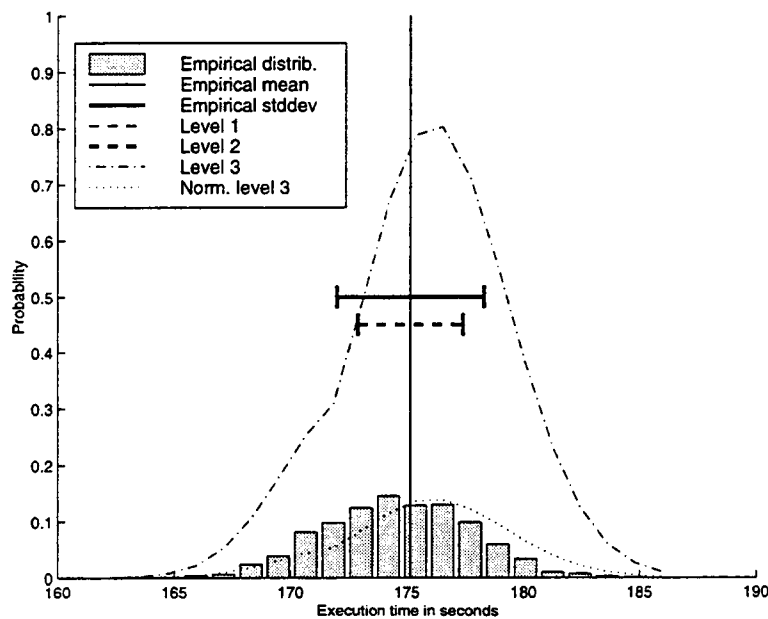
Figure 5.5: Adjusted curve for the first asynchronous implementation
