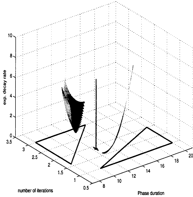
Figure 4.18: Example of Large Deviation Computation
