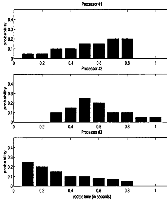
Figure 5.1: Update time distributions for the three processors
