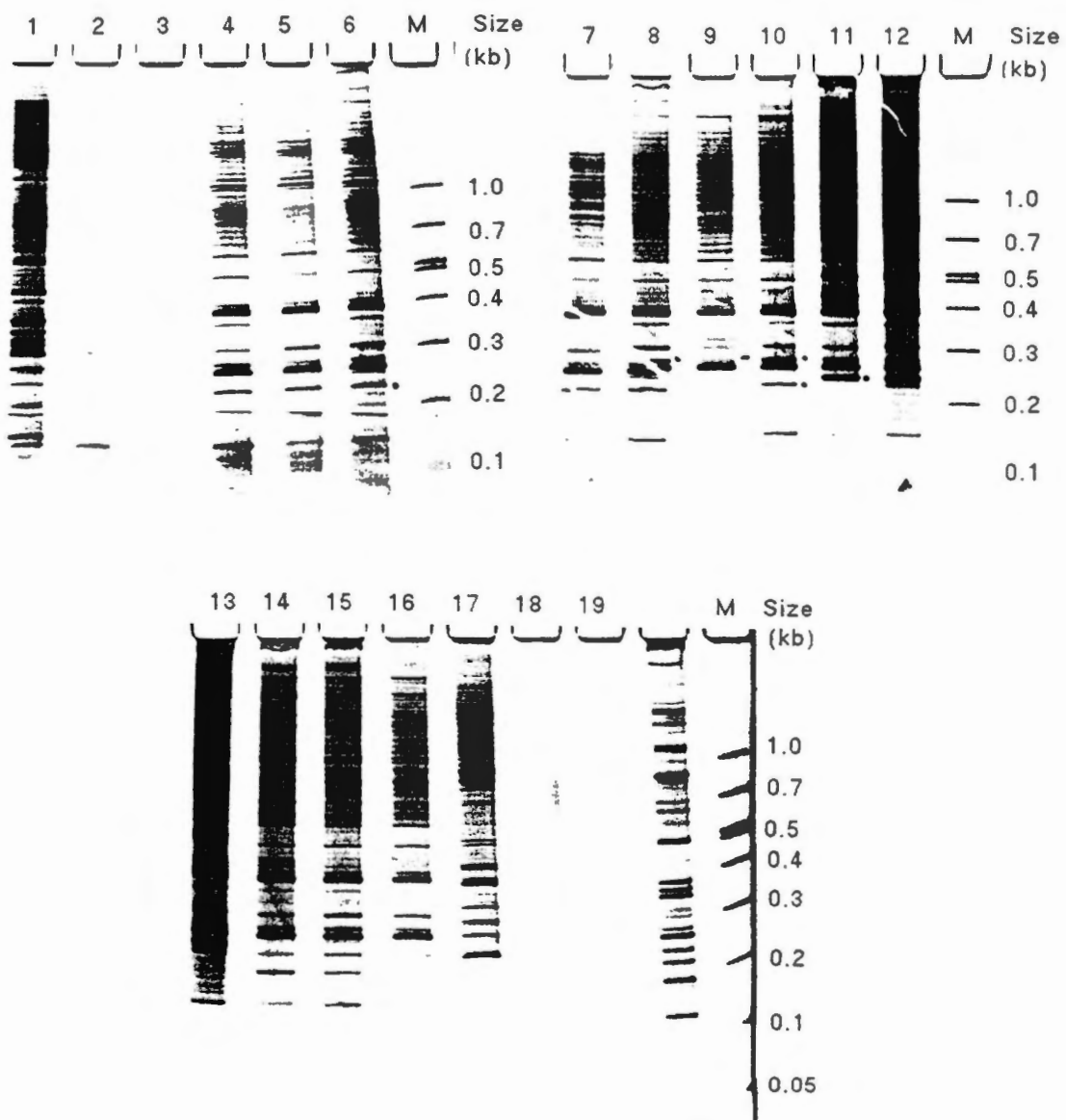
Figure 5-11. Silver-stained 10% polyacrylamide gels of DNA amplification fingerprinting using original DAF program a and OR30 (5'GTCCAAGA3') primer for 1-19 aphid samples. Molecular marker ranged from 0.1 to 1.0 kb is shown on the right.
