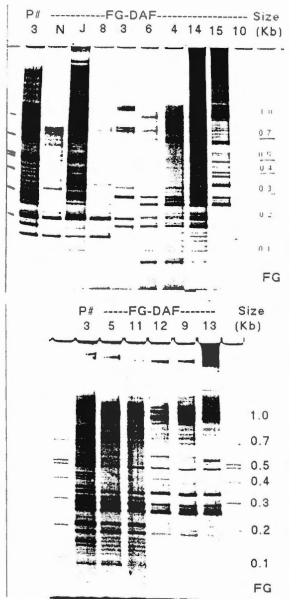
Figure 4-2. Polyacrylamide gels for 15 PCR programs using 8-4 (5'GTAACGCC3') primer for soybean DNA template cultivar Noir1. P# 3 (shown in both panels) and N-DAF are the original DAF program run in twin-block Ericomp and MJR thermocyclers, respectively.
