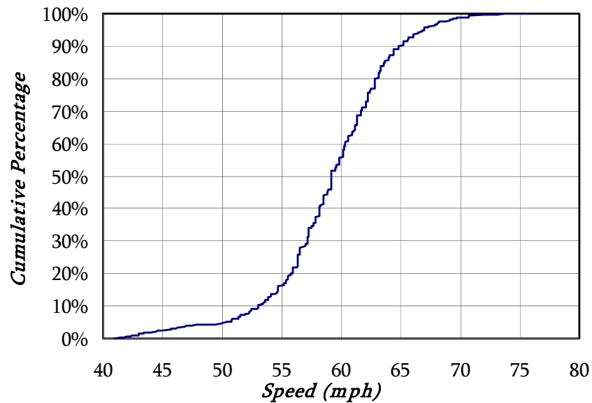
Figure 3-4 Histogram and Cumulative Distribution of the Sample Truck's Speed
