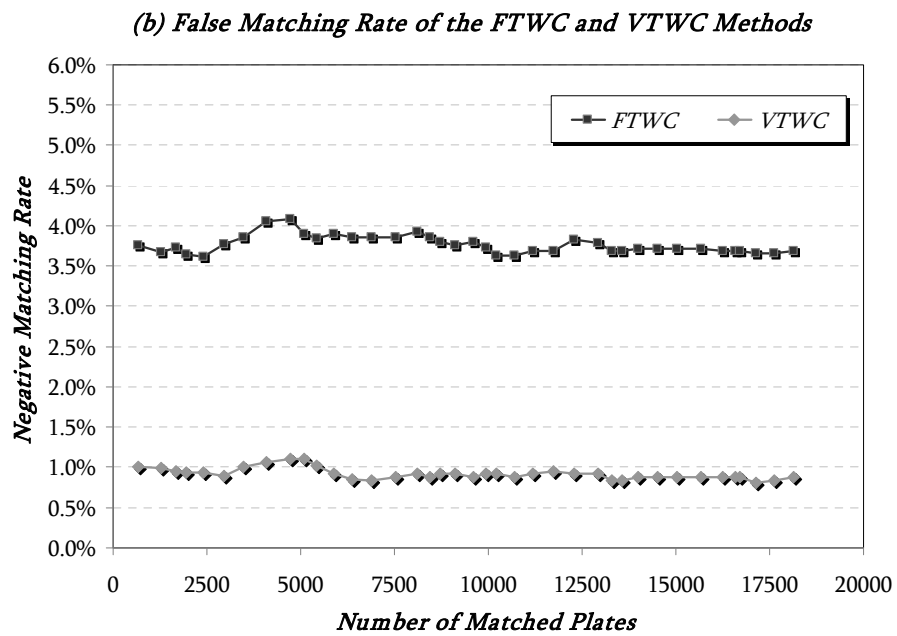
Figure 6-7 Performance of the Matching Procedures for Sequentially Estimates of C using LP Method
