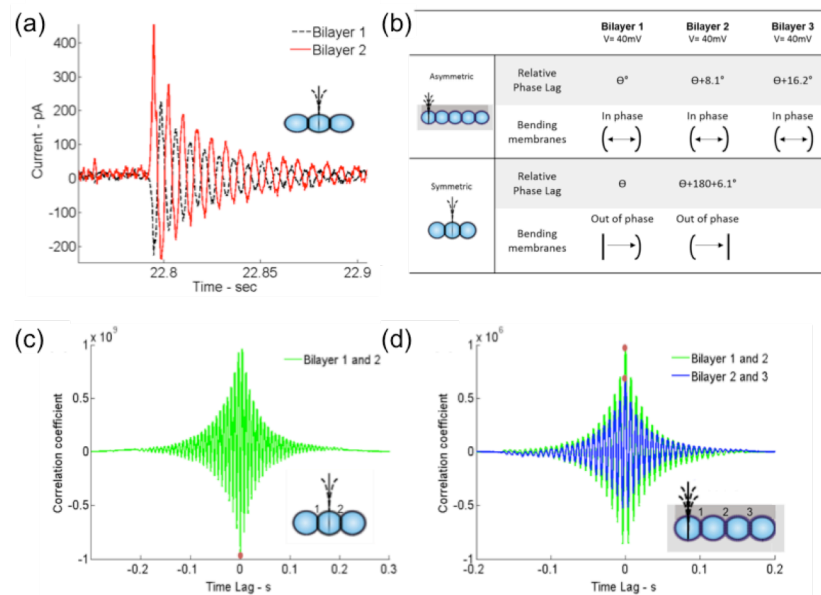
Figure 27: (a) Measured sensing currents of both bilayers in a three-droplet array in response to flicking a hair positioned in the middle droplet. (b) Table of phase analysis of sensing currents and membrane bending in asymmetric and symmetric serial array. (c) Phase correlation coefficient versus time lag of membrane currents for symmetric (c) and asymmetric (d) hair cell array configurations. The red circle in both plots marks the location of the largest amplitude coefficient.
