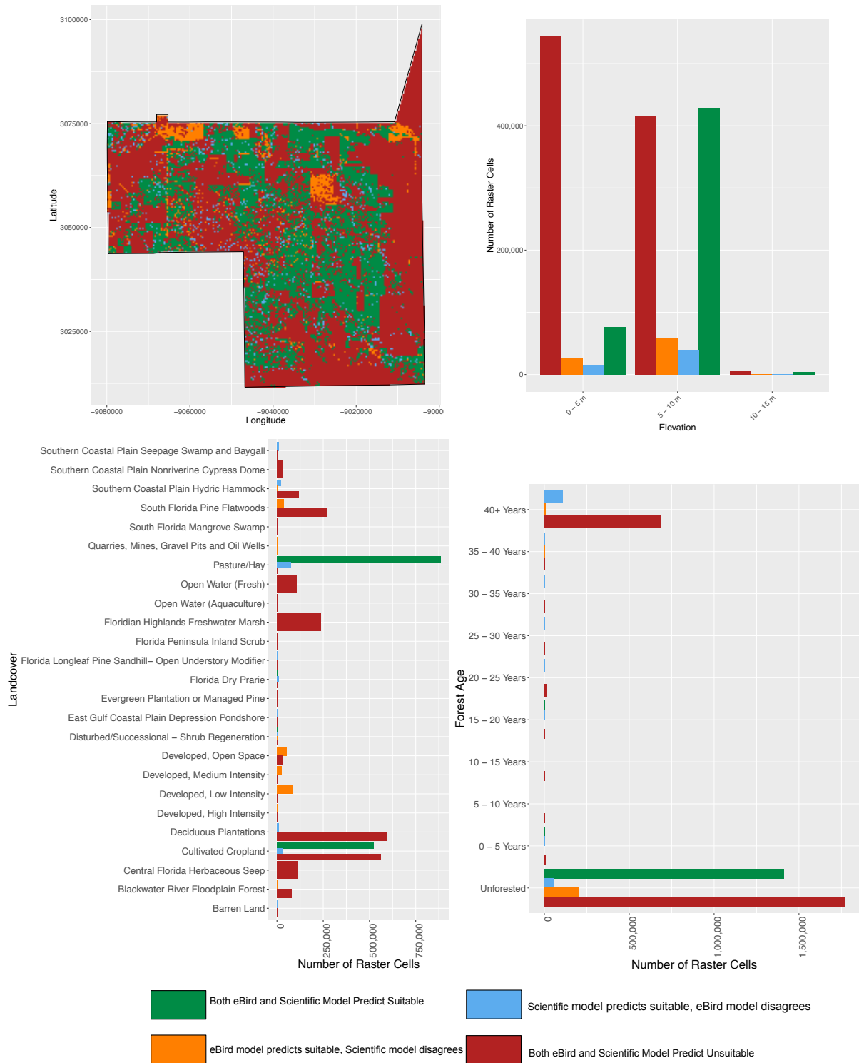
Figure 3.5 (cont.) Map of model agreement and distribution of environmental characteristics in Areas A, B, C, and D in Hendry county, where there was high concordance between the scientific and eBird model
