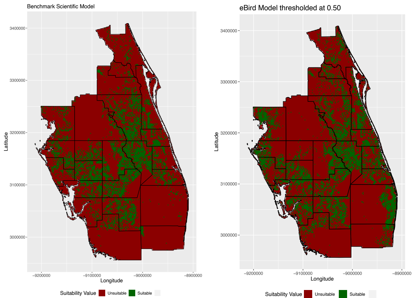
Figure 3.3 Binary suitability models developed with scientific data (left) and eBird data (right)
