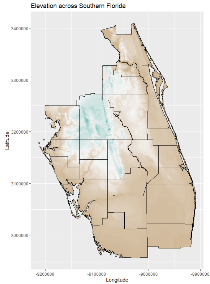
Figure 1.2 Two types of spatial data used as input variables for Species Distribution Models
