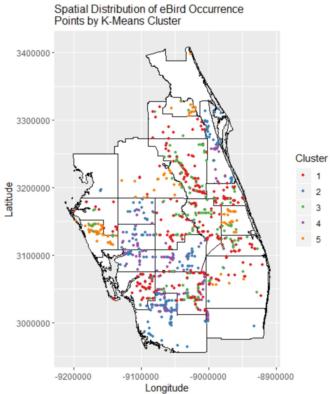
Figure 4.12 The spatial distribution of presence points from eBird classified by cluster
