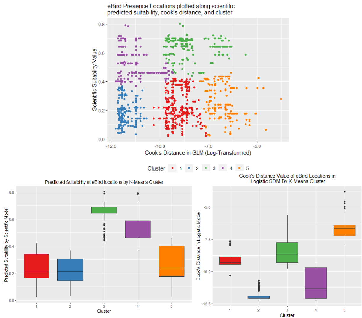
Figure 4.6 eBird points classified by clusters plotted with both explanatory variables: Scientific Suitability and Cook's Distance (top) showing the spread of values along scientific predicted suitability (bottom left) and showing the spread of values along Cook's distance (bottom right)
