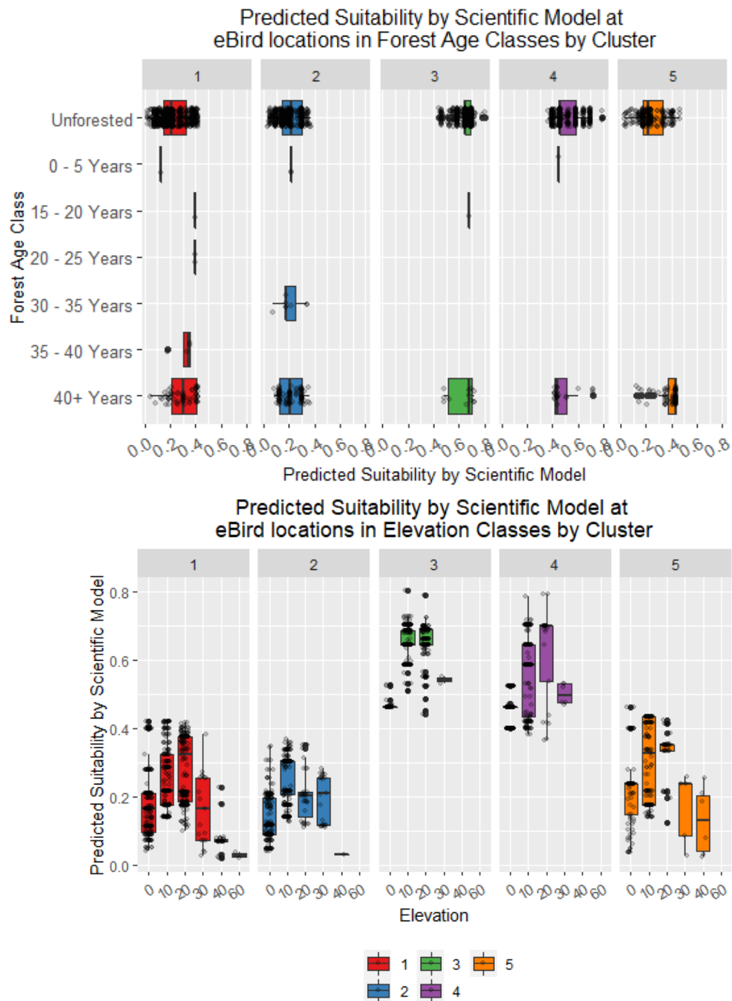
Figure 4.10 Predicted suitability by scientific model at eBird locations classified by cluster across elevation and forest age classes
