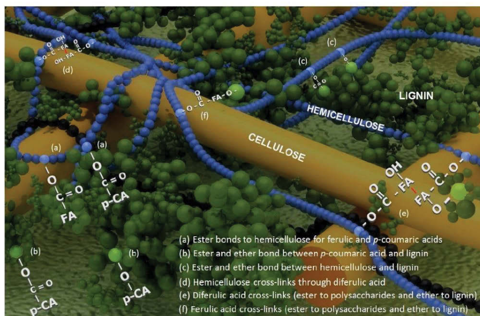
Figure 2. Structural representation of lignocellulosic biomass components. 5
