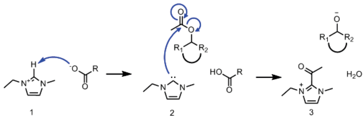
Figure 17. Mechanism for deacetylation of biomass using ionic liquids. R represents the H or \text{CH}_3 attached to the formate or acetate anion. \text{R}_1 and \text{R}_2 represent the carbon chain on the biomass structure.
