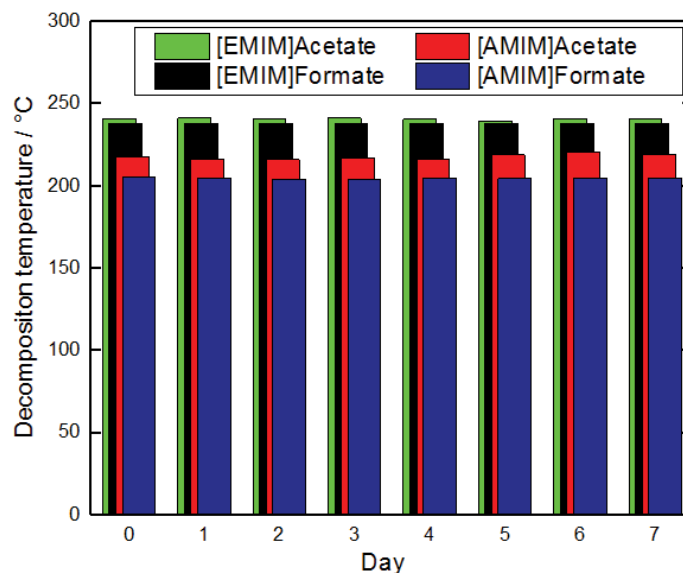
Figure 9. Thermal stability of ionic liquids over a 7-day period. Standard deviations were measured but not shown in the graph.
