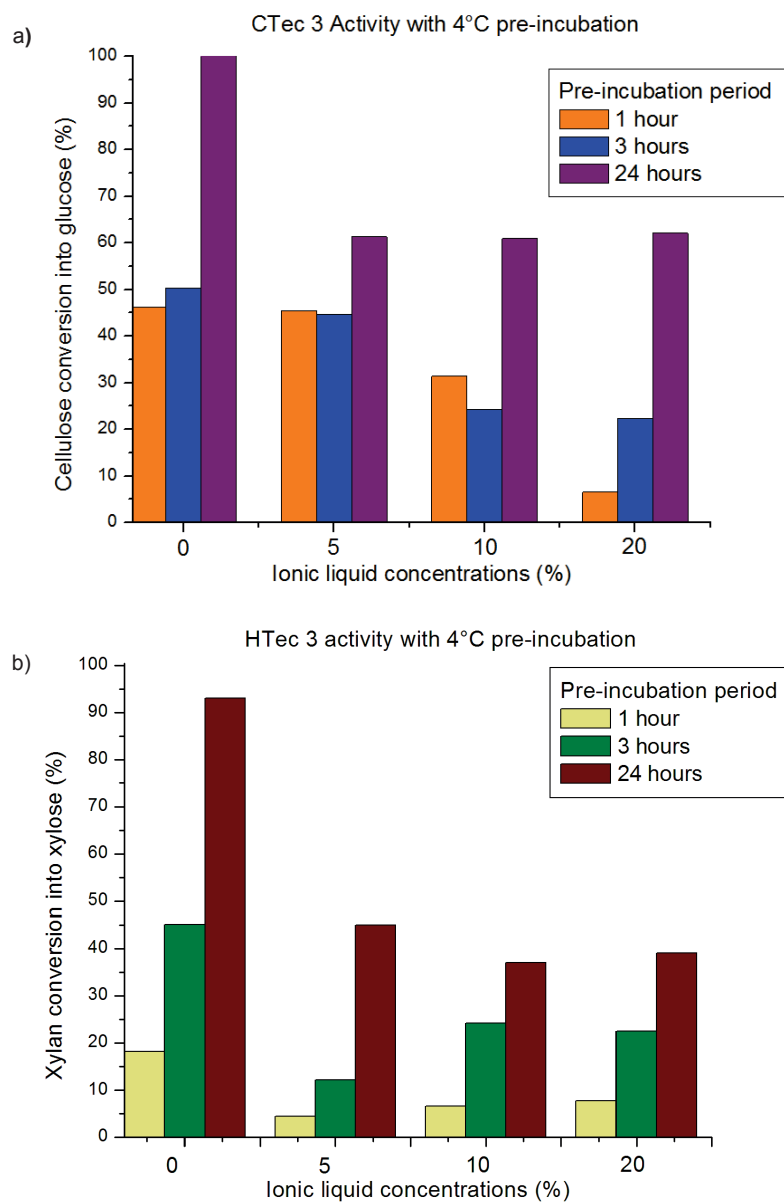
Figure 20. Activity of CTec 3 cellulases (a) and HTec 3 hemicellulases (b) in the presence of 0, 5, 10, and 20% IL.
