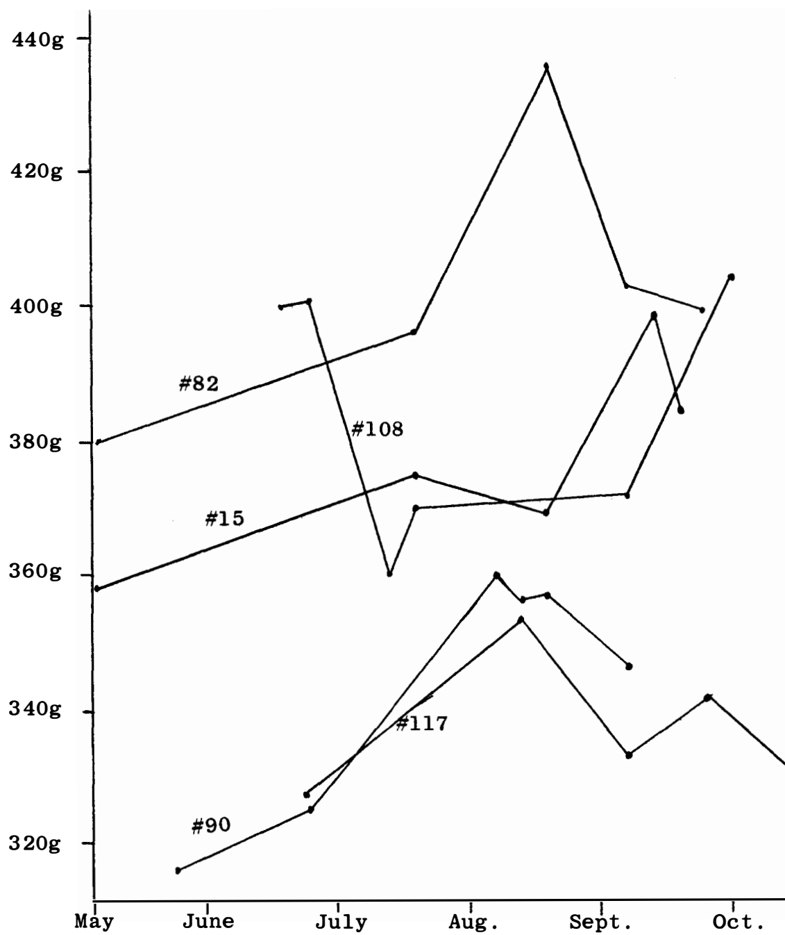
Figure 3. Weight fluctuations of female turtles during 1968.
