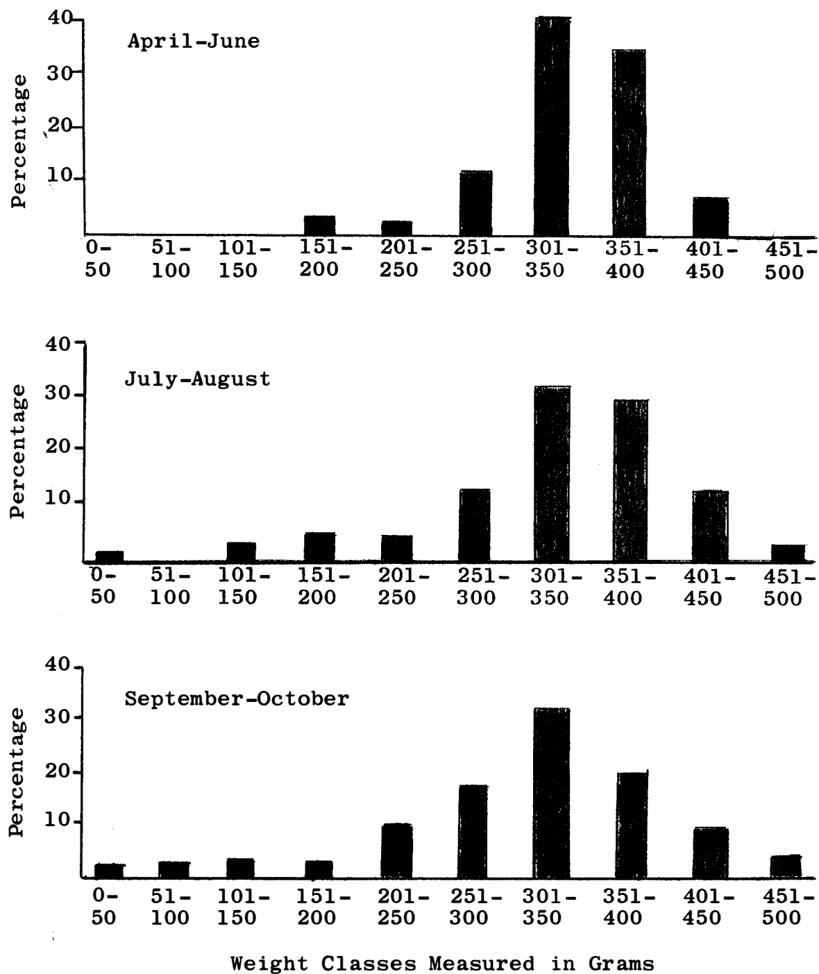
Figure 4. Percentage of turtles found in each weight class for different seasons.
