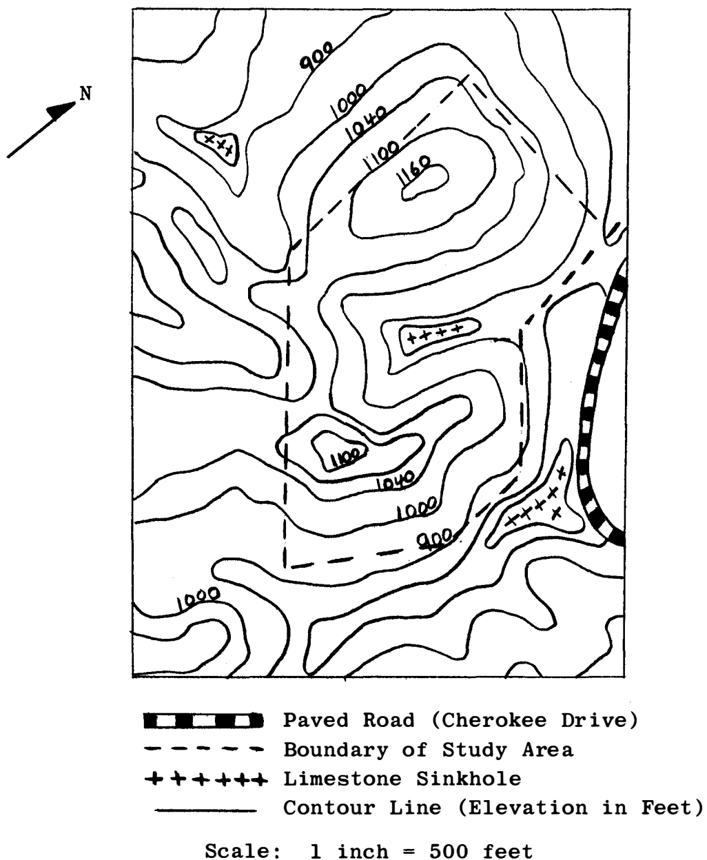
Figure 1. Map of study area on The University of Tennessee's Cherokee Farm.
