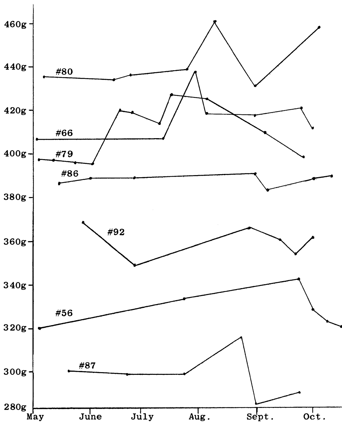
Figure 2. Weight fluctuations of male turtles during 1968.
