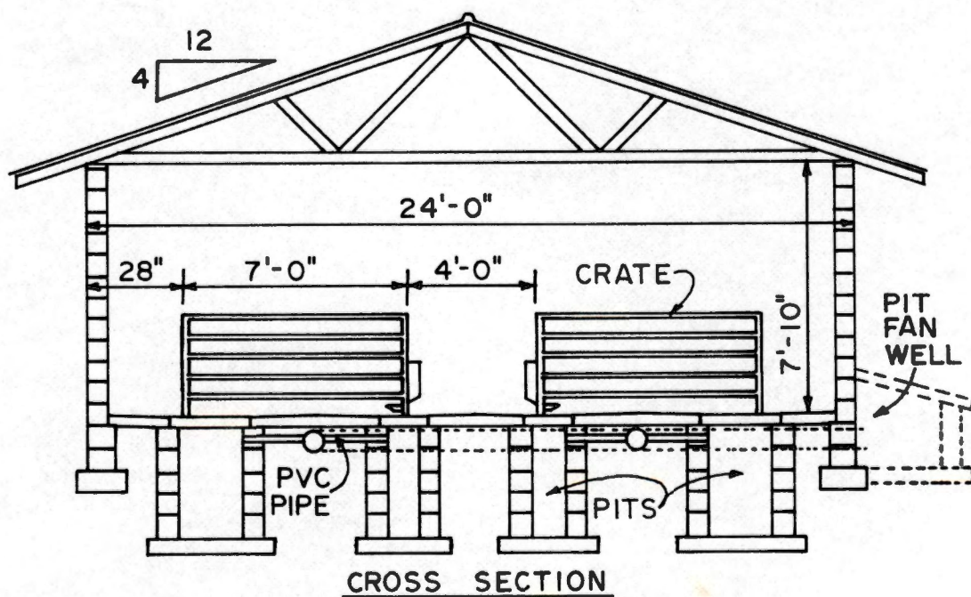
Figure 2. Farrowing House with PVC Pipe Pit Ventilation System.
