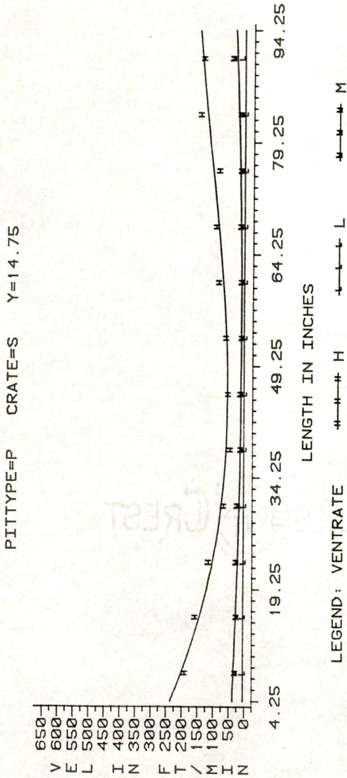
Figure D-1. Sow Nose Velocities for PVC Pipe Pit Ventilation, Solid Side Crates, and Y = 14.75 inches.
