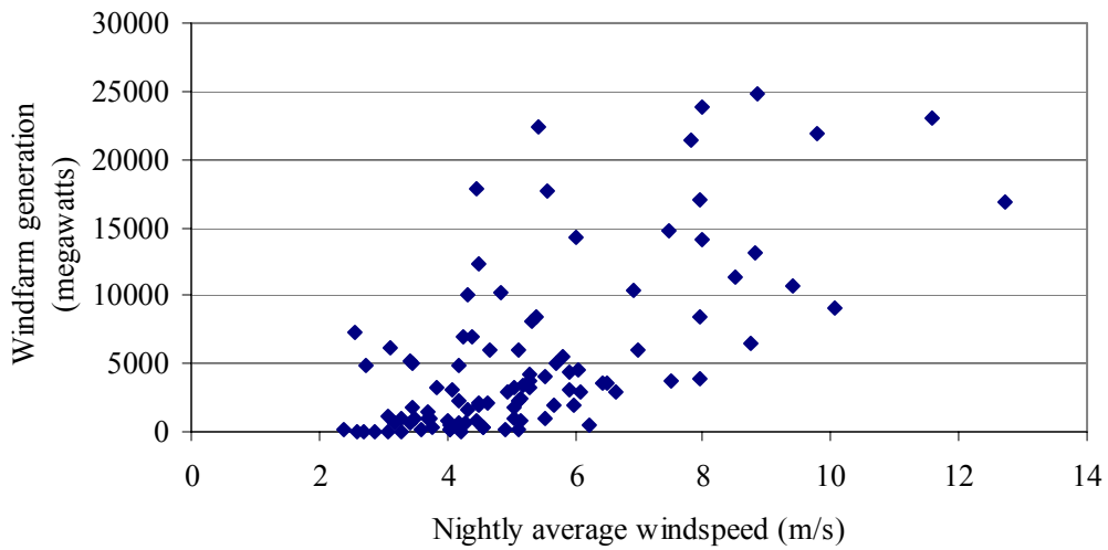
Figure 19. Relationship of nightly wind speed with windfarm generation at Buffalo Mountain Windfarm, eastern Tennessee, 16 July – 30 September 2002 & 2003.
