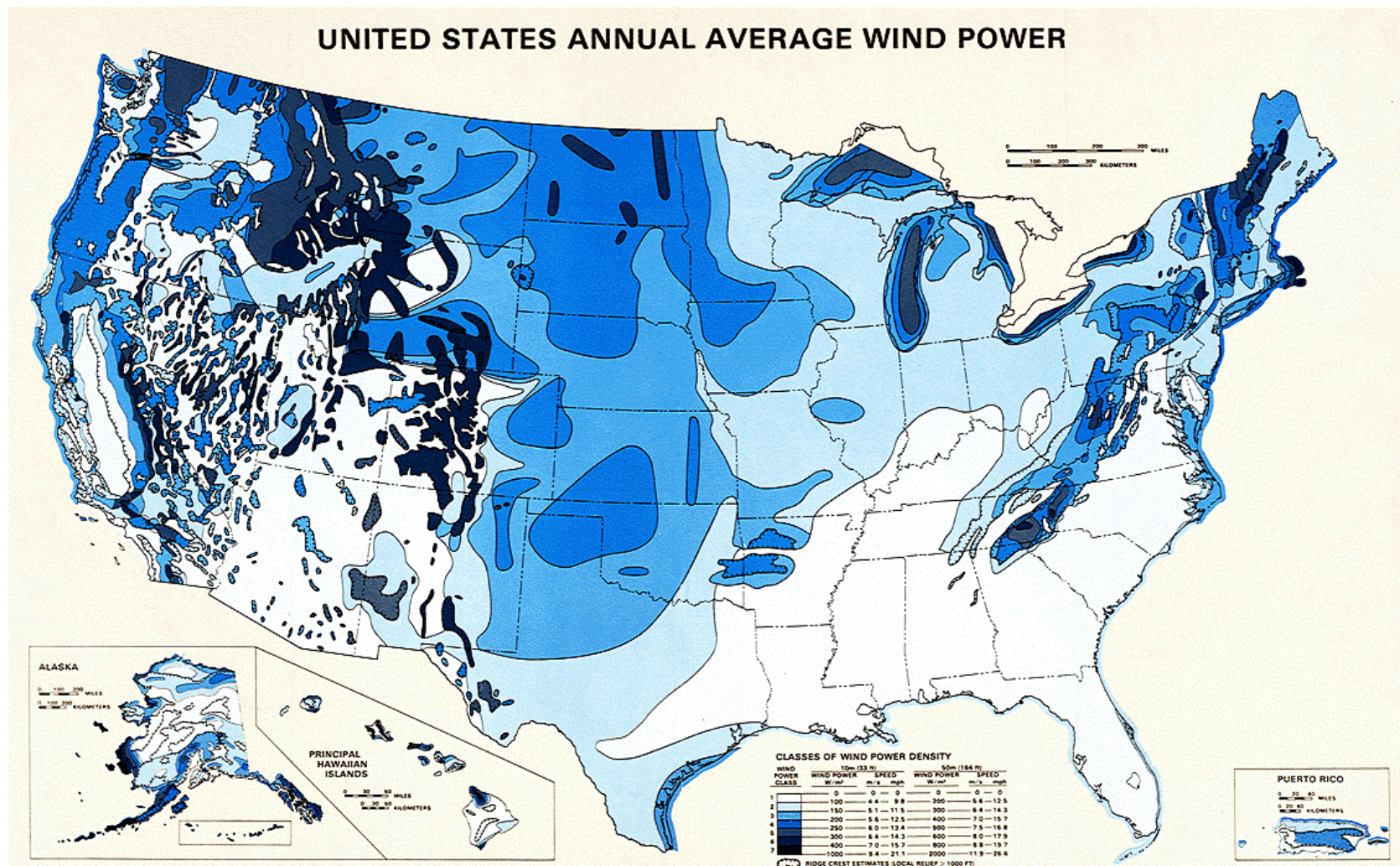
Figure 1. Distribution of annual average wind power as presented by Elliott et al. 1986 in the “Wind Energy Resource Atlas of the United States” a document prepared by Pacific Northwest Laboratory for the U.S. Department of Energy.
