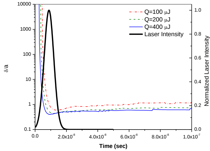
Figure 4. Ratio of skin layer thickness to plasma radius and normalized laser intensity profile versus time (seconds) of the simulated plasma for absorbed laser energies of 100, 200, & 400 \mu\text{J} . Microwave frequency f=12 \text{ GHz} .
