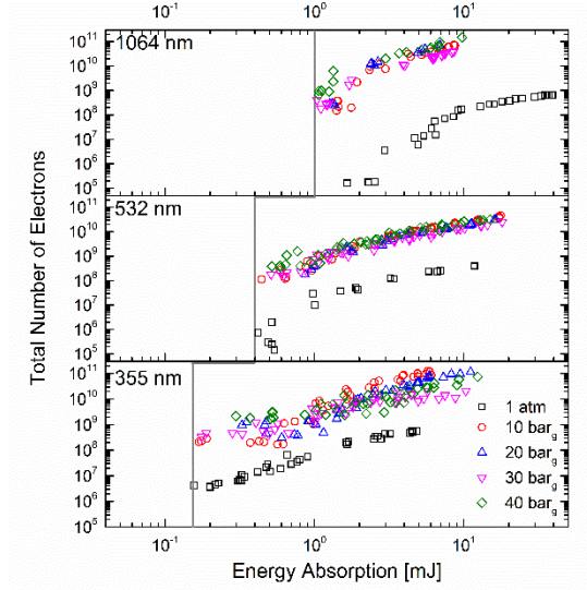
Figure 16. Total electron number versus laser energy absorption during laser induced breakdown in air at pressures ranging from atmospheric to 40 bar g with 1064 nm, 532 nm, and 355 nm wavelength beams.
