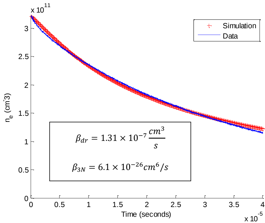
Figure 29. Comparison of experimental and fitted electron number density curves for the first 40 microseconds
