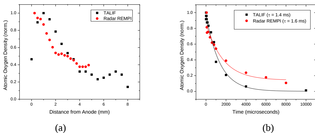
Figure 54. Comparison of TALIF and Radar REMPI measurements of atomic oxygen produced by a 4 kV pulsed discharge in a 1% O 2 /He mixture at 100 Torr. Normalized atomic oxygen density shown as (a) spatial profile and (b) temporal profile.
