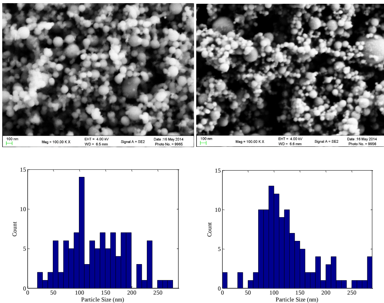
Figure 60. SEM images of (left) Al and (right) Fe nanoparticle samples, and (bottom) statistical analysis of the size distribution of the two samples
