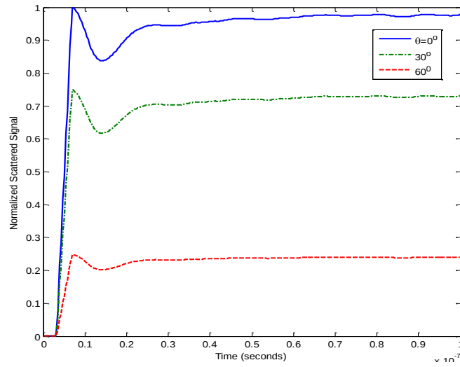
Figure 5. Normalized scattered signal versus time (seconds) from the simulated laser induced plasma for an absorbed laser power of 100 \mu J and microwave receiver horn angles of 0^\circ , 30^\circ , & 60^\circ .
