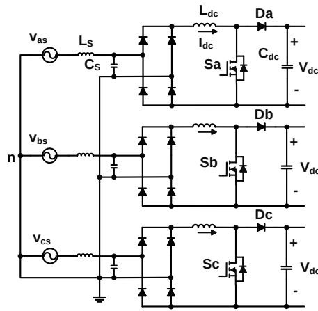
Fig. 1-8. Phase-modular boost rectifier for data center power supply.
