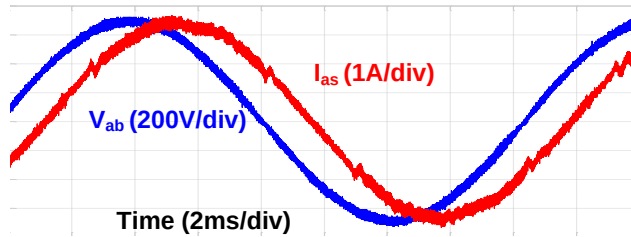
Fig. 7-29. Experiment results with traditional method (480 Vac, 5A Idc, 500 ns overlap time).
