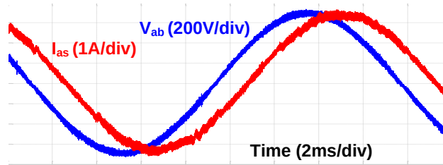
Fig. 7-30. Experiment results with proposed method (480 Vac, 5A Idc, 100 ns overlap time).
