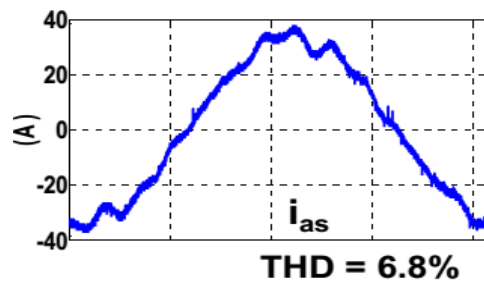
Fig. 10-3. Input current waveform of CSR with distortion [144].
