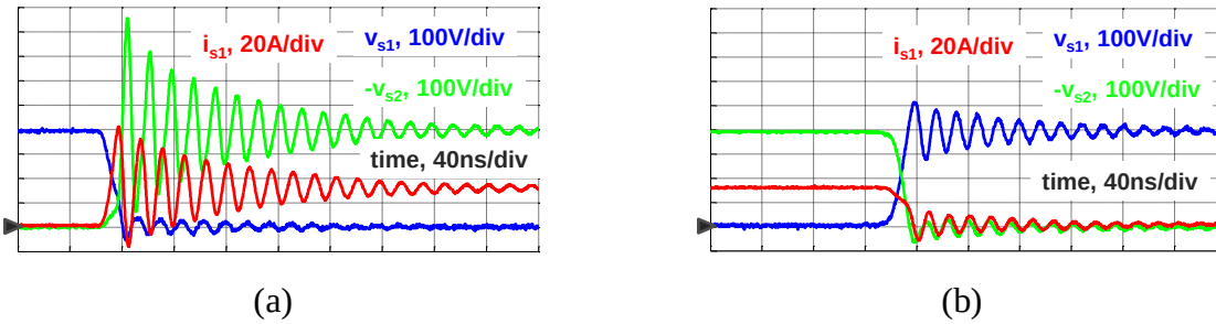
Fig. 5-26. Switching waveforms of CSR module when V_{xy} = 400 \text{ V} , I_{dc} = 34 \text{ A} and R_g = 5 \Omega : (a) S1 turn on; (b) S1 turn off.
