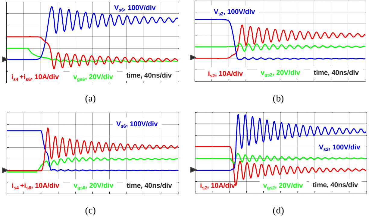
Fig. 3-22. Switching waveforms of new CSR when (a) S_6 and S_4 off (b) S_2 on (c) S_6 and S_4 on (d) S_2 off.
