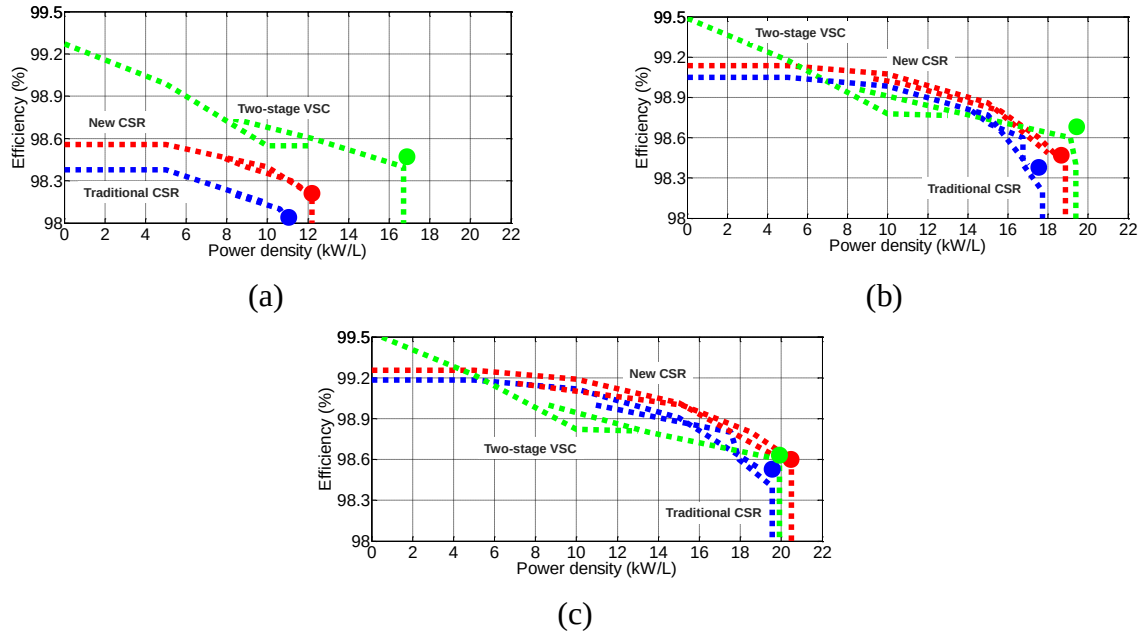
Fig. 4-36. Pareto front in efficiency-power density plane: (a) Die area = 1000 mm 2 ; (b) Die area = 2000 mm 2 ; (c) Die area = 2500 mm 2 .
