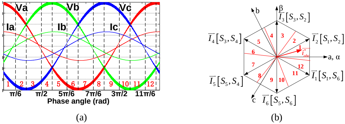
Fig. 8-1. Sector division in space vector PWM: (a) Input current and voltage; (b) Space vector plane.
