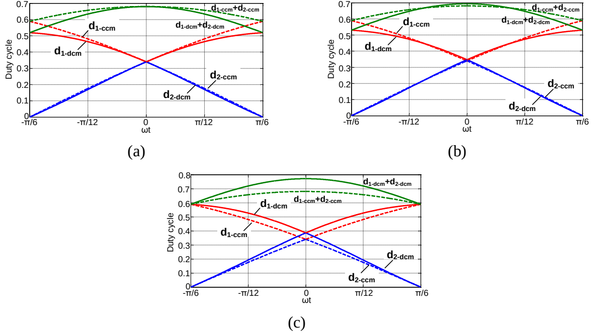
Fig. 8-17. Duty cycle comparison for SS-III in DCM and CCM: (a) P = 480 \text{ W} ; (b) P = 500 \text{ W} ; (c) P = 618 \text{ W} .
