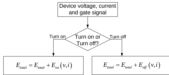
Fig. 5-11. Switching loss calculation process.
