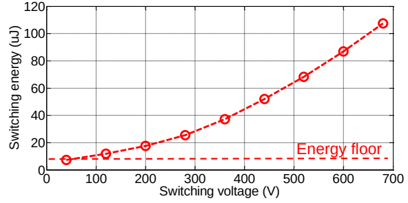
Fig. 5-10. Switching energy in CSR.
