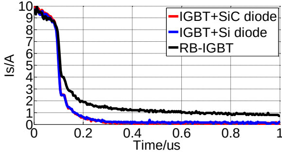
Fig. 6-6. "Tail current" comparison.
