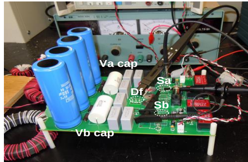
Fig. 6-3. Device double pulse test board.
