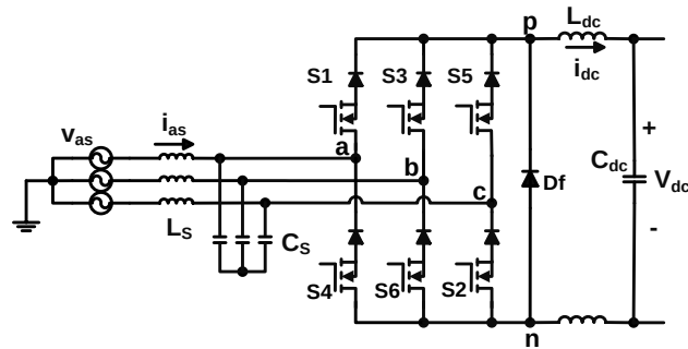
Fig. 1-10. Three-phase buck rectifier for data center power supply.
