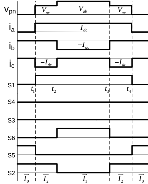
Fig. 3-11. Modulation scheme of traditional CSR in Sector 12.
