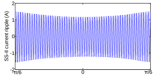
Fig. 8-6. Simulation result of current ripple with SS-II.
