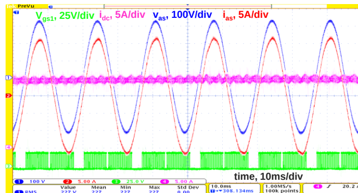
Fig. 3-34. Experimental waveforms under 400 V input voltage.
