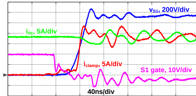
Fig. 9-16. Enlarged waveforms at t_1 in pulse test.
