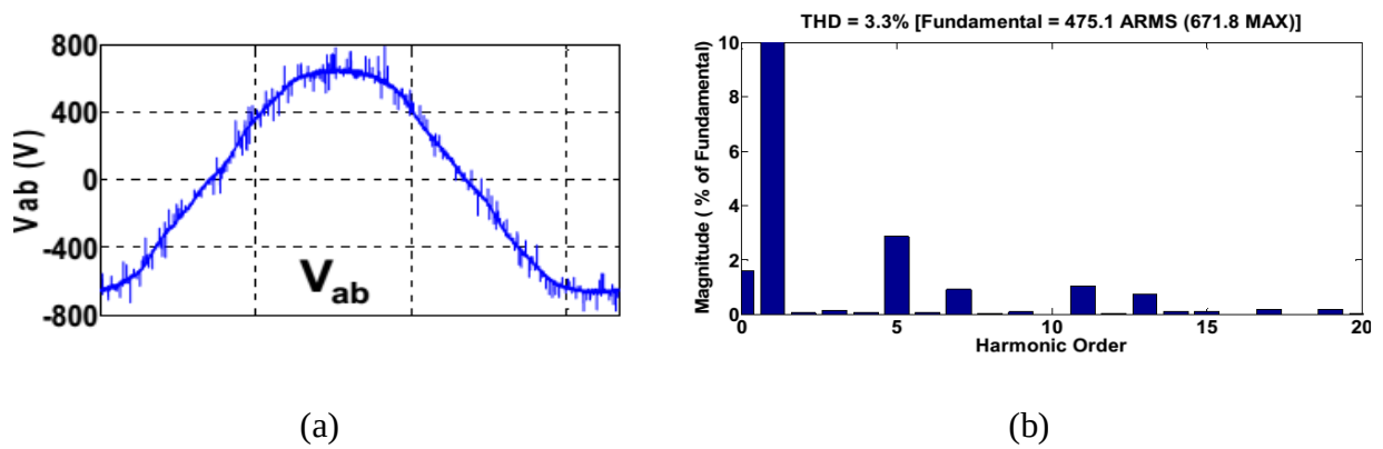
Fig. 10-2. Grid voltage with harmonics: (a) Voltage waveform; (b) Voltage Spectrum [144].
