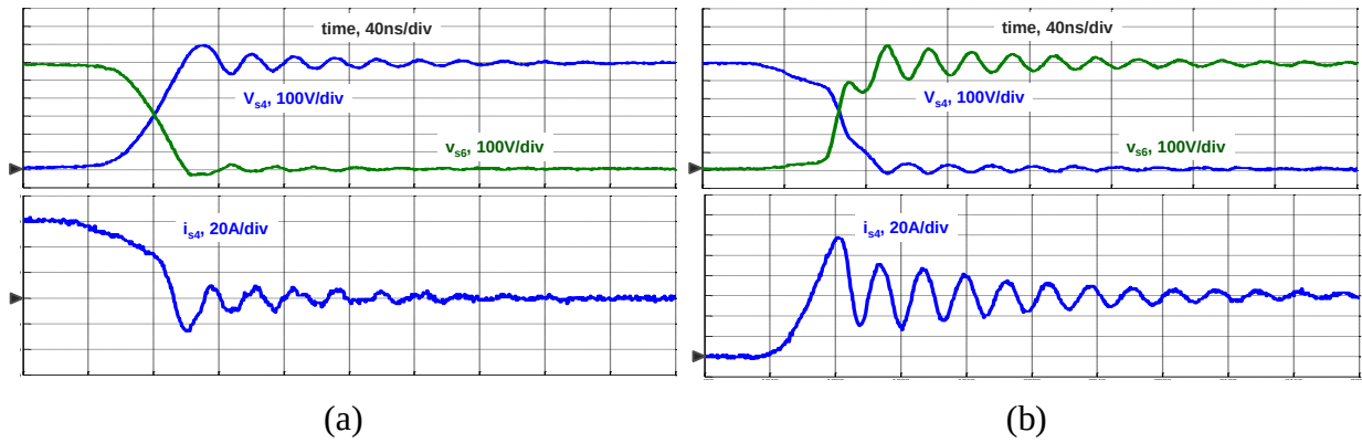
Fig. 5-50. Switching waveforms in Commutation loop 3: (a) Turn-off waveforms; (b) Turn-on waveforms.
