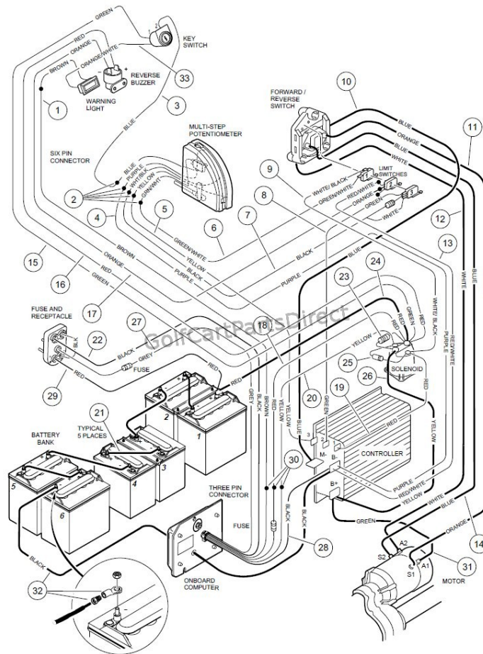
Figure 3: Golf Cart Wiring Diagram
