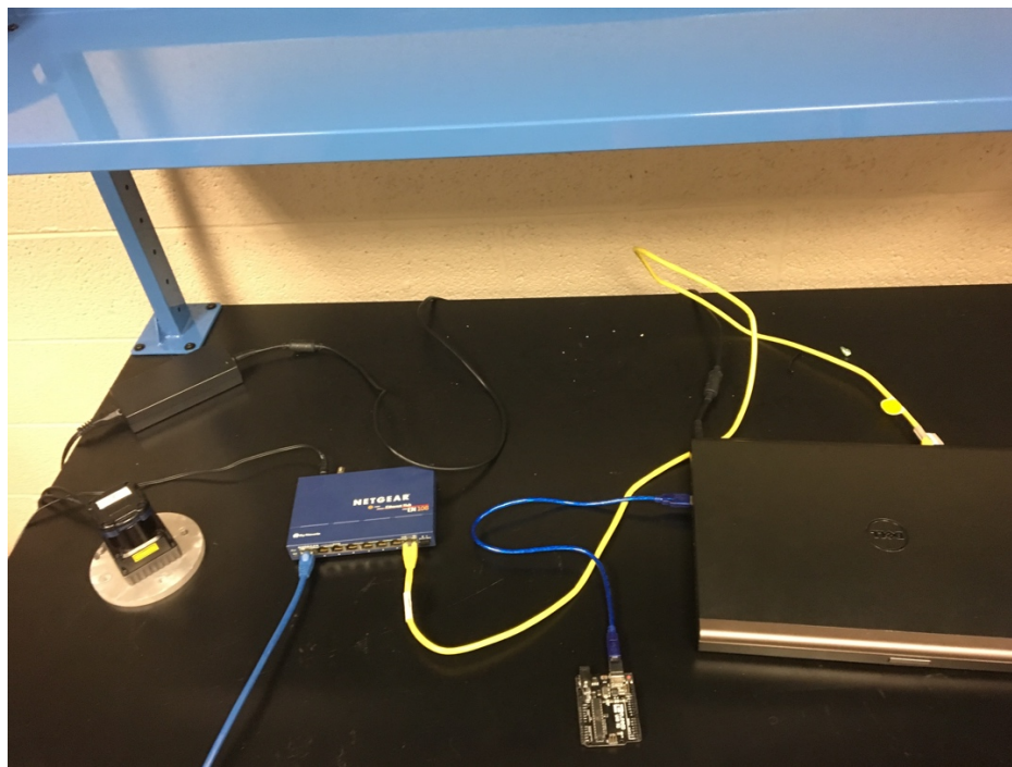
Figure 9: Testing Setup
