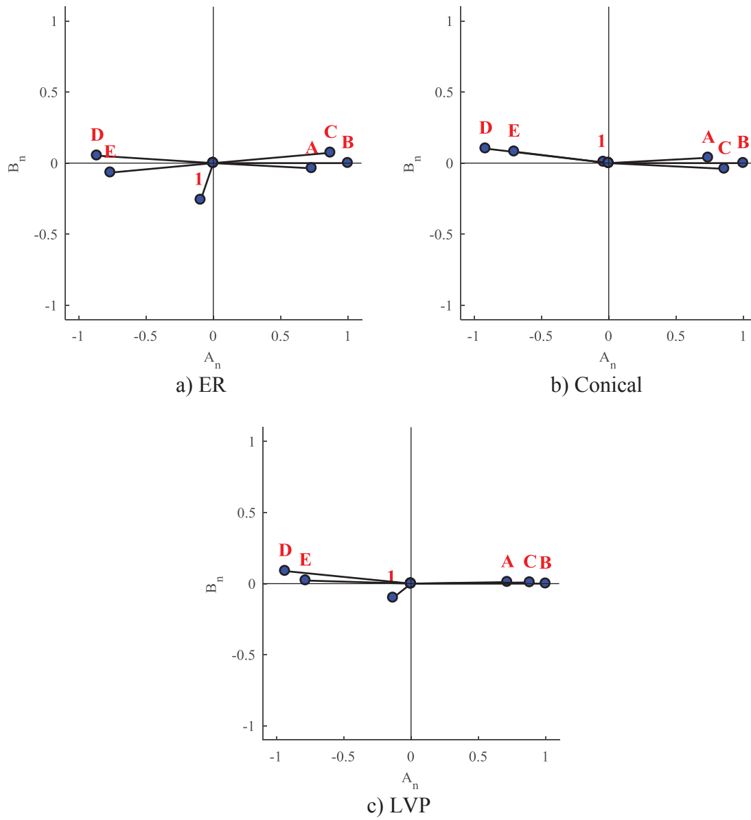
Figure 6.6. Phase Distribution for each Nozzle
