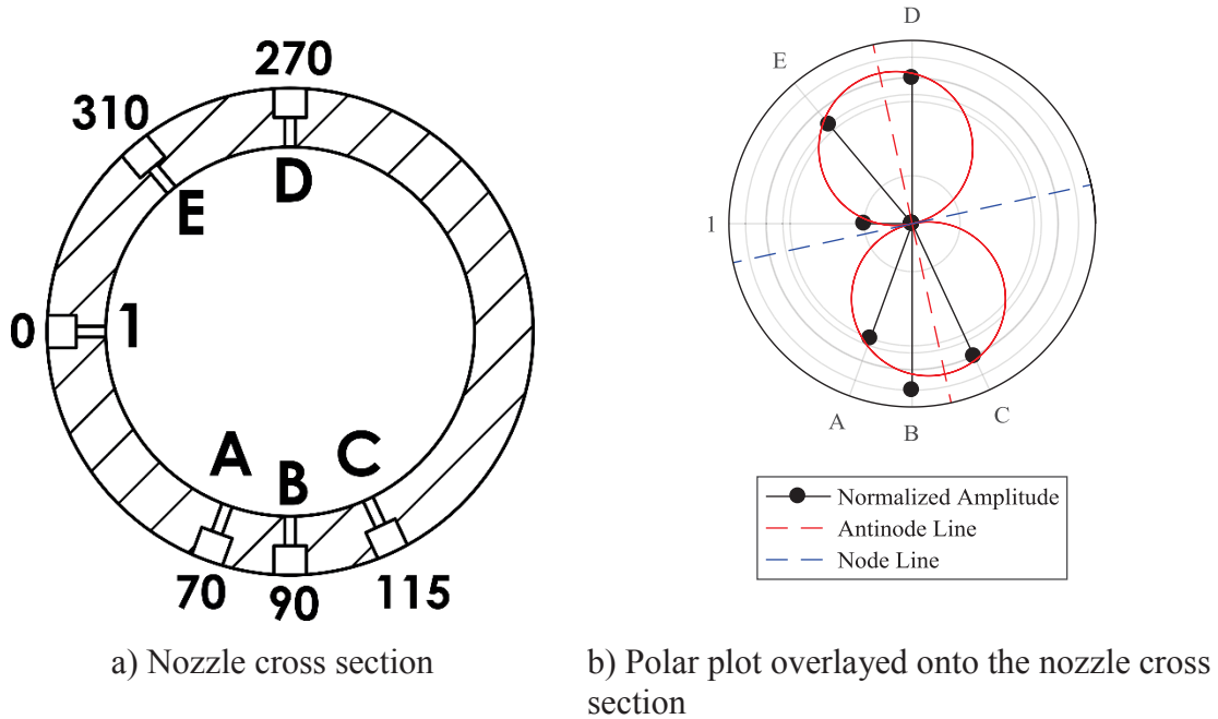
Figure 5.5. Mode Shape Plot from the ER Nozzle with Cross Sectional Reference
