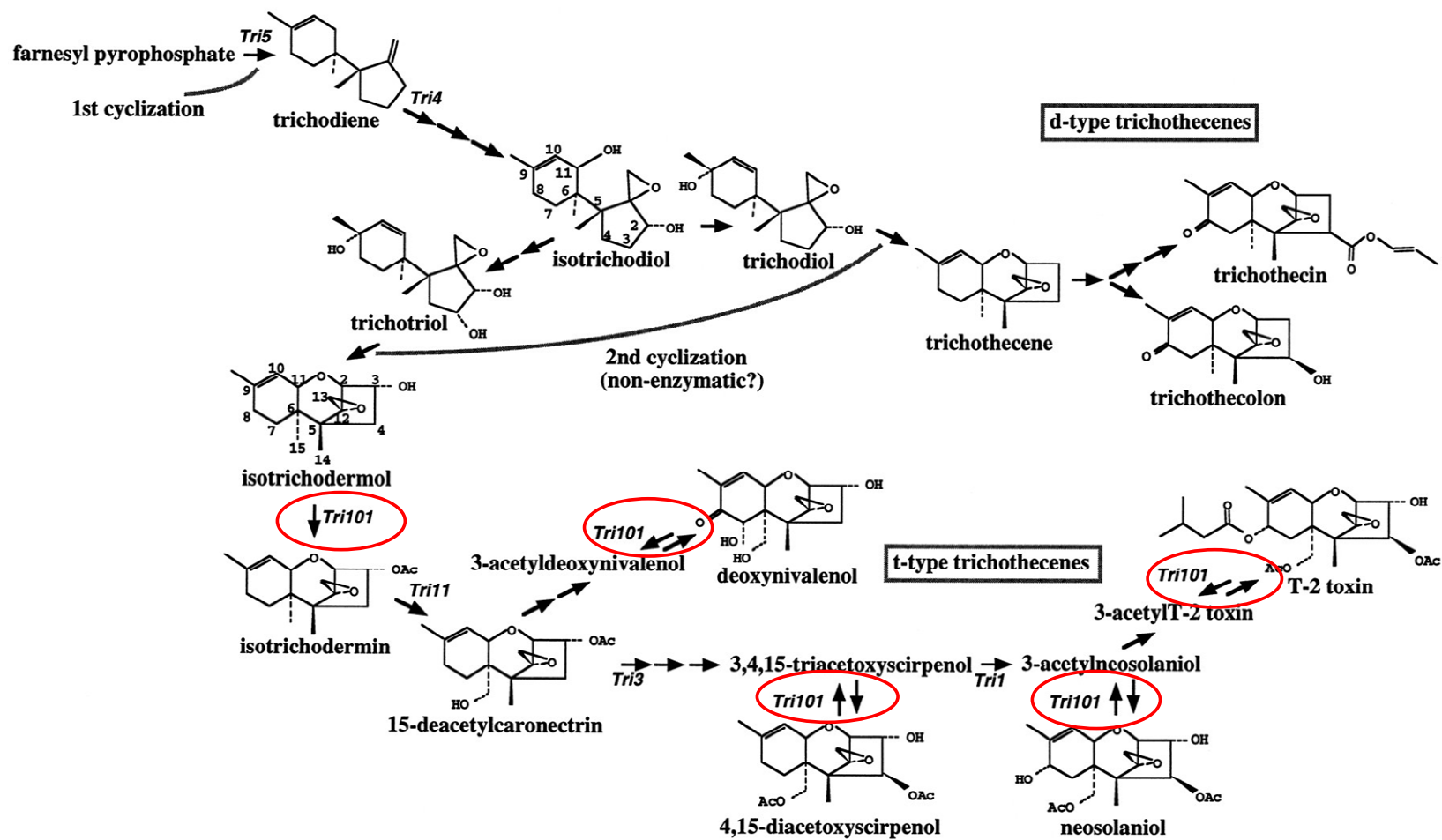
Figure 1.2 Trichothecene biosynthesis (Kimura et al. , 1998)
