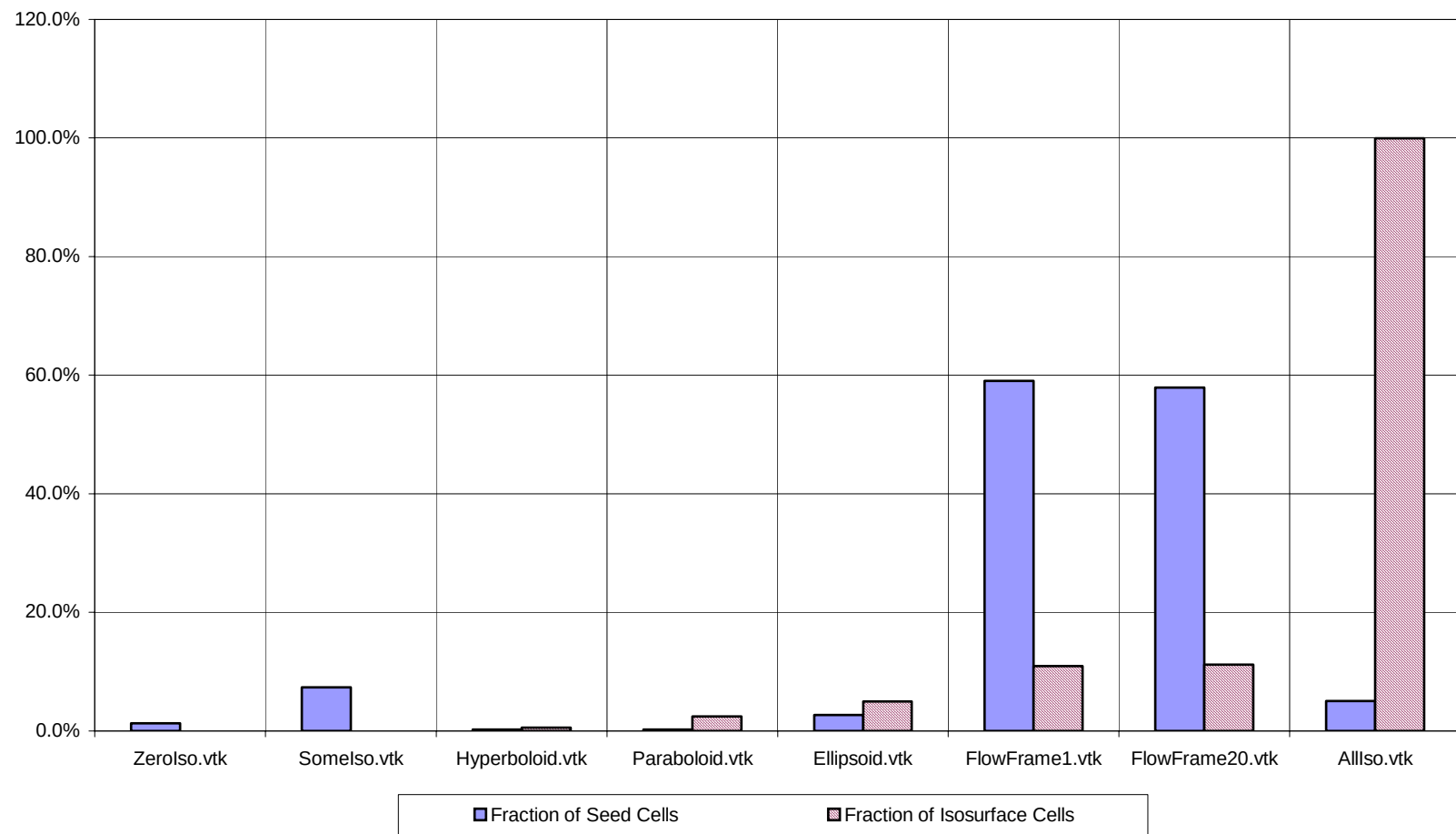
Figure 4.2: Dataset Characteristics
