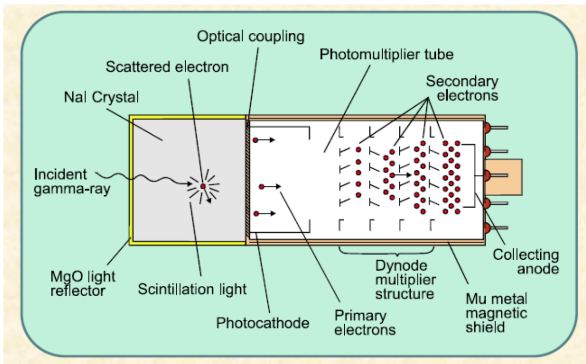
Figure 8: A typical scintillation crystal and a photomultiplier coupled together to make a complete detection element.
