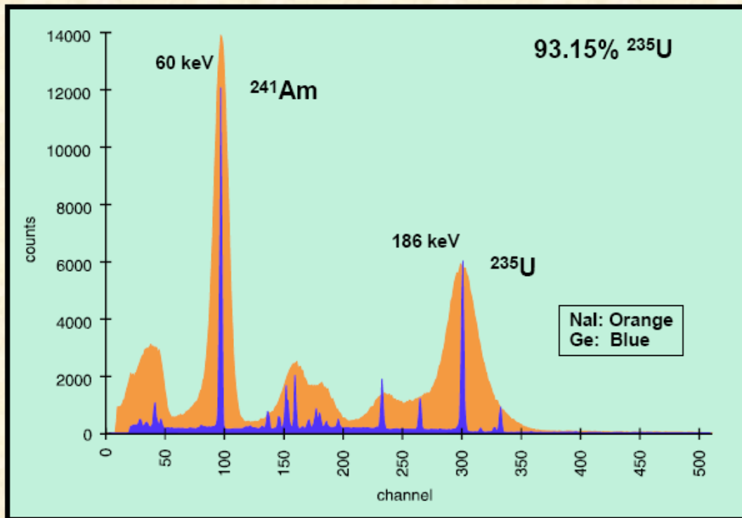
Figure 5: U-235 and Am-241 spectra at high and low resolution.
